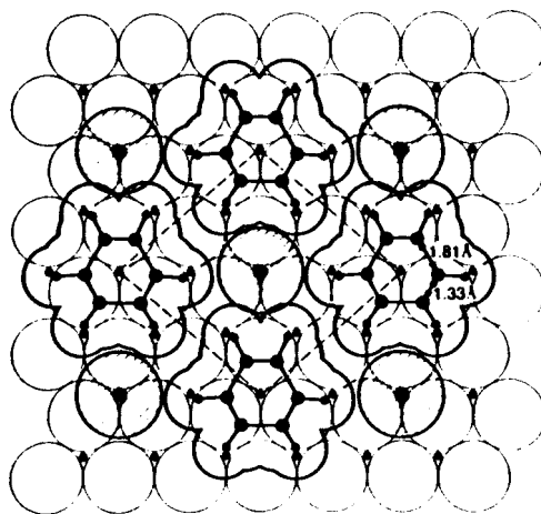
Rh(111) - (31/13) - C 6 H 6 + CO
