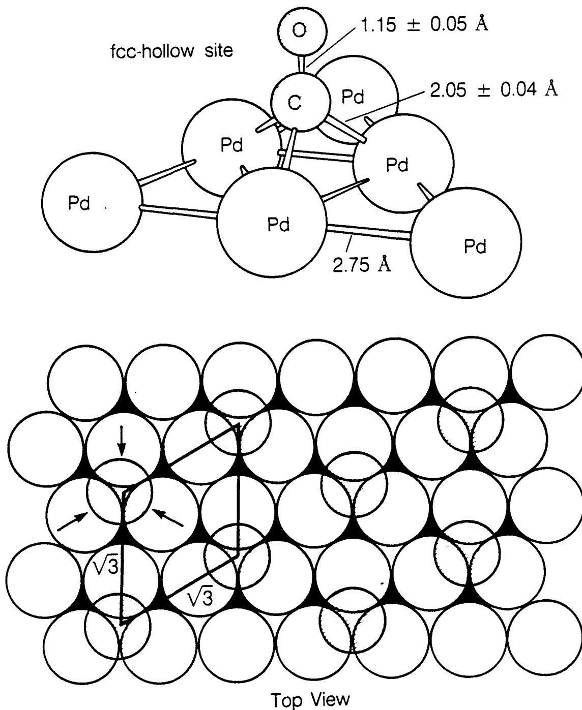
[Fig. 5-7] The optimum structure for CO in the ( \sqrt{3} \times \sqrt{3} )R30° arrangement on the Pd(111) surface, as determined by dynamical LEED and R-factor analysis. The arrows in the top view indicate the lateral displacements of the Pd atoms which have been considered in the structure determination (see Table 5-1.F). The analysis showed, however, no indication of such displacement.
