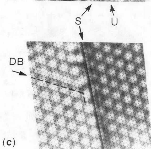
[Fig. 7-5] Three images of the (3x3) superlattice extending across an atomic step. ( V_t = -1.25\text{ V} , i_t = 4\text{ nA} ). (a),(b) Images derived from the same data, (c) image recorded \sim 10\text{ min} later.
