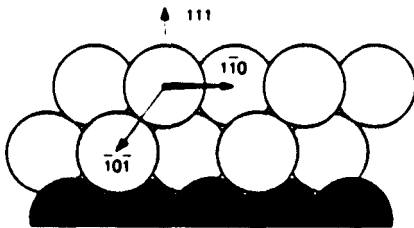
bcc (110)
