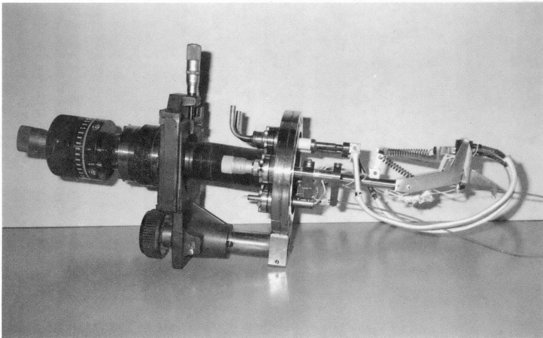
[Fig. 3-6] Photograph of high-precision manipulator for LEED and HREELS
