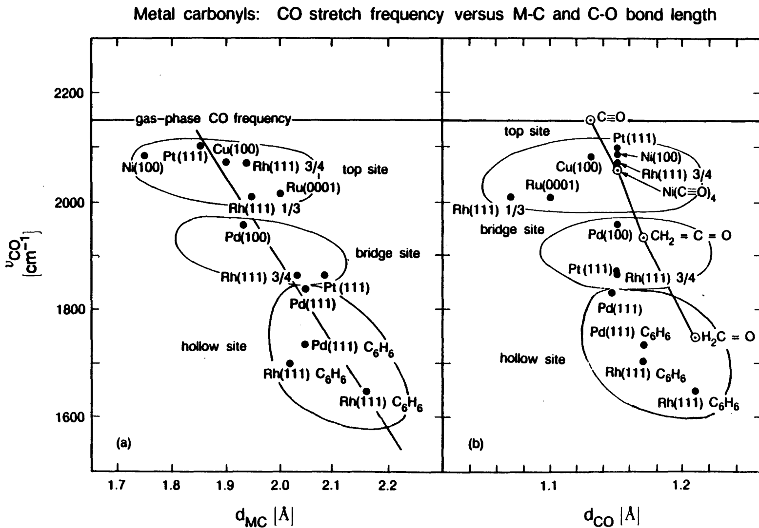
[Fig. 6-14] The correlation between the geometries of chemisorbed CO determined by LEED and CO stretching frequency observed by IR or HREELS.
