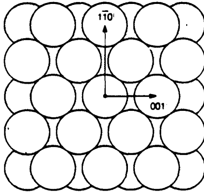
bcc (110)
