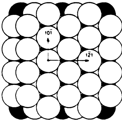
fcc (111)
