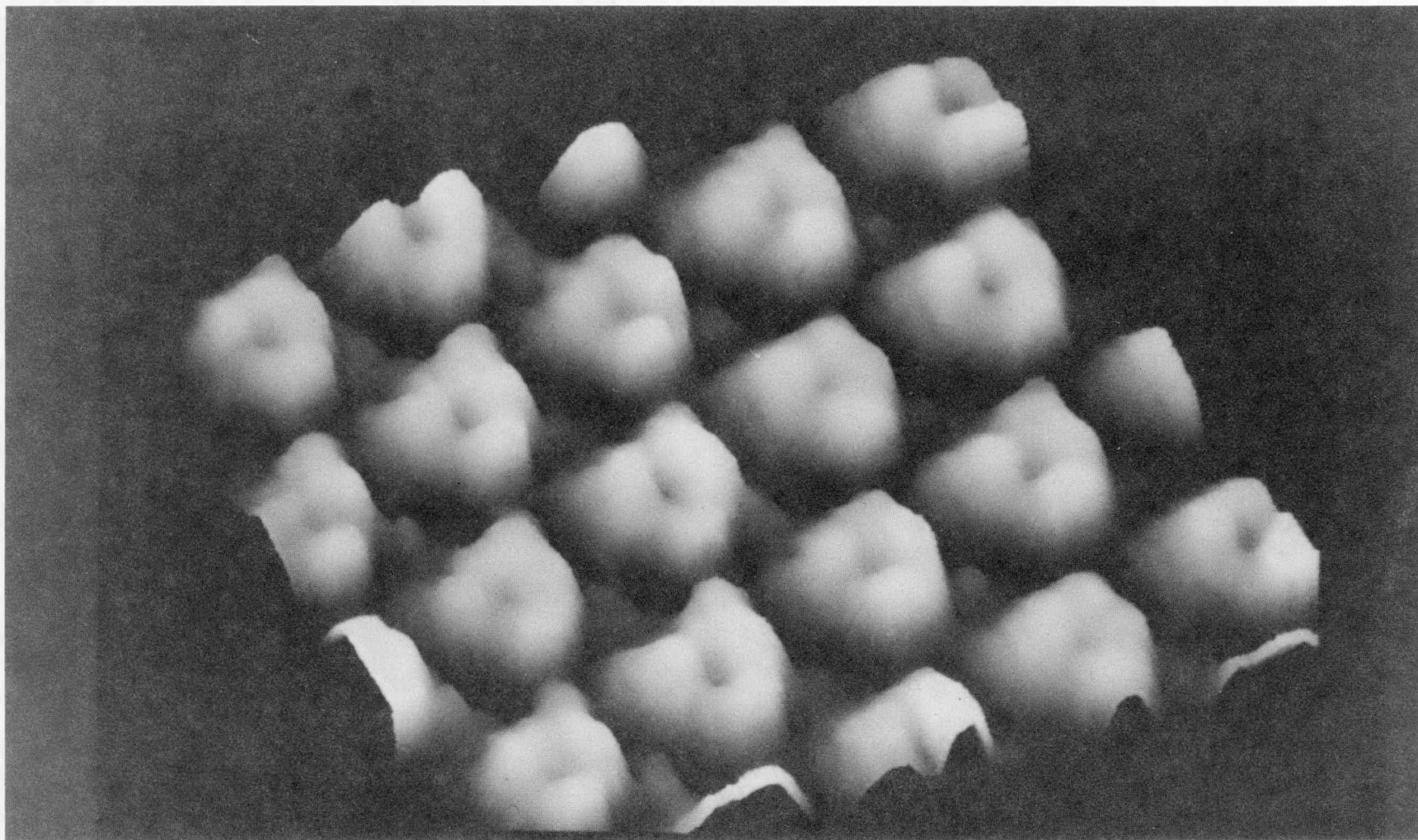
[Fig. 7-7] A three-dimensional view of the STM image ( V_t = -0.01\text{ V} , i_t = 2\text{ nA} )
