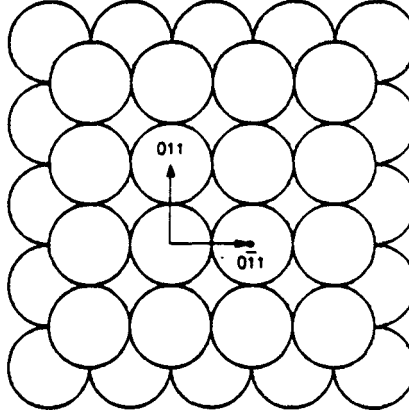
fcc (100)
