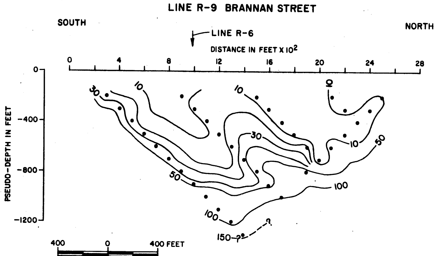
RESISTIVITY PSEUDO SECTION CALISTOGA AREA CONTOUR INTERVAL - 10 OHM FEET - 50 OHM FEET
