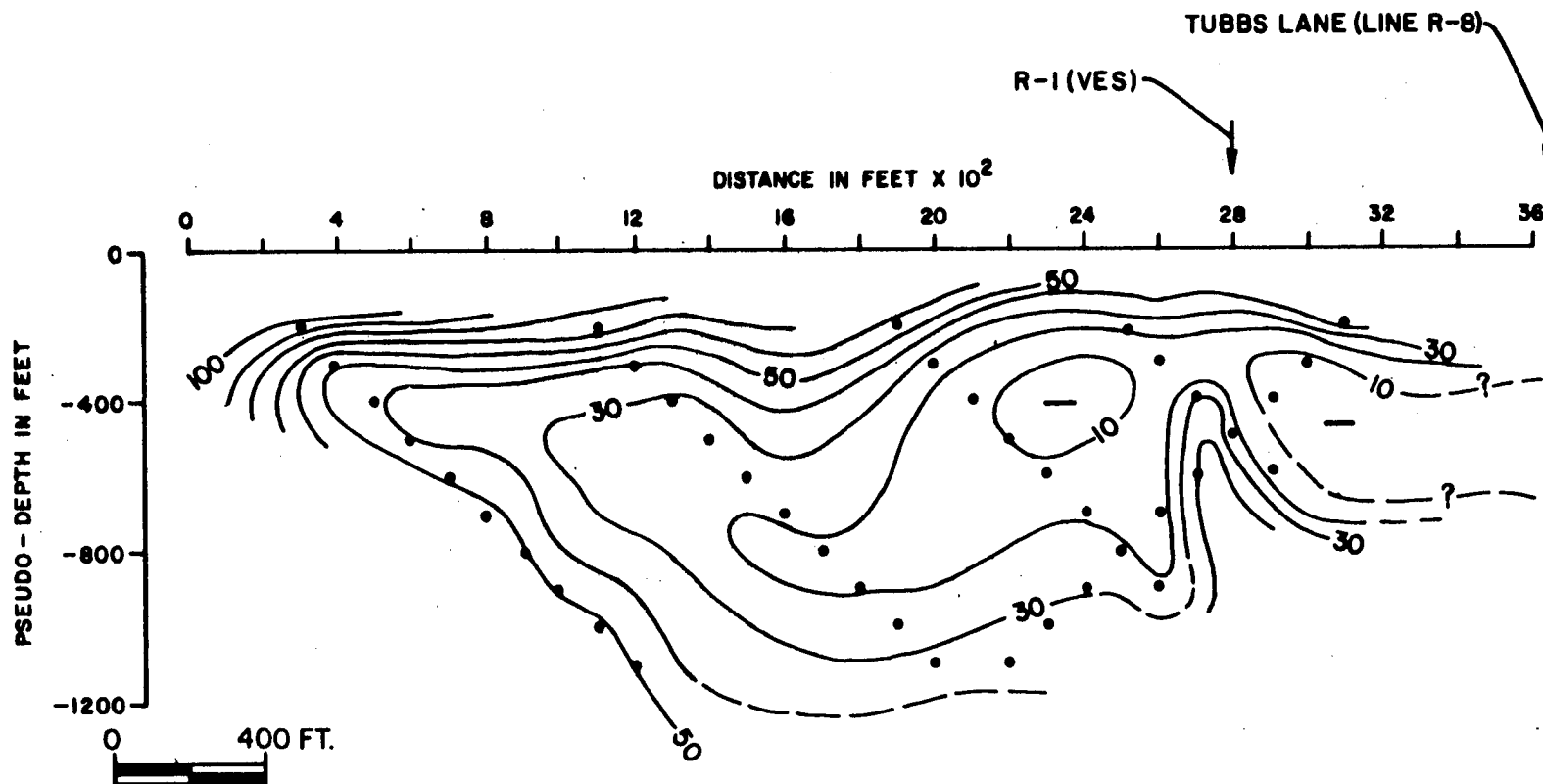
RESISTIVITY PSEUDO SECTION CALISTOGA AREA CONTOUR INTERVAL - 10 OHM FEET
