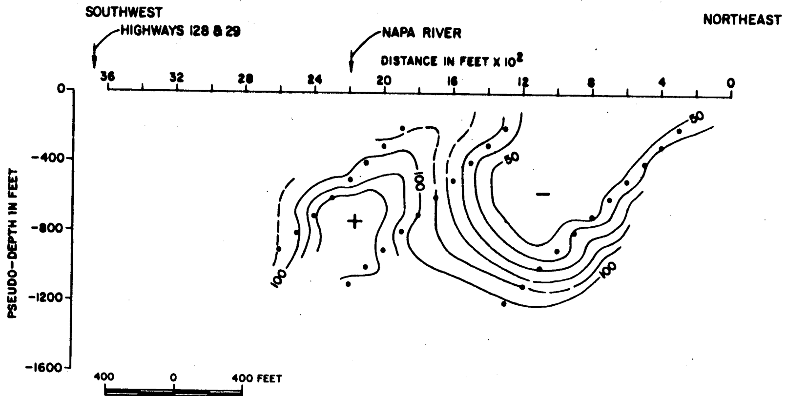
RESISTIVITY PSEUDO SECTION CALISTOGA AREA CONTOUR INTERVAL - 10 OHM FEET BY G. W. CHASE
