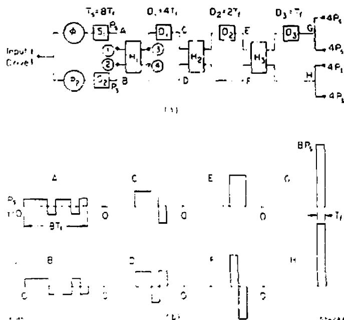
Fig. 7. (a) Diagram illustrating the pulse compression method of Z. D. Farkas; 28 (b) amplitude and relative phase of the RF power at the indicated points.
