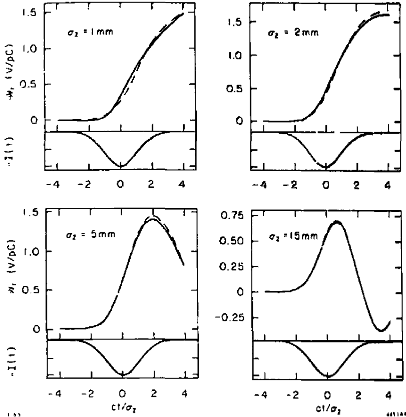
Fig. 15. Transverse wake potential ( m = 1 ) per cell for Gaussian bunches in the SLAC structure. Solid curves give TBC1 results and dashed curves are results from a sum of modes.
