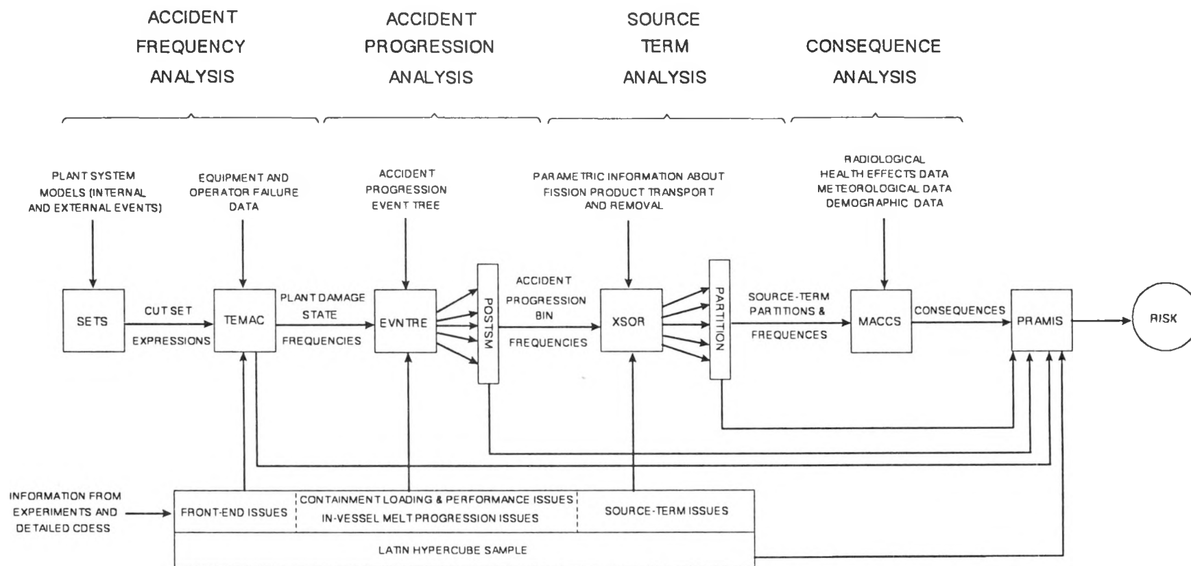
Figure 1.2. Overview of Integrated Plant Analysis in NUREG-1150
