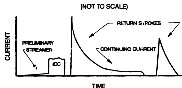
Figure 1. Typical Rocket-Triggered Lightning (RTL) Flash Current
