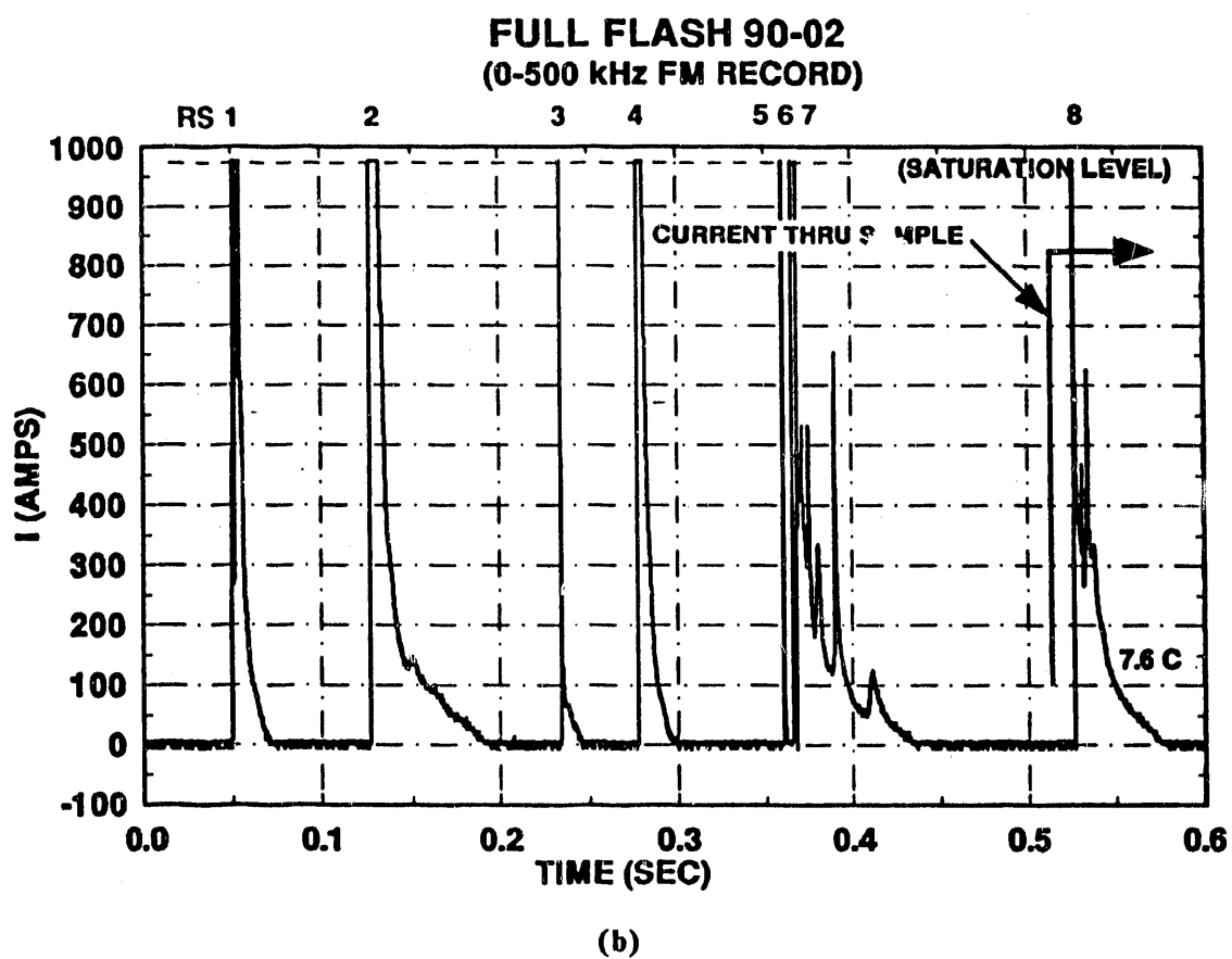
Figure 5. a) 80-mil Thick Al Specimen Exposed on Flash 90-02, and b) Current Recorded on Same Flash
