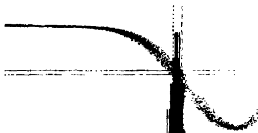
Fig. 5. Accelerator Gap leading edge of Fig. 3, expanded for time jitter measurement. Scope settings: 50 ps/div and 10 MV/div. Timing jitter sigma = 8.7 ps.
