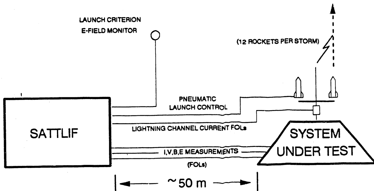
Figure 1. Munitions Storage Bunker Triggered Lightning Test Configuration
