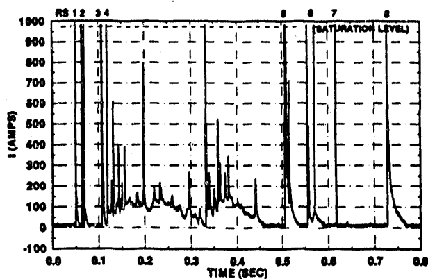
Figure 9. Flash 90-04 as Recorded by the SATT LIF Continuing Current Instrumentation
