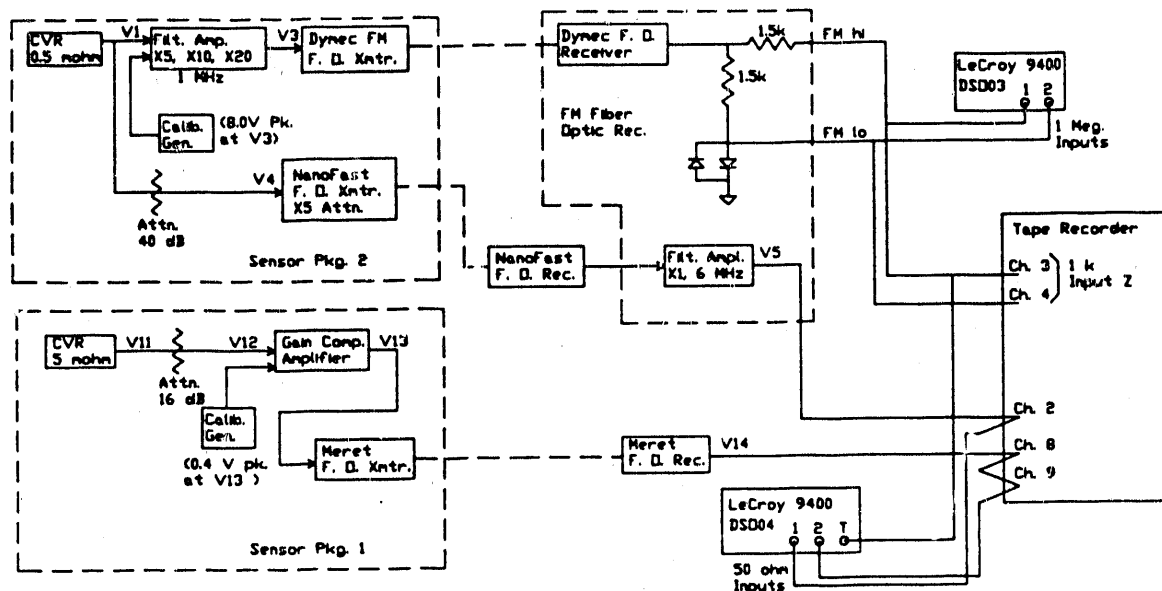
Figure 6. SATTILF Data Acquisition Instrumentation
