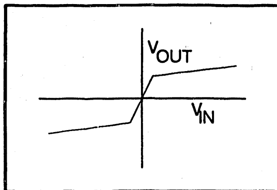
Figure 11. "Gain Compression" Amplifier Response Function
