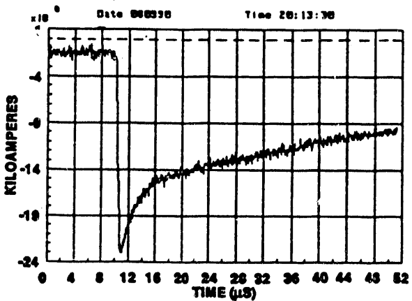
Figure 7. Stroke Currents of Flash 90-07 as Measured by KSC and SNL
