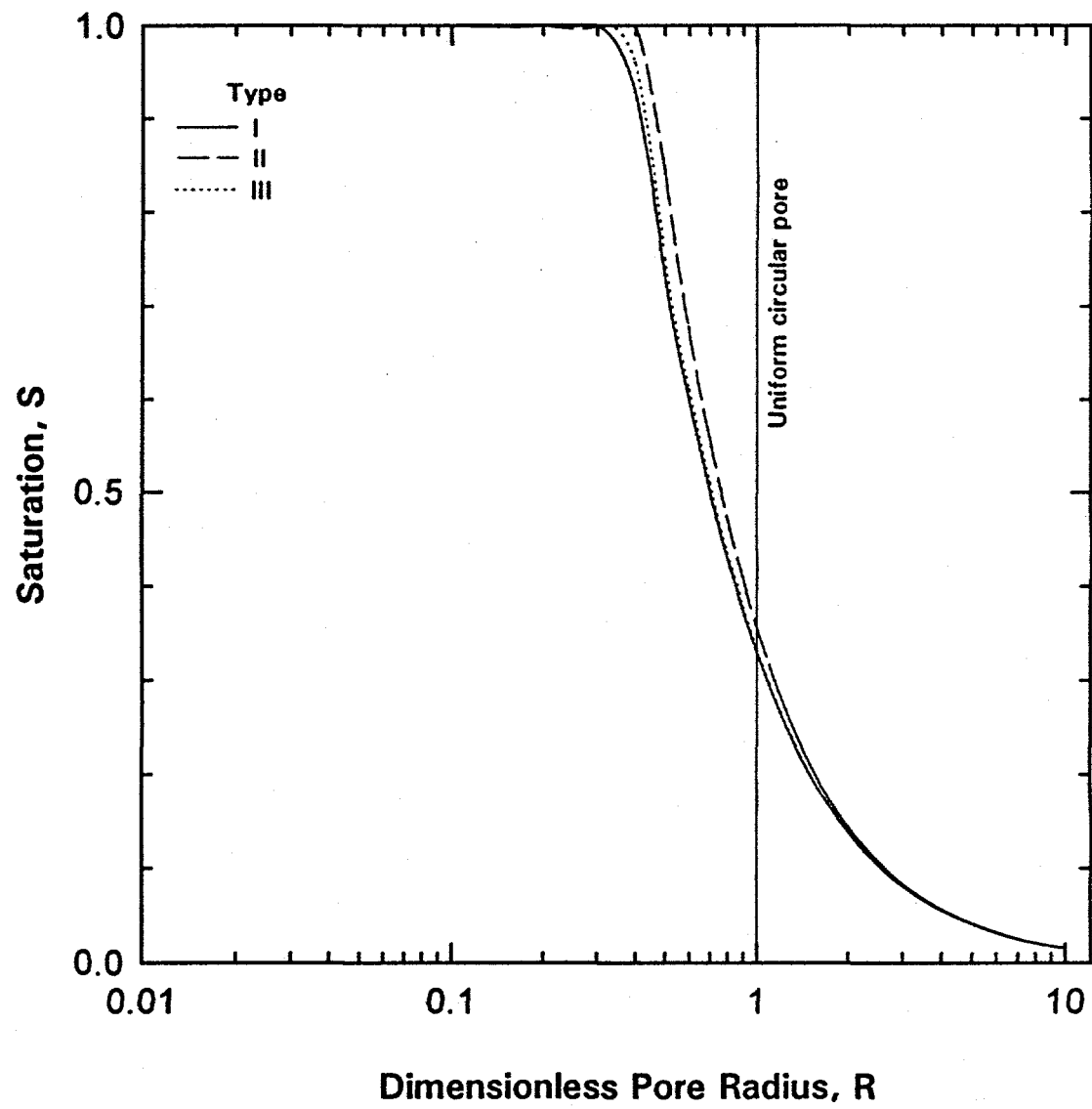
Figure 10. Effect of pore shape on residual saturation.
