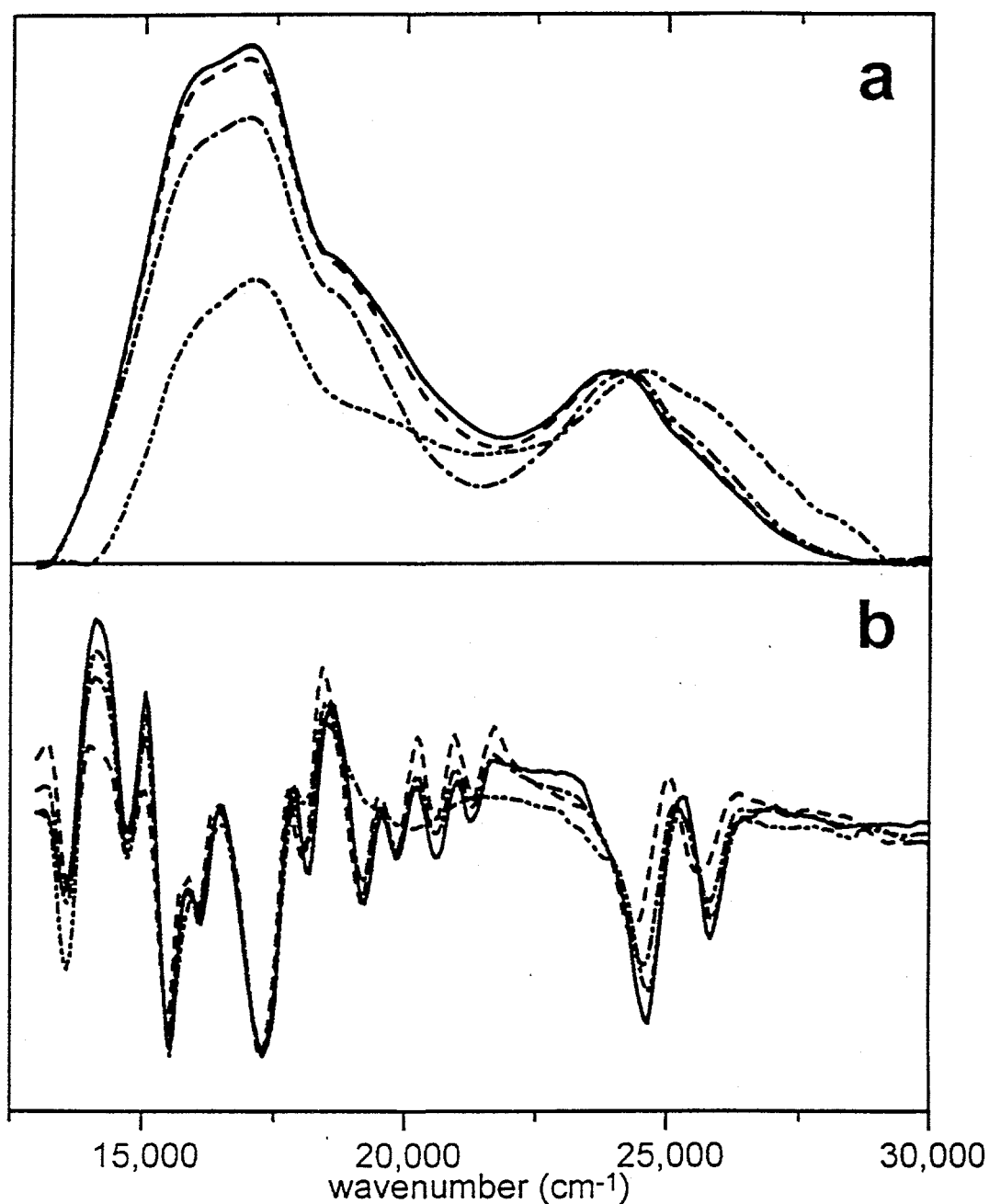
FIGURE 8. The effect of Co(II) concentration on the normalized VIS spectra of Co(II)-erionite samples dehydrated at 525°C. (a) The VIS spectra for 1.2 (---), 3.2 (-.-.-), 7.9 (....), and 8.2 (—) wt% Co samples were separately normalized to 1 at the intensity maxima of the bands at 25,000 \text{cm}^{-1} . The spectrum of the parent zeolite was subtracted. (b) Second derivative mode analysis of VIS spectra of the Co(II)-erionites with 1.3 (---), 3.2 (-.-.-), 7.9 (....), and 8.2 (—) wt% Co(II).
