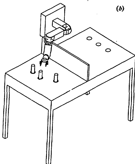
Fig. 10. CATIA simulation of telerobot performing task around an obstacle: (a) step 1, (b) step 2, and (c) step 3
