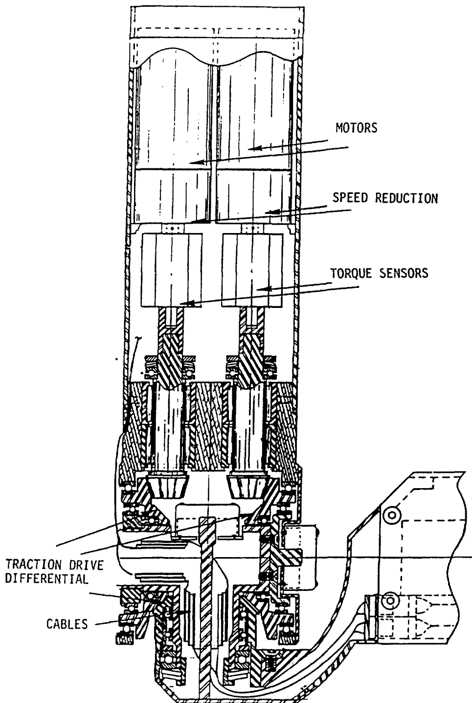
Fig. 6. Telerobot typical joint assembly
