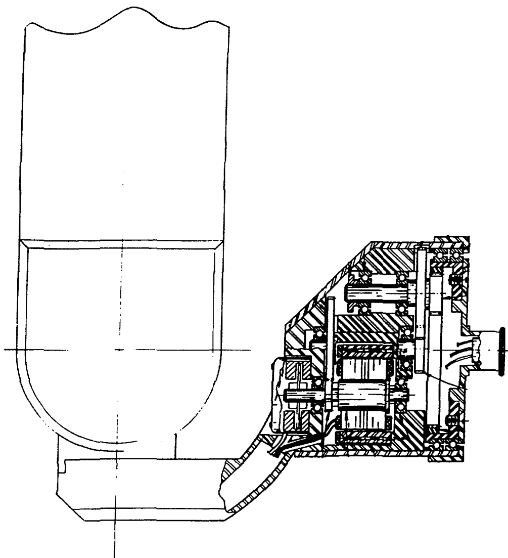
Fig. 8. Telerobot distributed wrist roll joint
