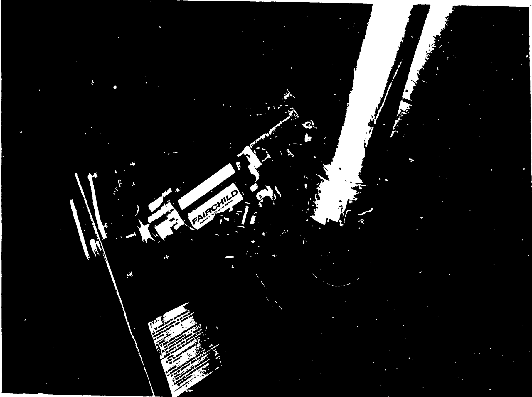
Fig. 1. M-2 operating Fairchild satellite refueling coupling
