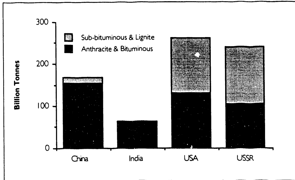
Figure I-5. Coal Reserves
