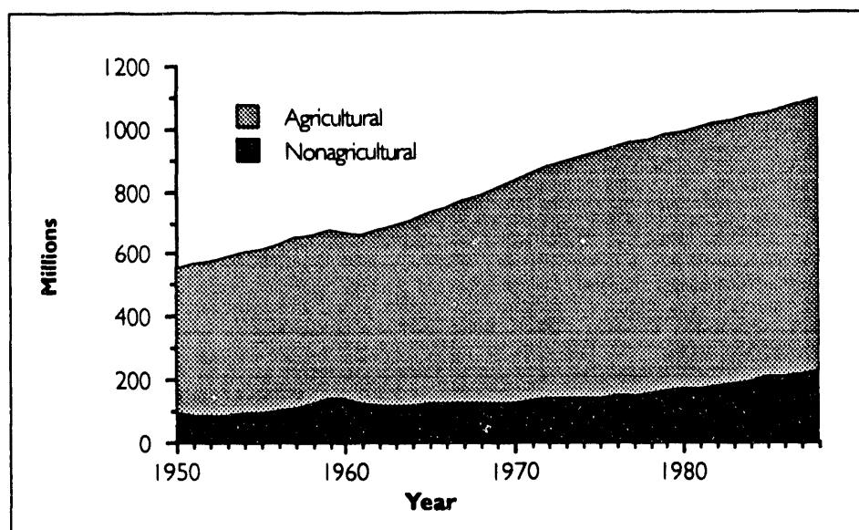
Figure IX-9. Population, 1950-1988
