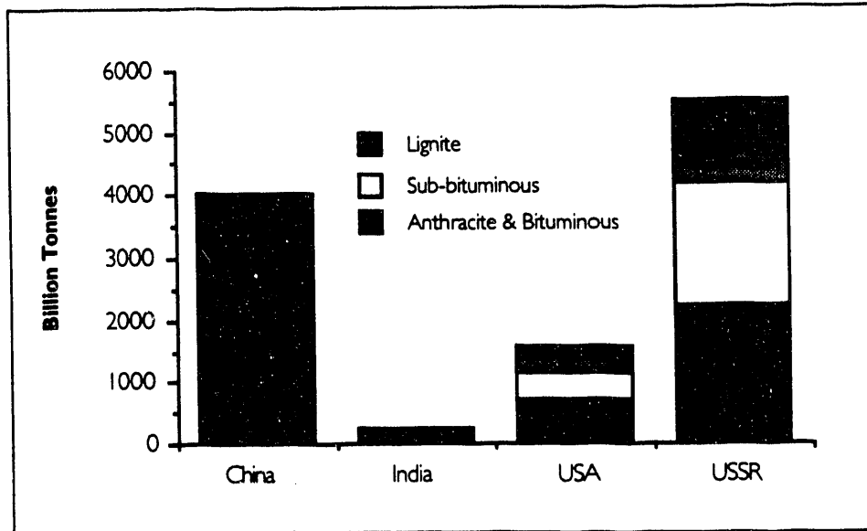
Figure I-1. Coal Resources
