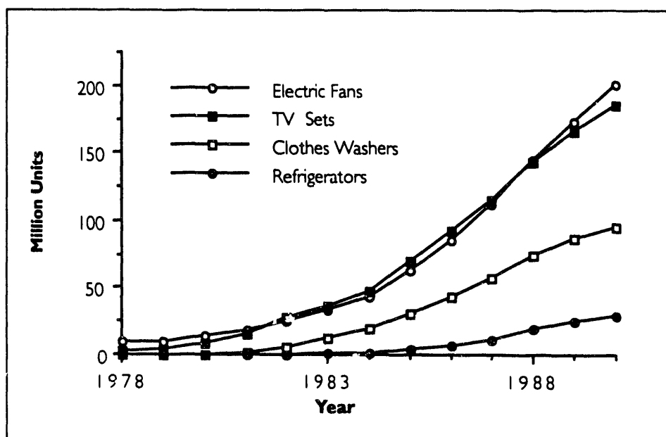
Figure V-5. Appliance Stocks, 1978-1990
