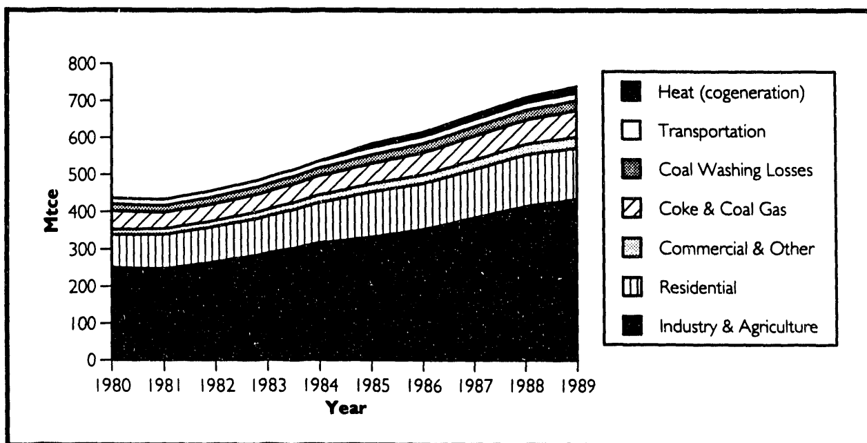
Figure IV-18. Coal Consumption by End-Use Sector, 1980-1989: Coal Inputs to Electricity Generation Attributed to Electricity End-Use Sectors*
