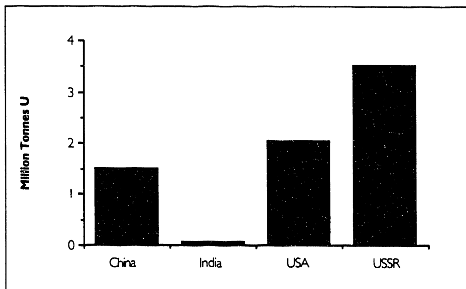
Figure I-4. Uranium Resources
