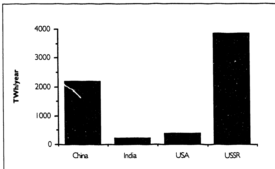
Figure I-8. Hydropower Reserves
