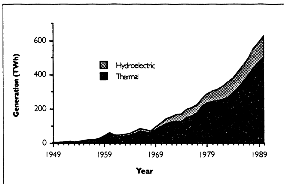
Figure II-15 Electricity Generation, 1949-1990
