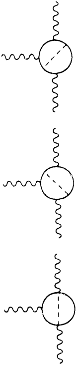
Figure 19. Two-loop corrections to the vector gauge boson propagator generated by Higgs particles.
