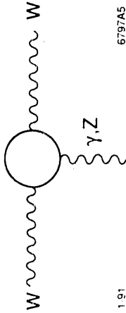
Figure 7. Loop corrections to boson propagators that generate anomalous moments.
