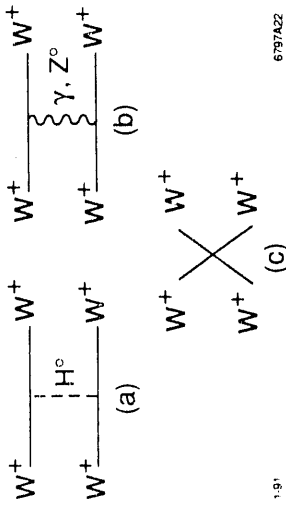
Figure 26. Feynman diagrams that contribute to W^+W^+ scattering.
