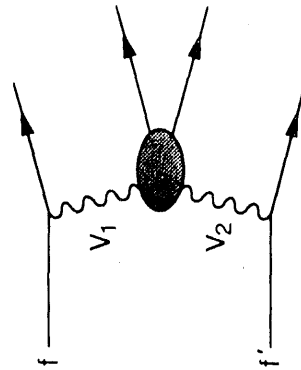
Figure 33. Peripheral scattering of gauge bosons in e^+e^- collisions.
