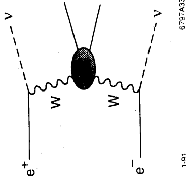
Figure 37. The W -fusion reaction in e^+e^- collisions.
