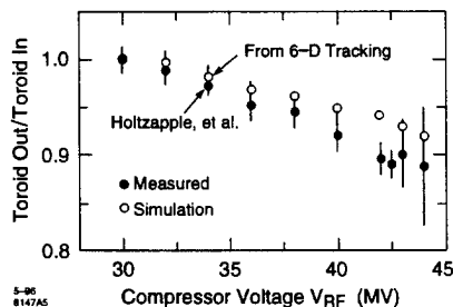
Figure 5: Transmission versus compressor voltage.
