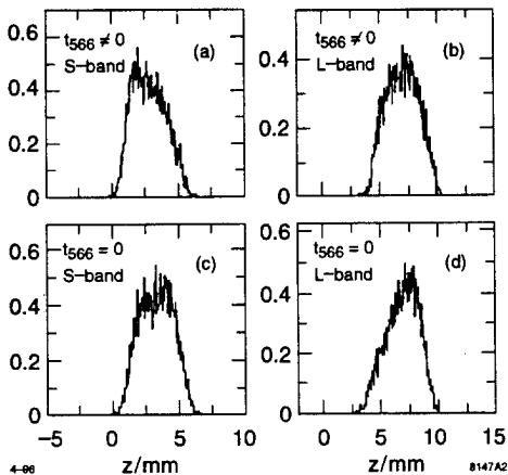
Figure 2: Effect of T_{566} and RF curvature on final bunch shape; a) expected bunch shape, b) \lambda_{RF} doubled, c) T_{566} = 0 , d) T_{566} = 0 , \lambda_{RF} doubled.
