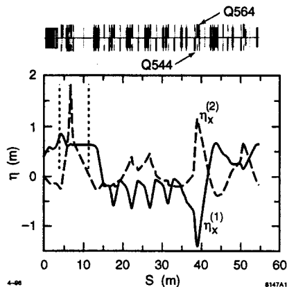
Figure 1: Magnet configuration and first & second-order dispersion in the SLC bunch compressor (RTL).
