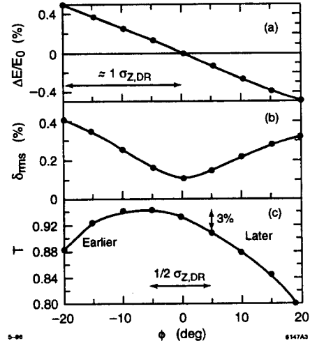
Figure 3: Sensitivity to initial phase errors; a) mean energy at end of linac, b) energy spread, c) relative transmission.
