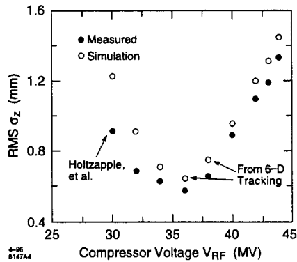
Figure 4: Bunch length versus compressor voltage
