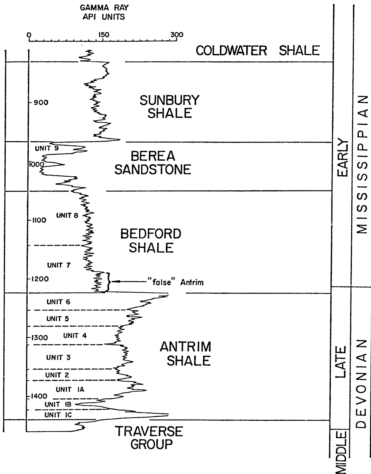
Fig. 4. Portion of gamma ray log curve from The Dow Chemical Company No. 1 Rhoburn well, Sanilac County, Well C 12, Cross Section C (Part 3). The entire sequence shown above was cored. Depths to informal Antrim, Bedford and Berea Sandstone units are shown on the core description in Appendix H. Lower strata of the Bedford are sometimes dark gray in color and may be mistaken for the Antrim.
