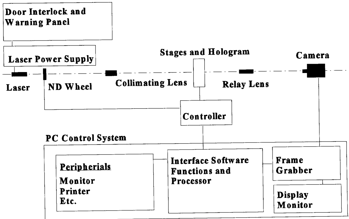
Figure 1. Sketch of Holographic Reconstruction Bench
