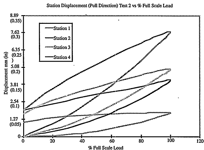
Figure 9. Displacement vs. Percent Full Scale Test Load
