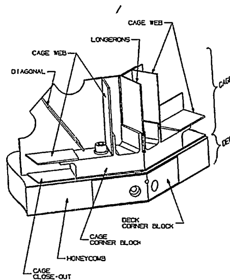
Figure 3. Structure Corner Fittings
