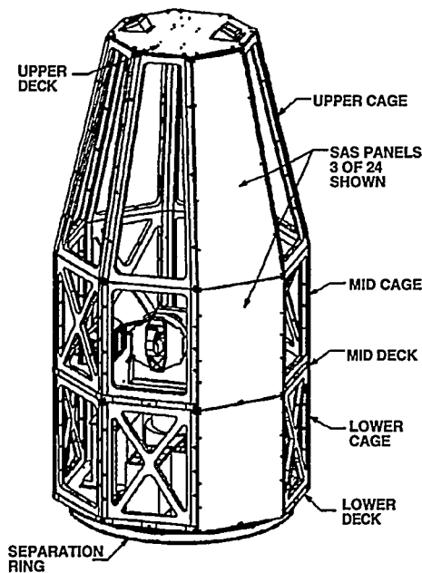
Figure 2. Structural Components
