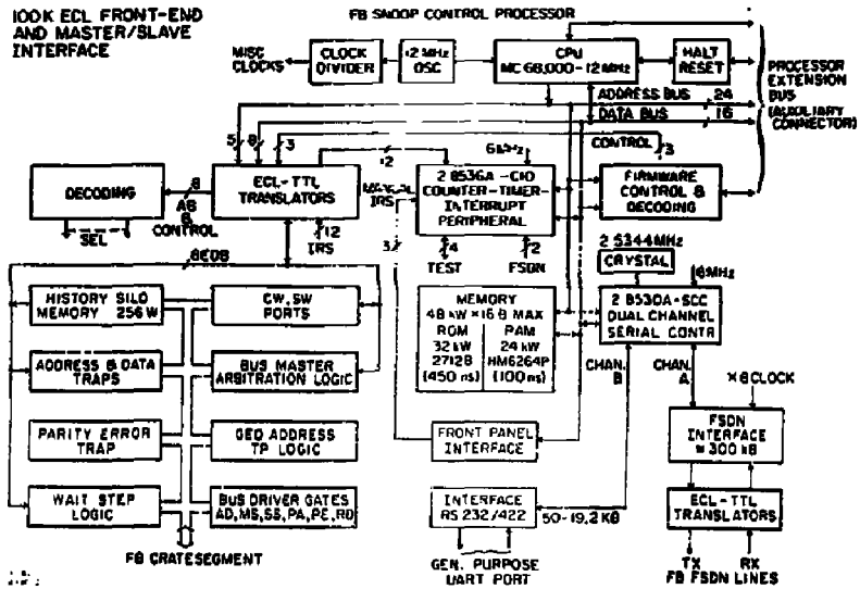
Fig. 1. SNOOP Module Block Diagram
