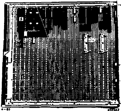
Fig. 2. Control Processor Section Prototype Board
