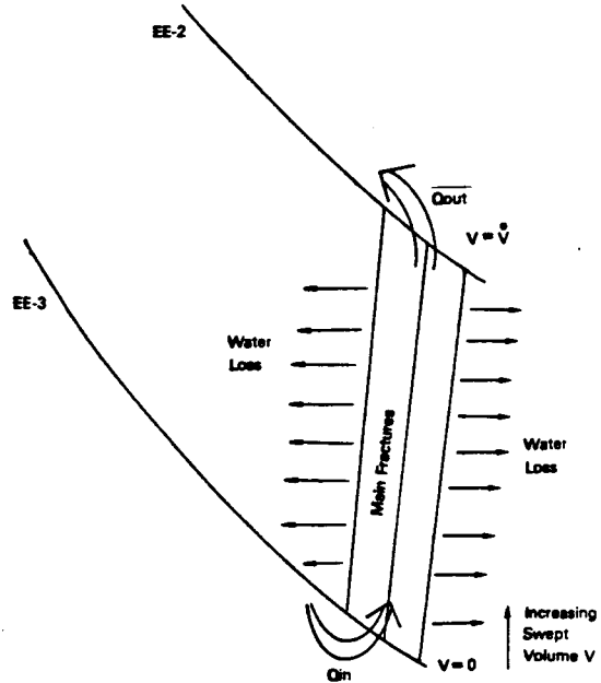
Figure 4. Schematic of Fracture Flow, Water Loss Model
