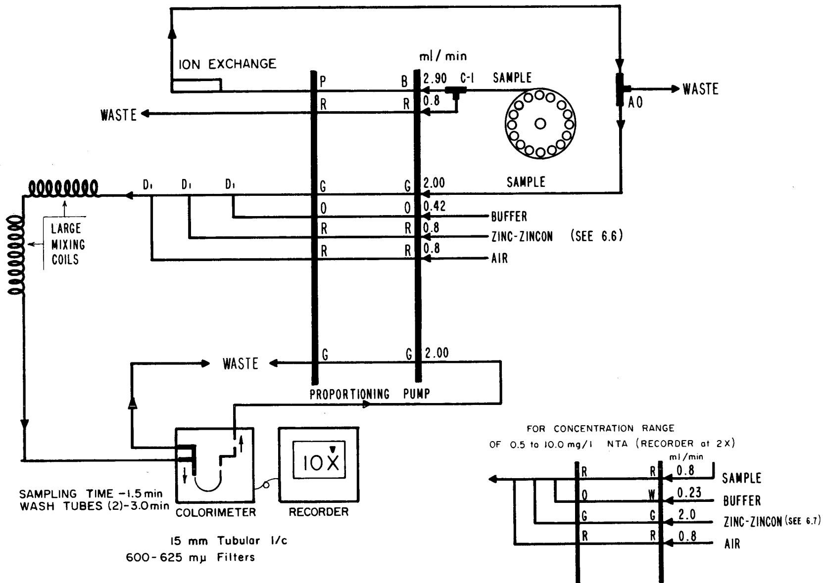
FIGURE 1. NTA MANIFOLD (0.04-1.0 mg/l NTA) AA-I
