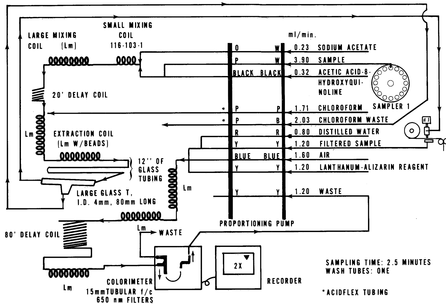
FIGURE 1. FLUORIDE MANIFOLD AA-I
