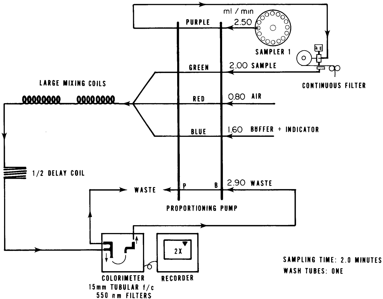
FIGURE 1. ALKALINITY MANIFOLD AA-I
