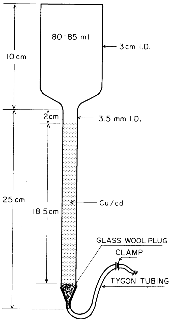
FIGURE 1. REDUCTION COLUMN
