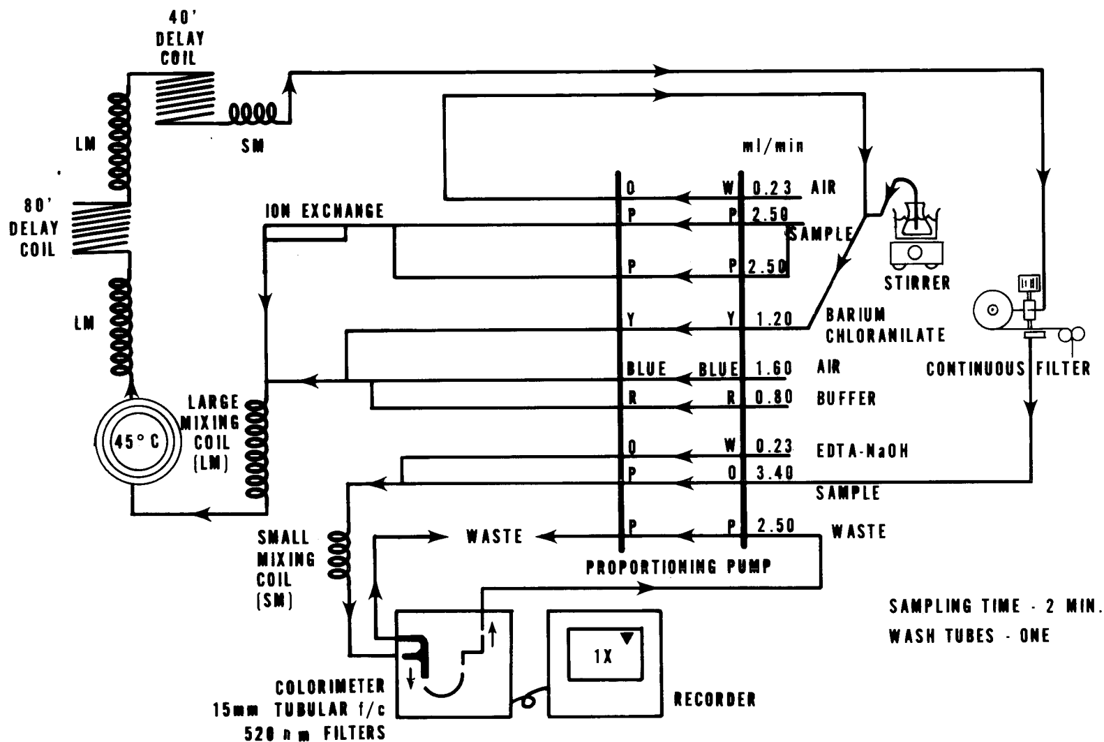
FIGURE 1 - SULFATE MANIFOLD AA-1
