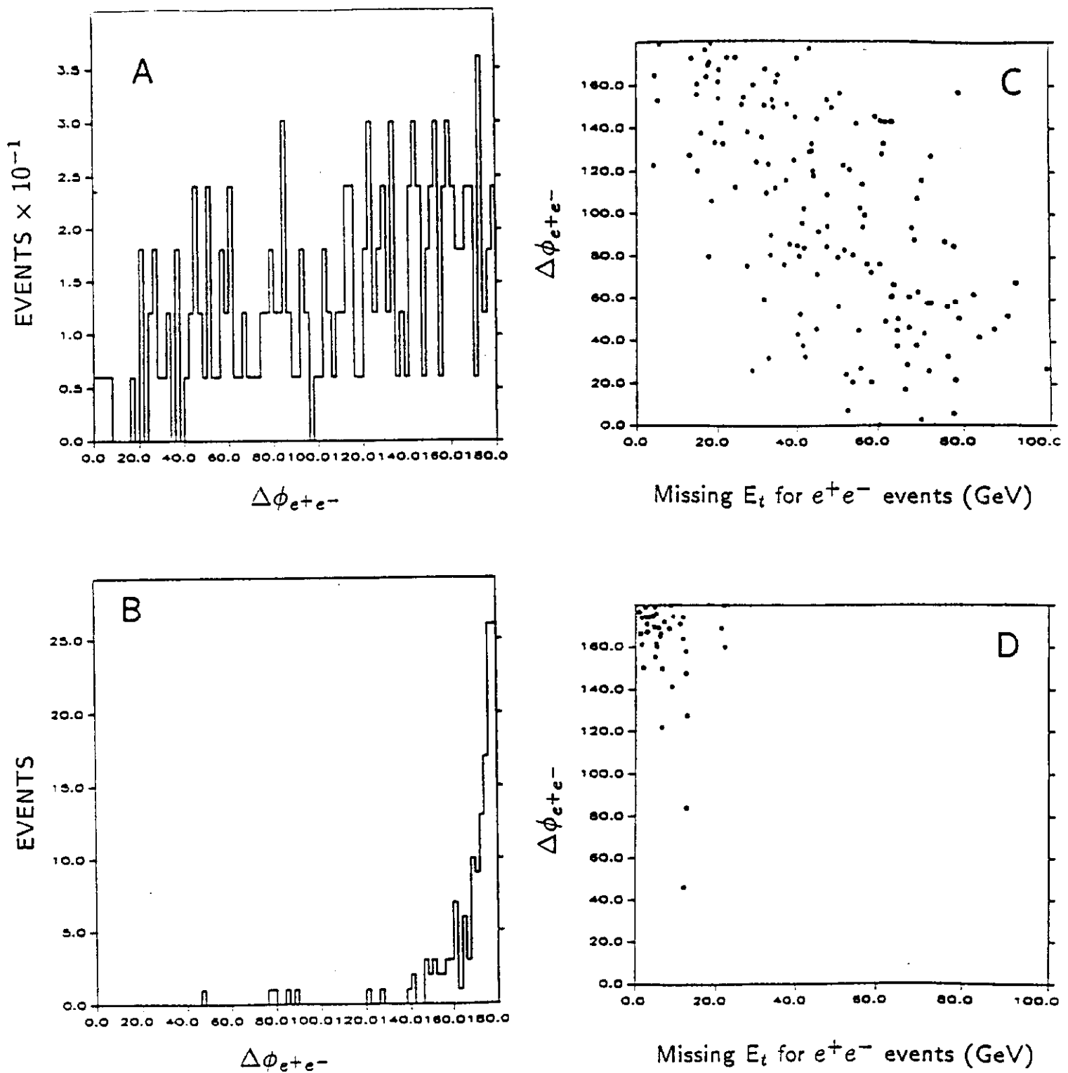
Figure 2. a) Distribution of the azimuth angle, \Delta\phi_{e+e-} , between the two electrons from a 730 \text{pb}^{-1} sample of Monte Carlo t\bar{t} events generated with top quark mass of 90 \text{GeV}/c^2 ; b) \Delta\phi_{e+e-} distribution for CDF data sample; c) \Delta\phi_{e+e-} vs \cancel{E}_t scatterplot for 90 \text{GeV}/c^2 top quark Monte Carlo events, after a M_{e+e-} cut to remove Z^0 events; d) \Delta\phi_{e+e-} vs \cancel{E}_t scatterplot for CDF data, Z^0 events removed.
