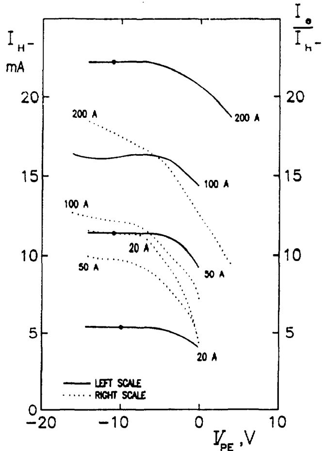
Figure 6. H^- yield and the ratio I_e/I_{H^-} vs. plasma electrode bias.
