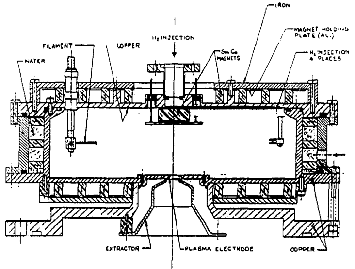
Figure 1. Cross section of the source.
