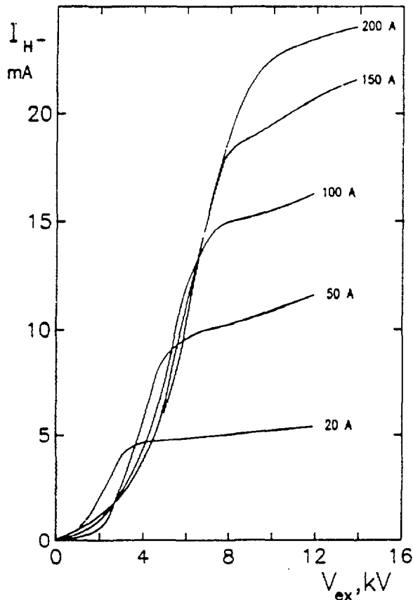
Figure 5. H^- yield vs. the extraction voltage.
