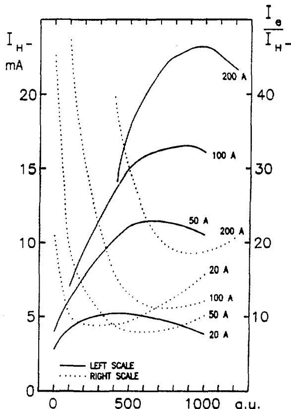
Figure 4. H^- yield and the ratio I_e/I_{H^-} vs. gas pressure.
