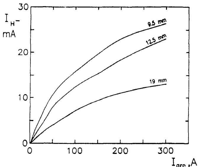
Figure 3. H^- yield vs. arc current, with the conical dipole field as parameter.
