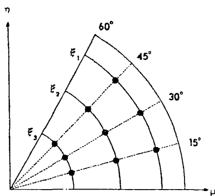
Figure IV.2c. Rectangular arrangement.
