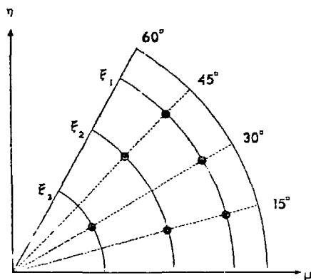
Figure IV.2b. Triangular arrangement.
