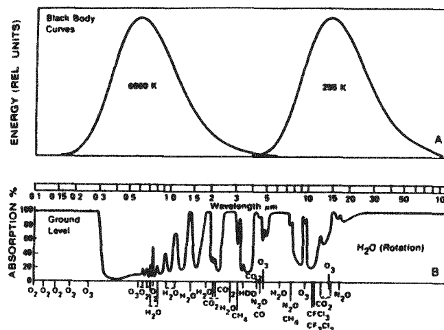
Figure 1—Radiant energy spectra of sun (at Earth distance) and Earth (above) and absorption bands of atmospheric gases (below). Wavelengths shown on center scale. (from Luther and Ellingson, 1985).
