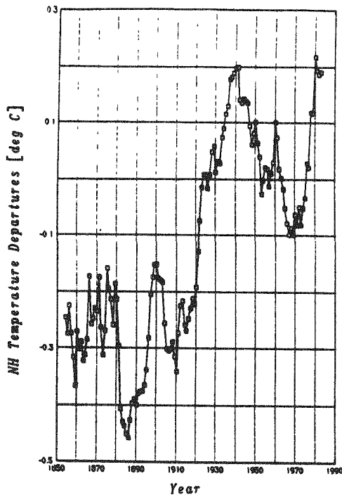
Figure 8—Plot of 7-year running average of the data in Fig. 4.
