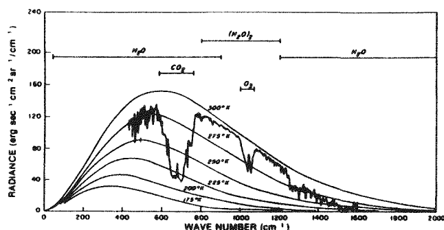
Figure 3—Terrestrial IR emission spectra recorded by IRIS-D on Nimbus IV near Guam at 15.1°N on 27 April 1970 (from Luther and Ellingson , 1985).
