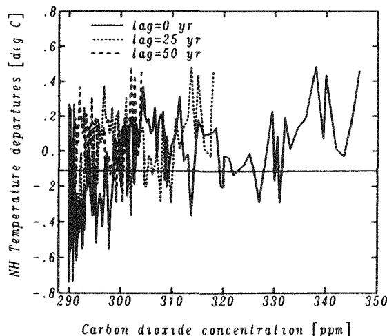
Figure 5—Plot of NH temperature data from Fig. 4 versus the atmospheric concentration of CO 2 at the time of the observation based on Pearman's (1980) model.
