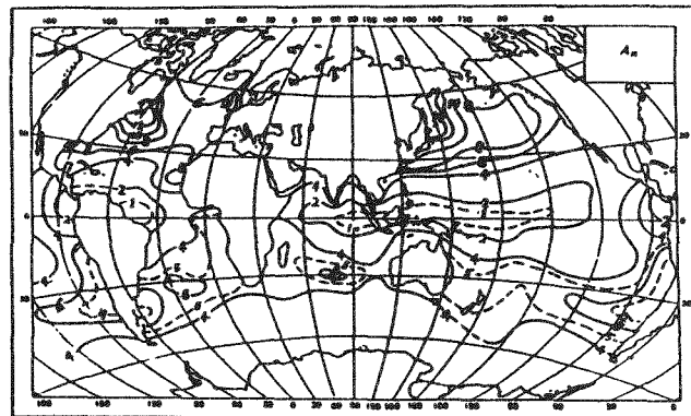
Figure 7—Map of the seasonal range in sea surface temperature in degrees C (adapted from Panfilova, 1972).
