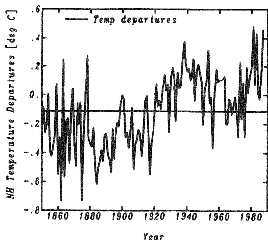
Figure 4—Northern Hemisphere surface air temperature annual mean departures from the 1951-1970 mean (re-plotted from Jones et al. , 1986).
