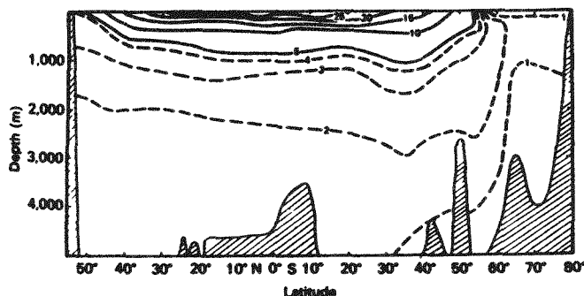
Figure 6—North-south section of water temperature [°C] in the Pacific Ocean approximately along the 170°W meridian (from Hamon and Godfrey, 1975 p. 33).
