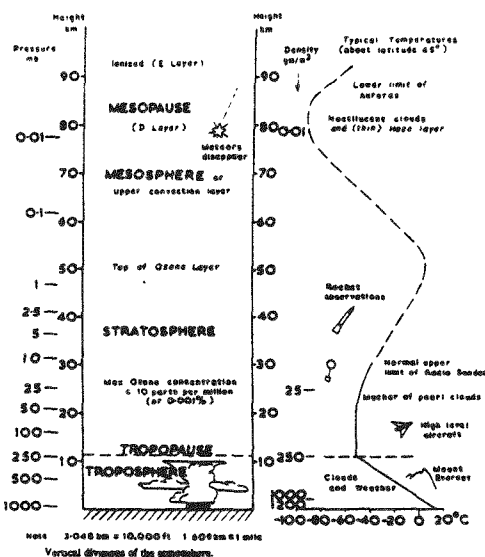
Figure 2—Typical vertical variation of temperature within the atmosphere and nomenclature for the various levels and layers. (from Lamb, 1972, p. 9).
