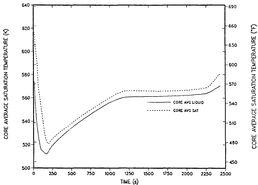
Fig. 51. Core-liquid temperatures during the MSLB/LOFW event for base transient.
