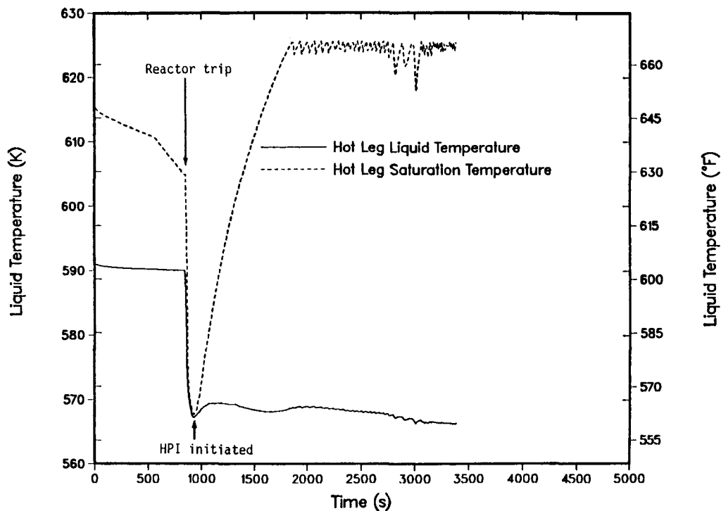
Fig. 22. Hot-leg temperatures during the SGTR/LOFW event for feed initiated on low primary pressure (11.4 MPa).
