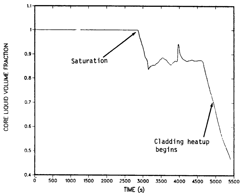
Fig. 46. Core-liquid volume fraction during the LOFW event for feed and bleed initiated at containment overpressure.
