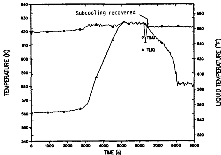
Fig. 78. Cold-leg temperatures during the LOFW event for feed initiated at rapid core heatup.
