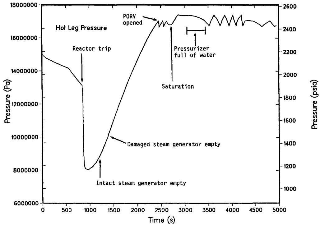
Fig. 20. Primary-system pressure during the SGTR/LOFW event for base transient.
