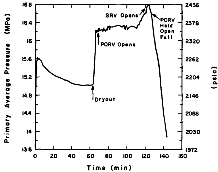
Fig. 68. Primary pressure during the LOSP event for feed-and-bleed case.
