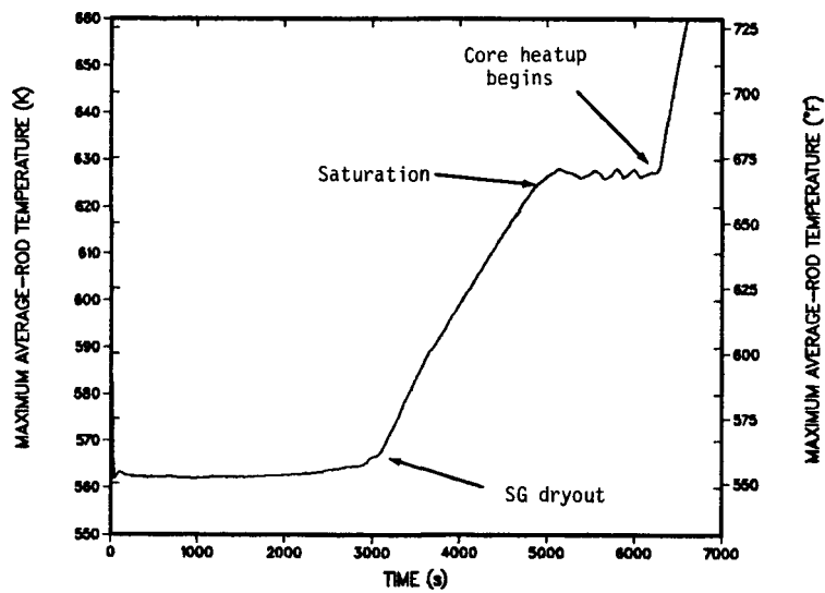
Fig. 75. Cladding temperatures during the LOFW event for base-case transient.
