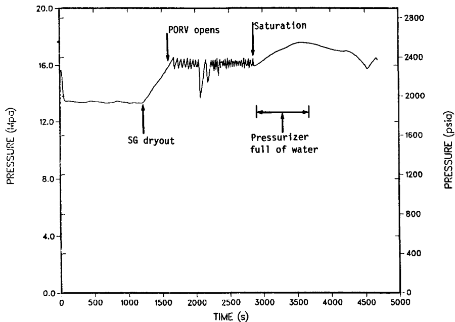
Fig. 34. Primary pressure during the LOFW event for base transient.
