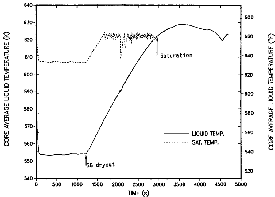
Fig. 35. Core-liquid temperatures during the LOFW event for base transient.
