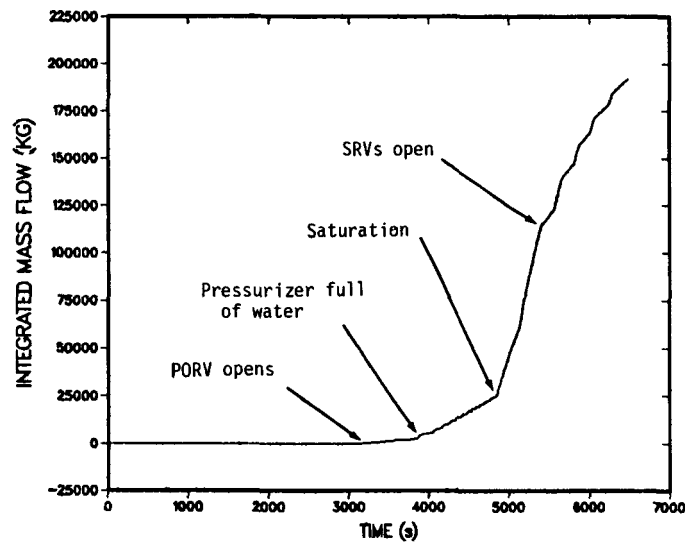
Fig. 73. Pressurizer relief flow during LOFW event for base transient.
