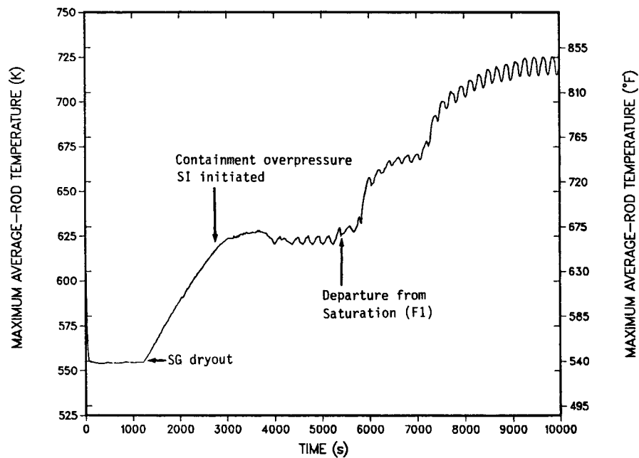
Fig. 38. Cladding temperature during the LOFW event for feed initiated at containment overpressure.
