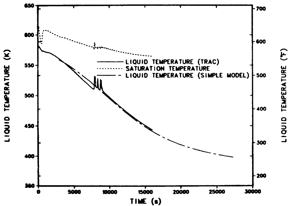
Fig. 8. Hot-leg temperatures during the LOSP/LOFW event for feed and bleed initiated at 120 s.
