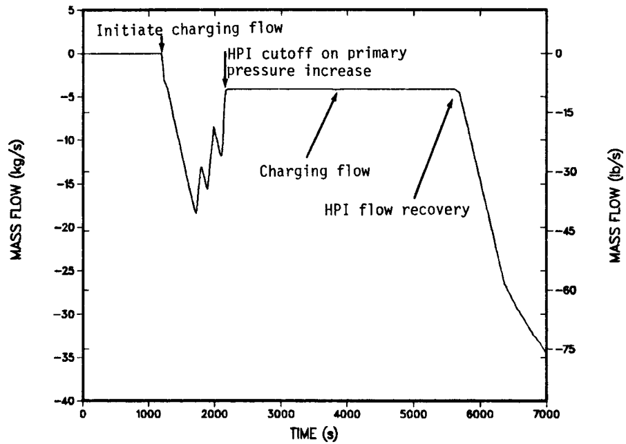
Fig. 43. Safety injection flow rate during the LOFW event with feed and bleed initiated at SGSD.
