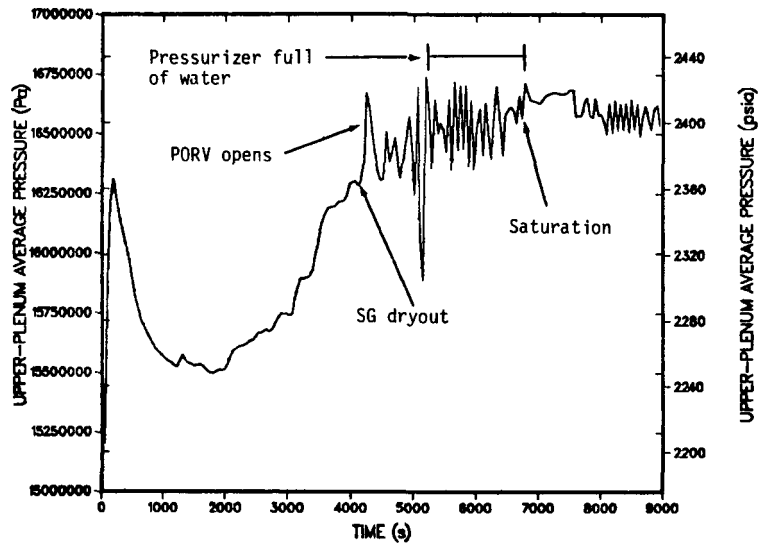
Fig. 62. Primary pressure during the LOSP event for base transient.
