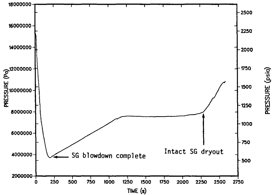
Fig. 48. Primary pressure during the MSLB/LOFW event for base transient.
