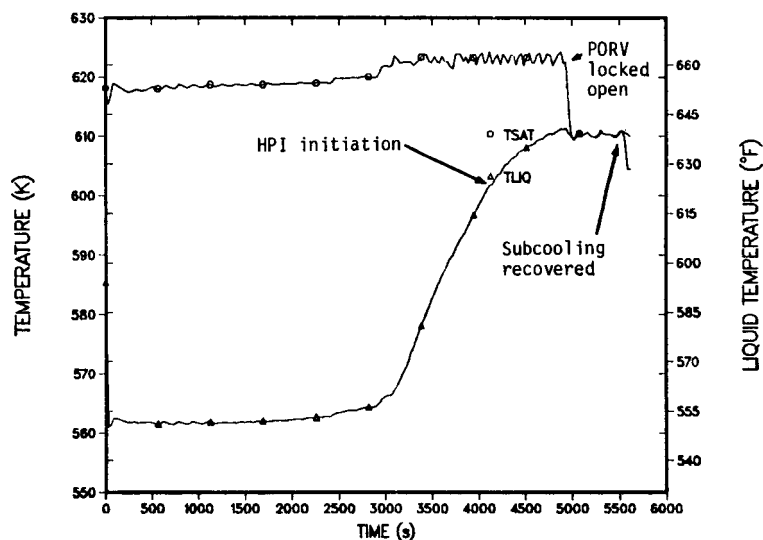
Fig. 79. Hot-leg temperatures during the LOFW event for feed and bleed initiated at containment overpressure.
