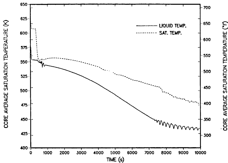
Fig. 40. Core-liquid temperature during the LOFW event for feed and bleed initiated at 300 s.
