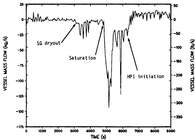
Fig. 77. Net vessel mass flow during the LOFW event for feed initiated at rapid core heatup.
