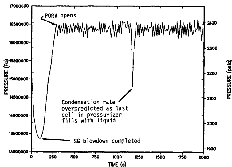
Fig. 86. Primary pressure during the MSLB/LOFW event for feed initiated at 0.8 s.
