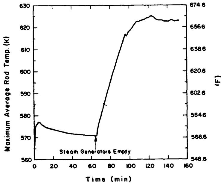
Fig. 67. Cladding temperatures during the LOSP event for feed initiated on high containment overpressure.
