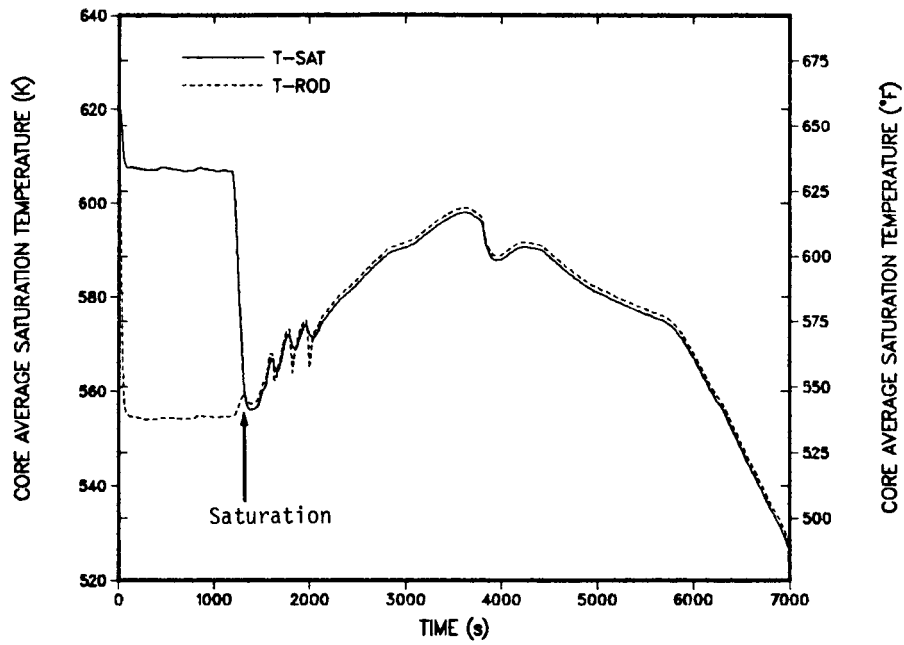
Fig. 42. Cladding temperature during the LOFW event for feed and bleed initiated at SGSD.
