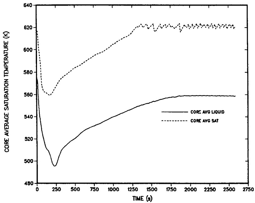
Fig. 55. Core average temperatures during the MSLB/LOFW event with feed initiated on low pressurizer level at 31 s.
