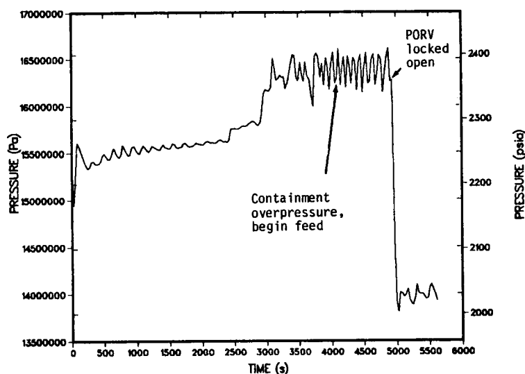
Fig. 80. Primary pressure during the LOFW event for feed and bleed initiated at containment overpressure.
