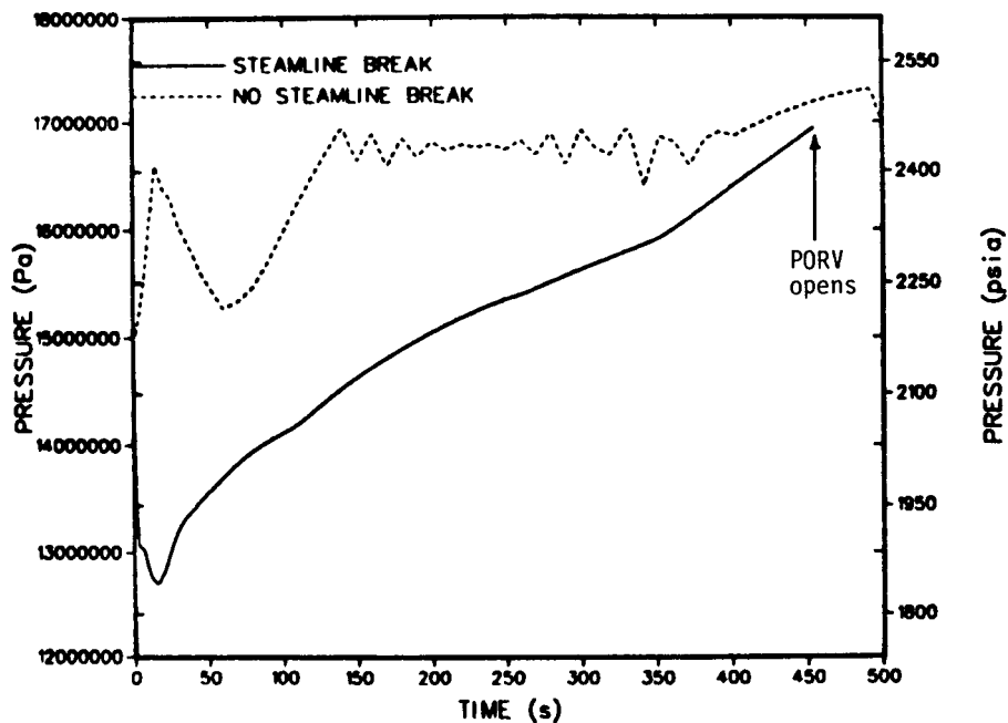
Fig. 19. Primary pressure during the MSLB/LOFW event for base transient.
