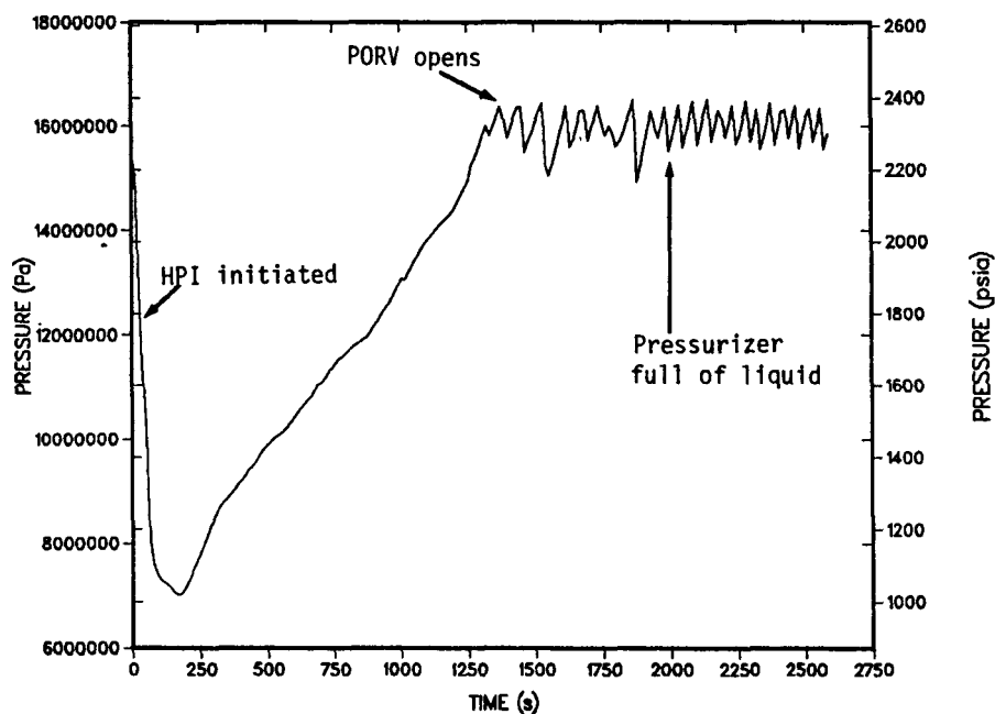
Fig. 53. Pressurizer pressure during the MSLB/LOFW event for feed initiated on low pressurizer pressure at 31 s.
