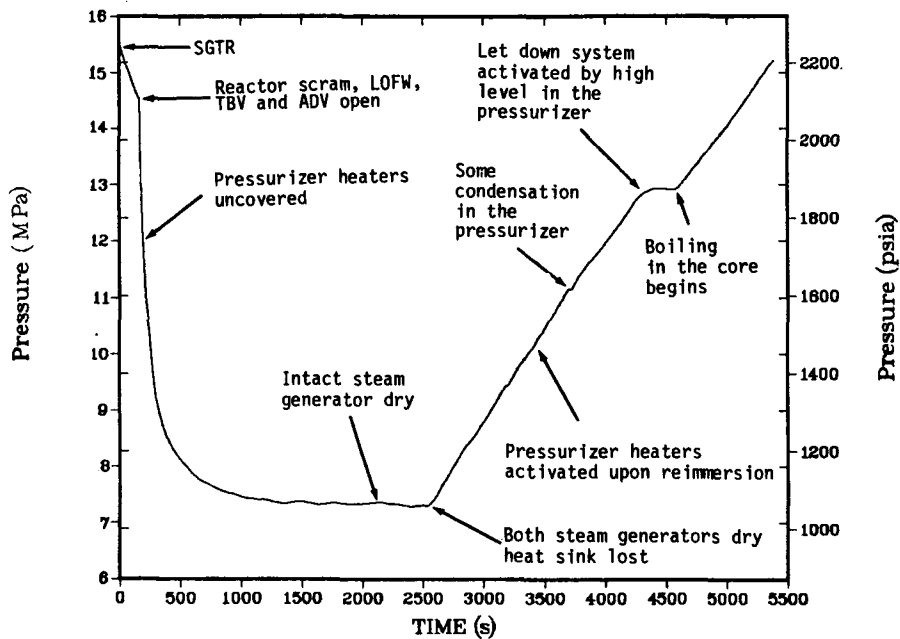
Fig. 57. Pressurizer pressure during the SGTR/LOFW event for base transient.
