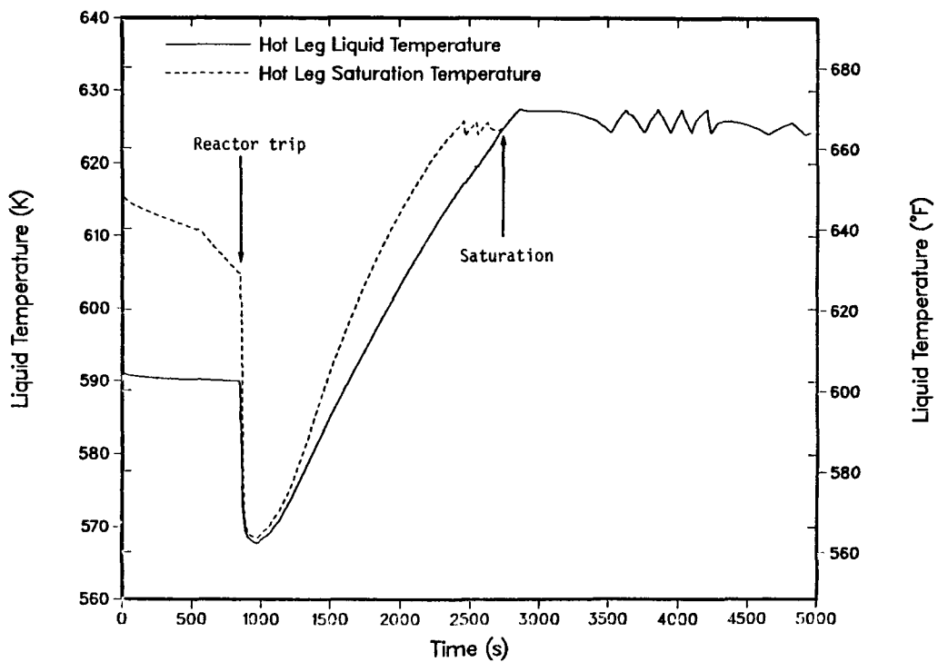
Fig. 21. Hot-leg temperatures during the SGTR/LOFW event for base transient.
