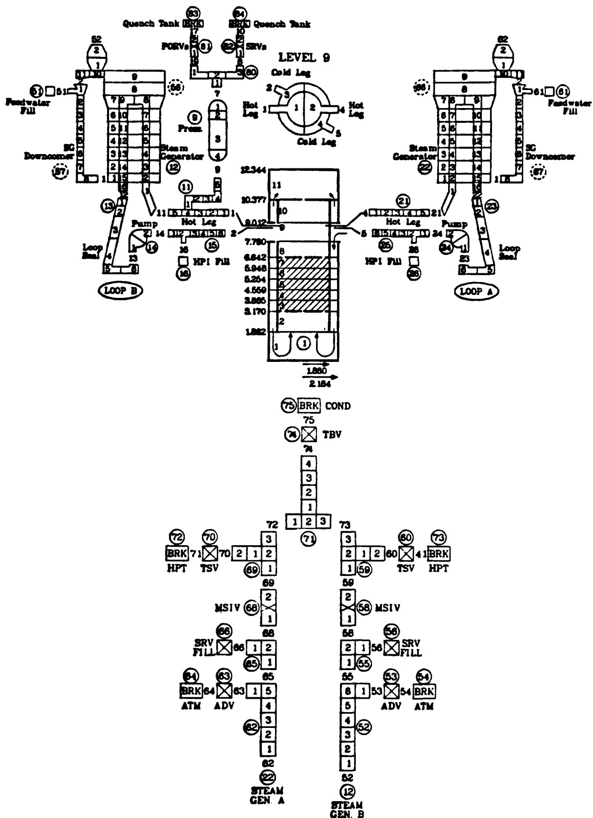
Fig. B.2. TRAC noding of Calvert Cliffs-1 with combined cold legs.
