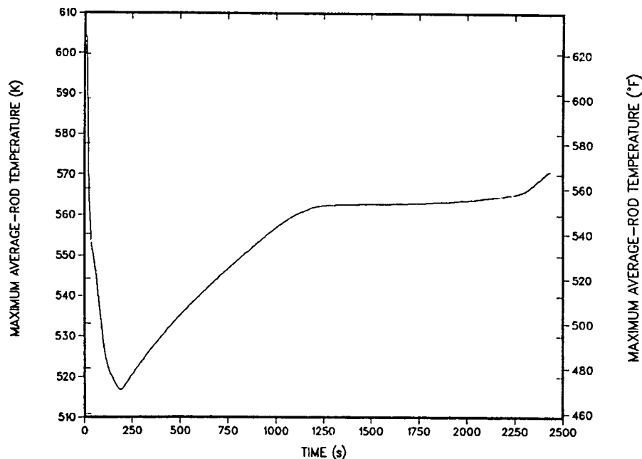
Fig. 50. Cladding temperatures during the MSLB/LOFW event for base transient.
