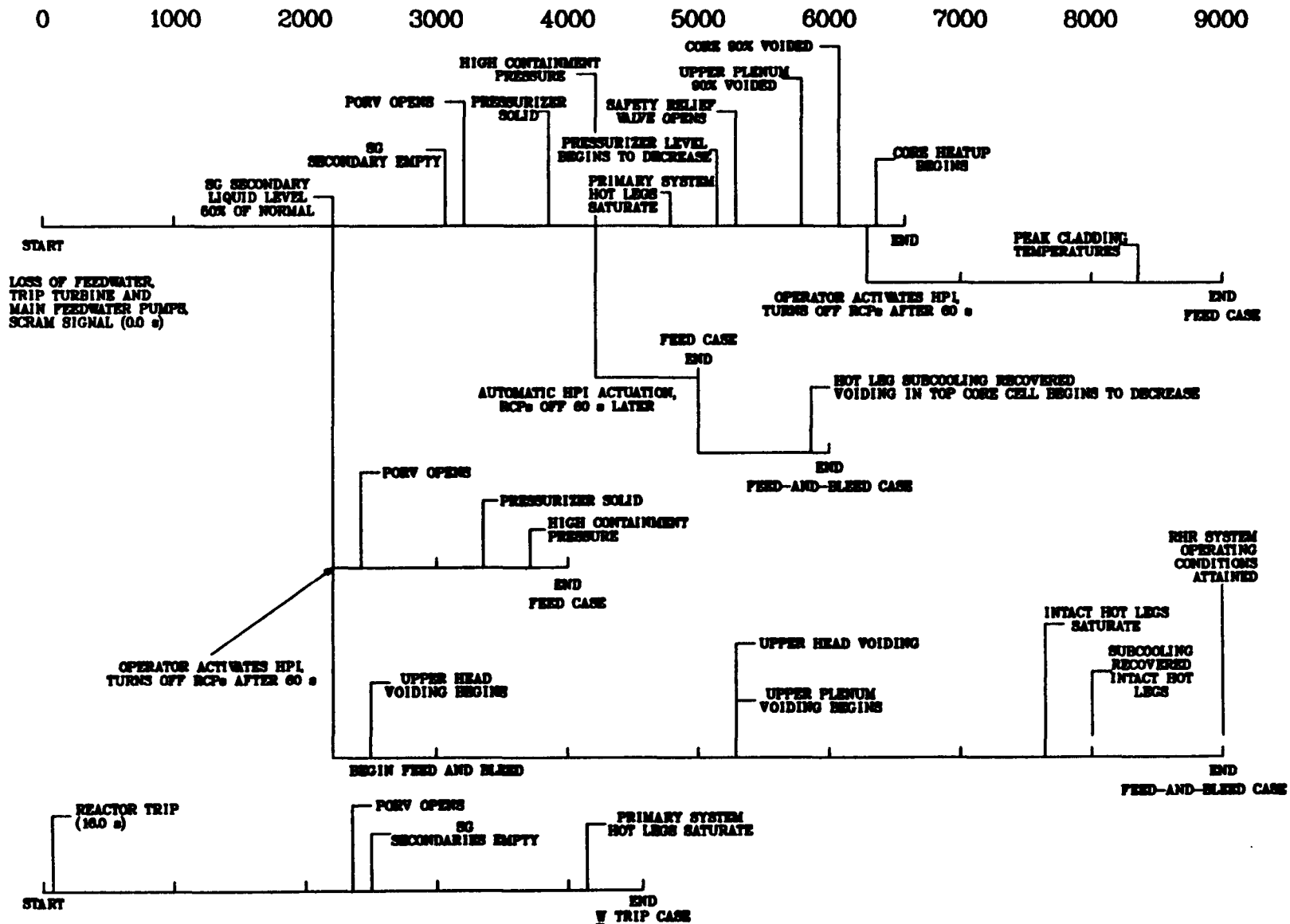
Fig. 71. Zion-1 LOFW event line (nominal equipment).
