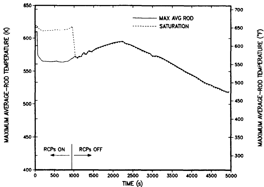
Fig. 96. Cladding temperature during a LOFW event with feed and bleed initiated at SGSD.
