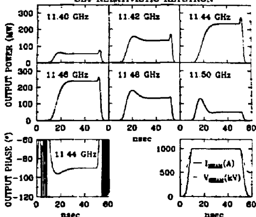
FIG. 3 Transient analysis of SL4, an 11.4 GHz six cavity relativistic klystron. In this linear calculation, the fields produced in the input cavity by the RF generator have reached equilibrium before the beam turns on. The klystron cavity frequencies without beam are tuned to 0, 32, 24, 35, 425, and 6 MHz, respectively, above 11424 MHz. The pulsed beam detunes the cavities by 25 MHz and loads them with Q_{ext} = 230 when beam current and voltage are at their maximum values, 1 kA and 1 MV. The gain cavities are loaded externally with Q_{ext} = 120 for faster risetime. Input Q_c = 300 . Output Q_c = 20 . For the six cavities, R/Q = 27, 27, 27, 27, 60 , and 511, respectively. Inter-cavity spacings are 28, 14, 21, 21, and 14 cm.
