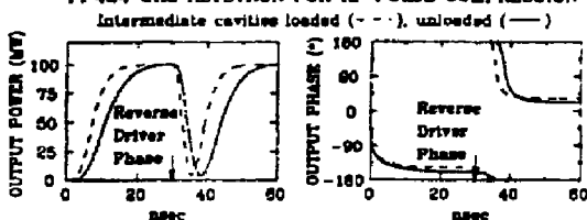
FIG. 4 Transient analysis of a 100 MW, 11.424 GHz five-cavity conventional klystron design for RF pulse compression. In this linear calculation, the RF generator is switched on at 0 nsec in the presence of a DC beam. The generator phase is reversed at 30 nsec, after the switch-on transient has subsided. Dashed curves show that improved risetime is obtained by adding external loads with Q_{ext} = 150 to the gain cavities. Input Q_c = 190 . Output Q_c = 26 . The klystron cavity frequencies without beam are tuned to 21, 18, 40, 500, and 20 MHz, respectively, above 11424 MHz. The DC, 510 A, 440 kV beam detunes the cavities by -21 MHz and loads them with Q_{ext} = 210 . For the five cavities, R/Q = 36, 36, 36, 39 , and 201, respectively. Inter-cavity spacings are 6, 6, 8, and 3 cm.
