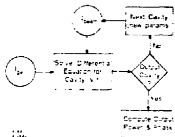
FIG. 2 Flowchart for klystron transient calculations
