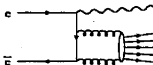
Fig. 1. Radiative J/\psi Decays
