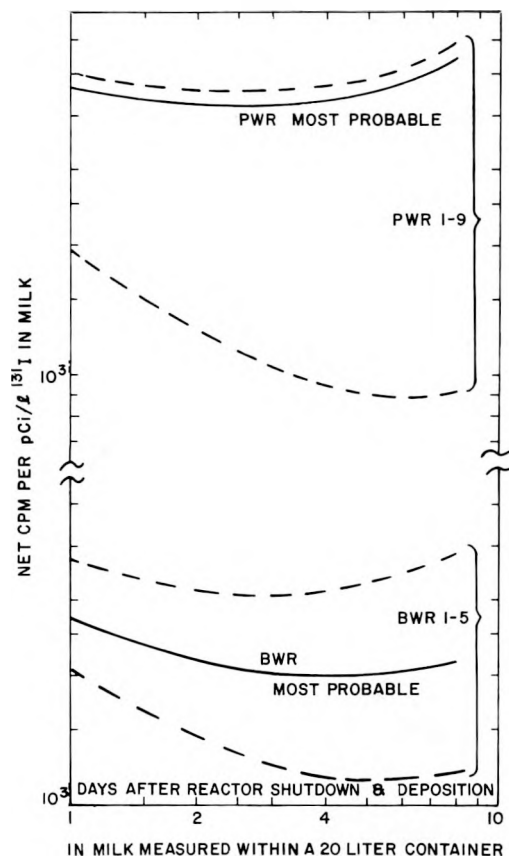
Figure 3.2 6306 Probe Response to WASH 1400 Fission Products in Milk Measured Within a 20 Liter Container
