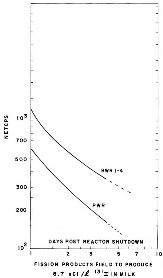
Figure 2.3 6306 Probe-on-Meter Response 1 Meter Above an Infinite Fission Products Field to Produce 8.7 nCi/l ^{131}\text{I} in Milk
