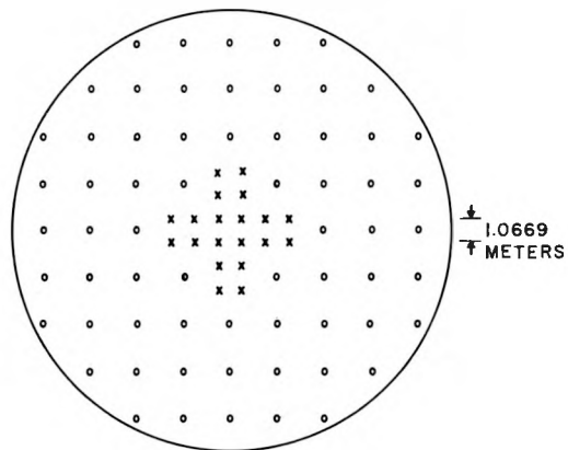
Figure 2.1 Simulated ^{131}\text{I} Semi-Infinite Fallout Field
