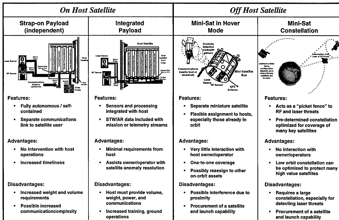
Figure 3. STW/AR Deployment Architecture Options.
