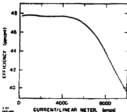
Fig. 3. Efficiency versus current, 200 kV beam energy.
