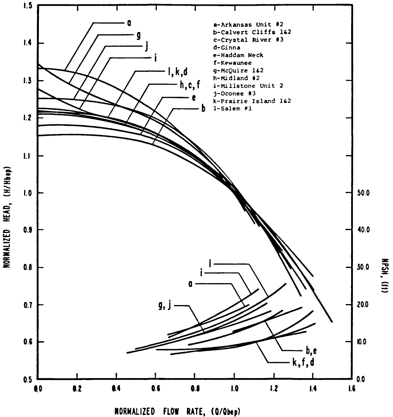
Figure 3.2a. Performance and Cavitation Curves for RHR Pumps. Head vs. Flow Rate Data Normalized by Individual Best Efficiency Point Values.
