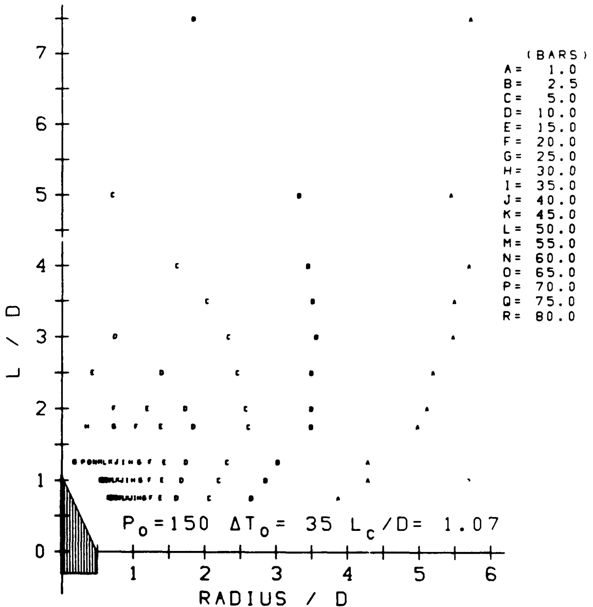
Figure C-3 Composite target pressure contours as a function of target L/D and target RADIUS/D for stagnation conditions of P_0 = 150 bars and 35 degrees of subcooling. Smooth lines connecting like alphabetic letters form an approximate pressure contour corresponding, in bars, to the pressure versus alphabetic letter key. This contour is approximate and is only informational.
