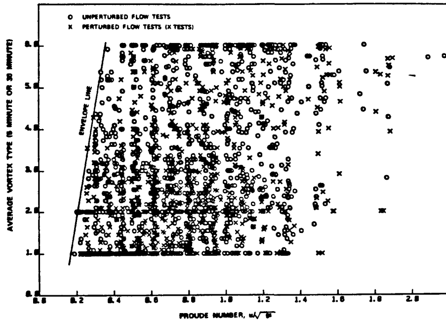
Figure 3.12. Surface Vortex Type as a Function of Froude Number; Horizontal Outlet Configuration.
