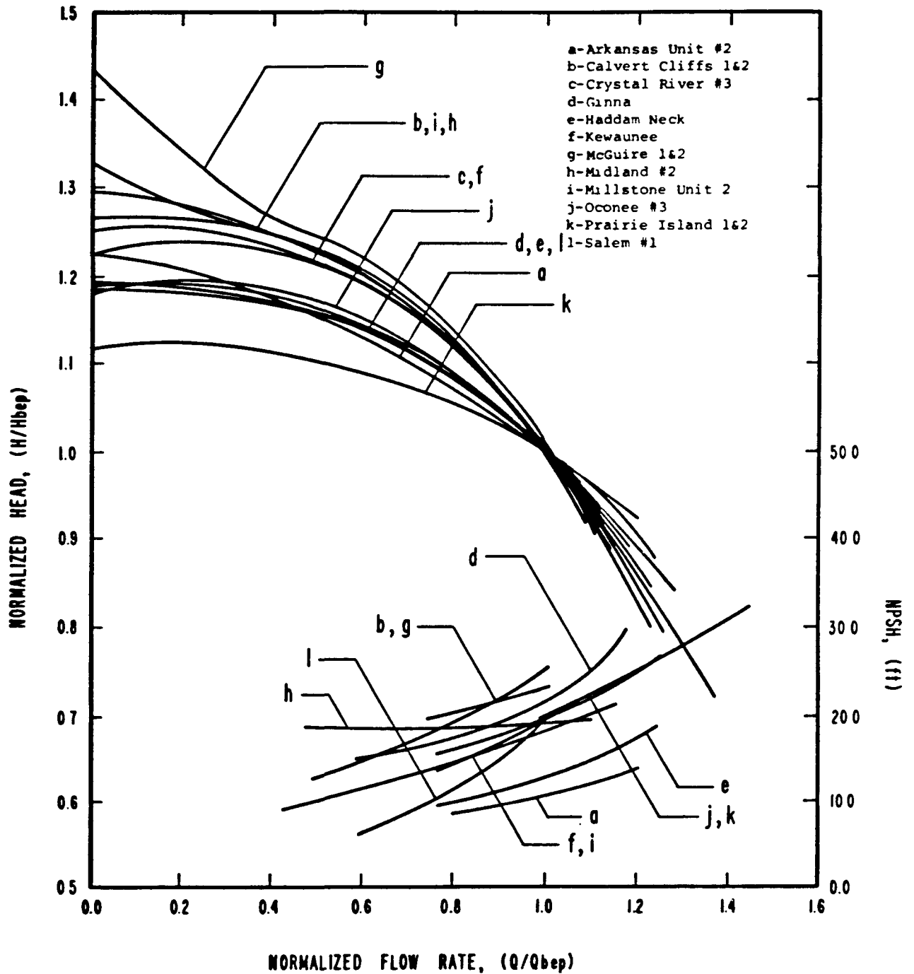
Figure 3.2b. Performance and Cavitation Curves for CSS Pumps. Head vs. Flow Rate Data Normalized by Individual Best Efficiency Point Values.
