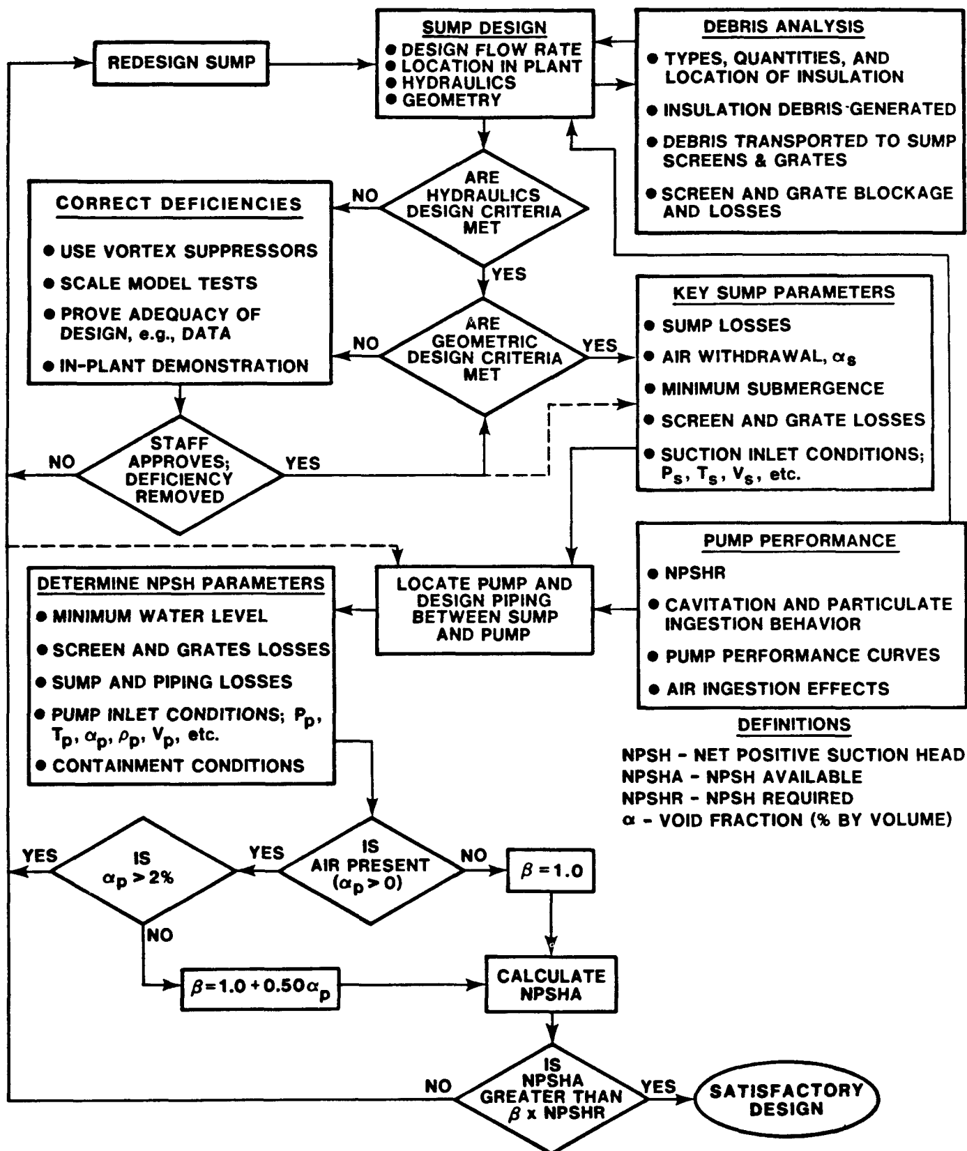
Figure 5.3. Combined Technical Considerations for Sump Performance
