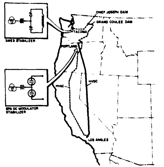
Fig. 1. - Pacific intertie transmission system routes and dynamic stabilizers
