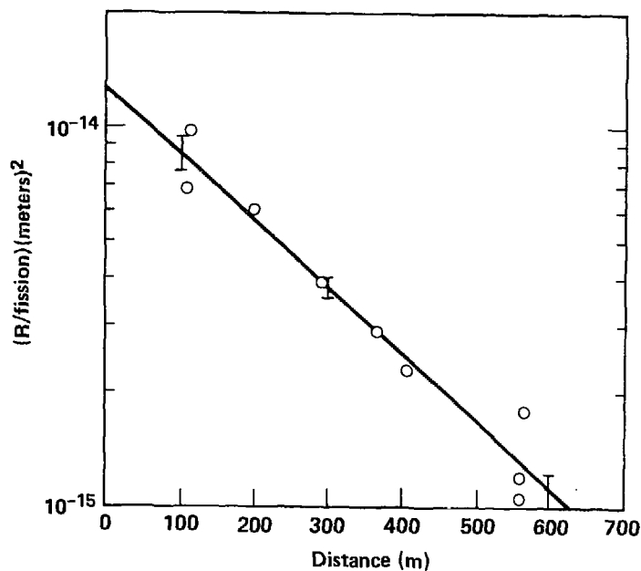
Figure 6 -- Gamma relaxation length.
