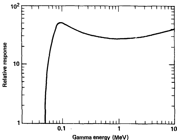
Figure 2 -- Reuter-Stokes energy dependence.
