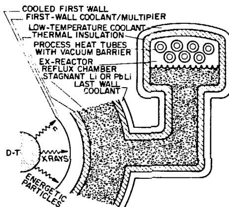
EX-REACTOR REFLUX BLANKET
