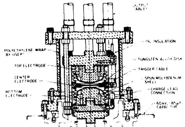
Fig. XVII-11. ZT-40 field distortion start switch.
