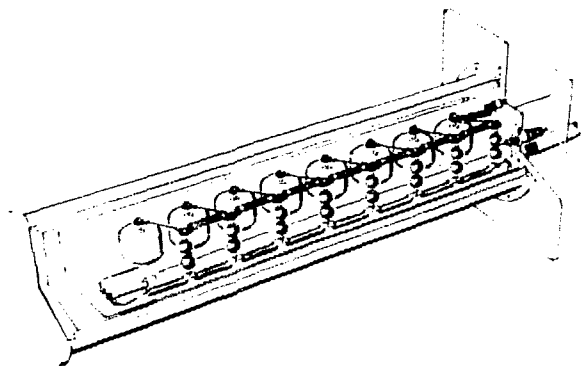
Fig. XVII-17. ZT-40 micromarx 200-kV pulse generator.
