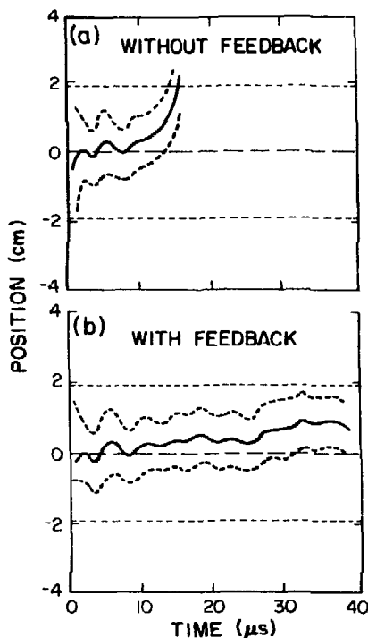
Fig. III-17. Luminosity position data showing feedback control.
