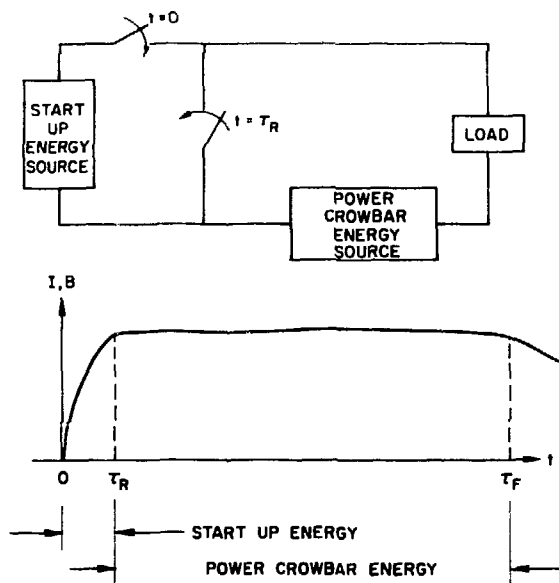
Fig. XVII-27. Basic power crowbar circuit.
