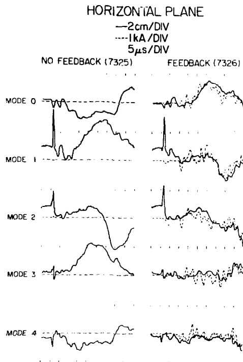
Fig. III-15. Horizontal mode amplitudes controlled by feedback.
