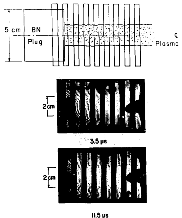
Fig. IV-9. Side view interferograms in the vicinity of boron nitride end plugs.
