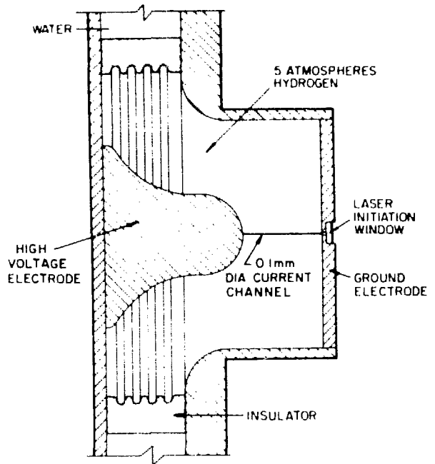
Fig. XVII-20. HDZP load geometry.
