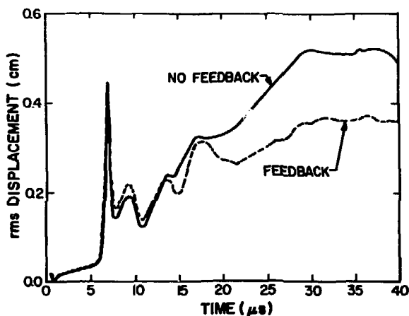
Fig. III-18. Averaged rms displacements with and without feedback stabilization.
