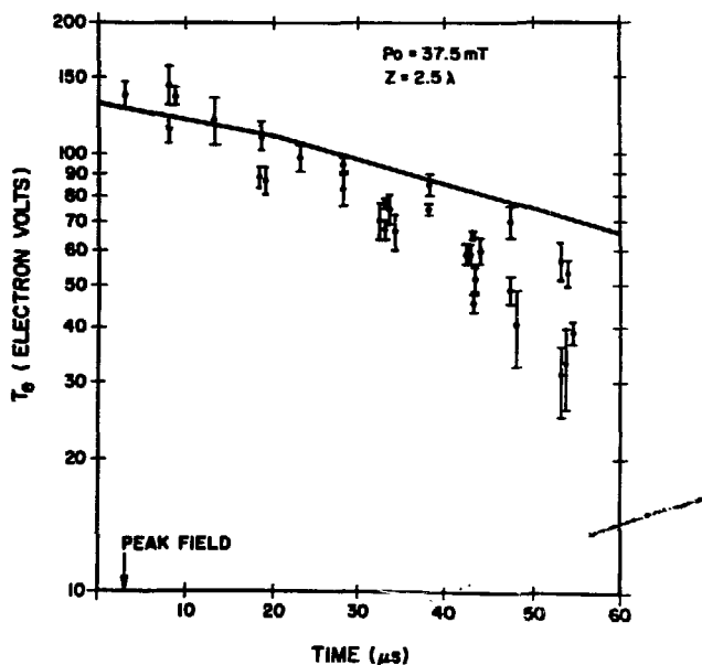
Fig. III-10. Thomson scattering temperature measurements vs time.
