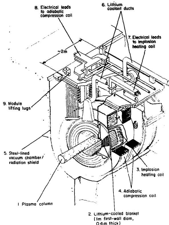
Fig. XVI-1. Cutaway view of a 2-m long, 0.5-m-radius (first-wall) Linear Theta-Pinch Reactor (LTPR) module. This module is similar to that envisaged for the Toroidal Reference Theta-Pinch Reactor (RTPR). 1,2
