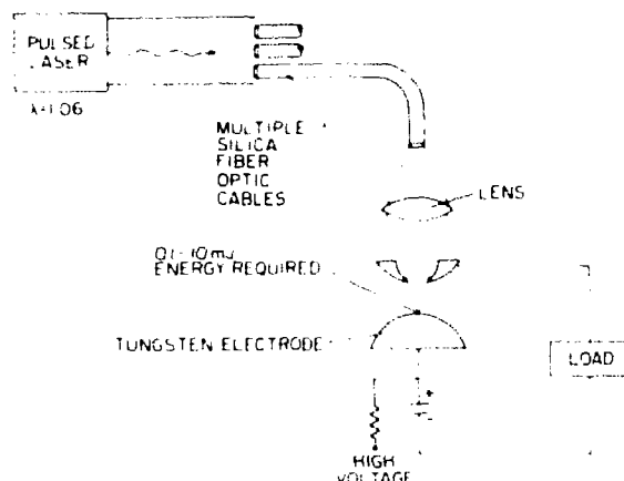
Fig. XVII-26. Laser fiber-optic spark gap trigger system.
