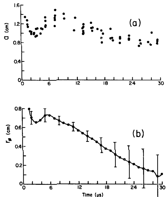
Fig. IV-3. (a) Time history of plasma radius, a , and (b) averaged excluded flux radius, r_0 .
