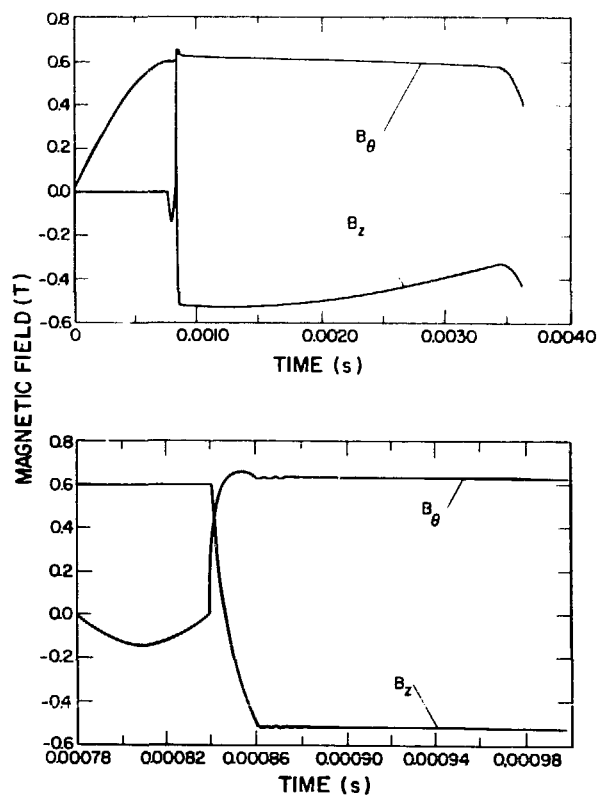
Fig. XVII-9. Representative Slow Mode II waveforms.
