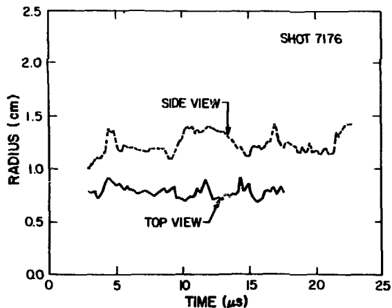
Fig. III-12. Plasma ellipticity from luminosity.
