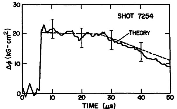
Figure III-9. Excluded flux decay compared with end-loss theory.
