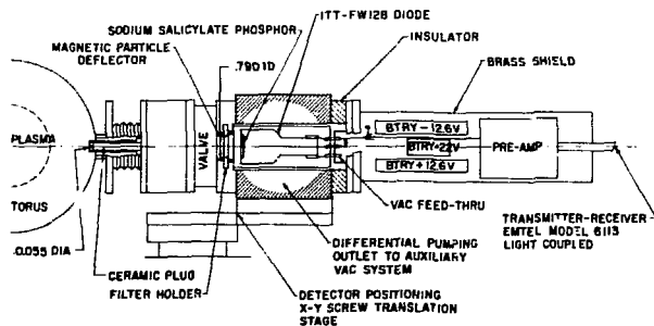
Fig. II-1. Schematic of radiation detector.
