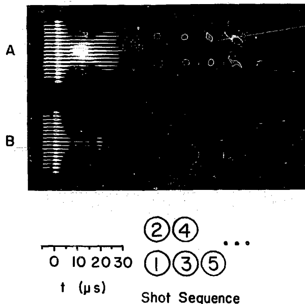
Fig. VI-10. Side-on-streak and end-on-framing pictures illustrating the difference between (a) the dirty mode, and (b) the clean mode. The time of the implosion corresponds to t=0 . The framing pictures were taken at 1.6- \mu s intervals with first frame at t=2 \mu s.
