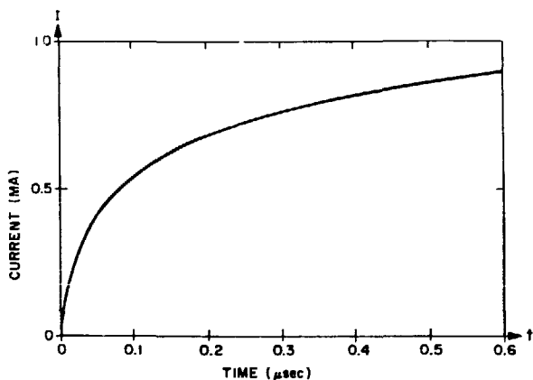
Fig. XVII-19. HDZP minimum current waveform.
