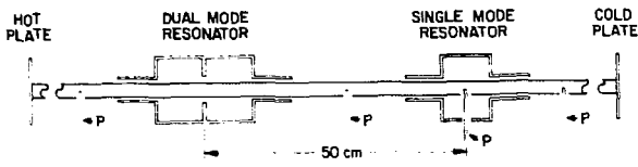
Fig. X-1. Experimental setup of Q-machine experiments.
