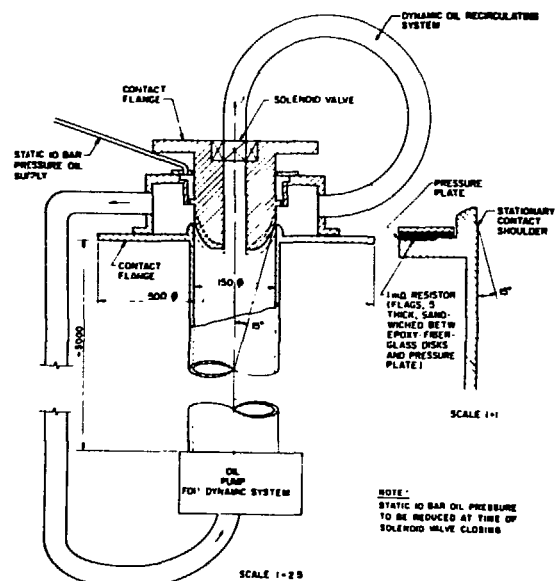
Fig. XV-1. Hydraulically actuated oil circuit breaker for 100-kA intermittent duty and approximately 2-kA, 500-V interrupting capacity.
