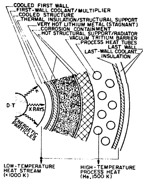
SIMPLE RADIATOR BLANKET
