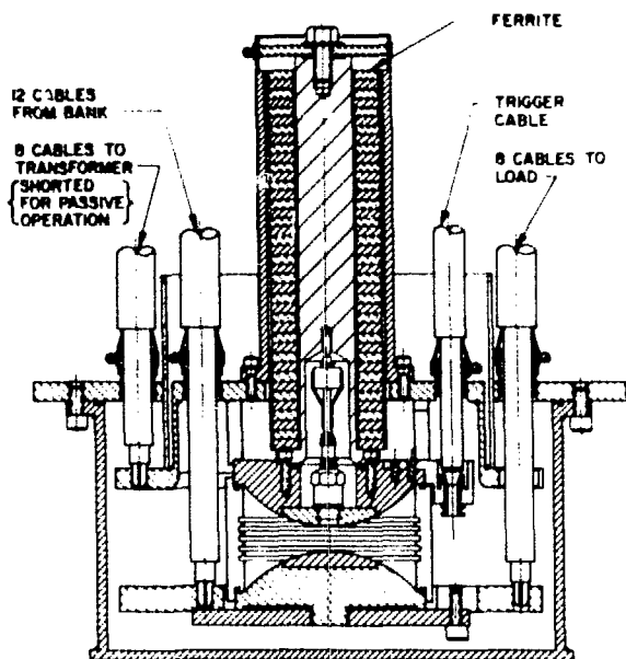
Fig. XVII-12. ZT-40 passive crowbar switch.
