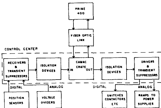
Figure XIV-1. Conceptual design of ZT-40 control system. Dotted line encloses electronics located immediately above power supply room.
