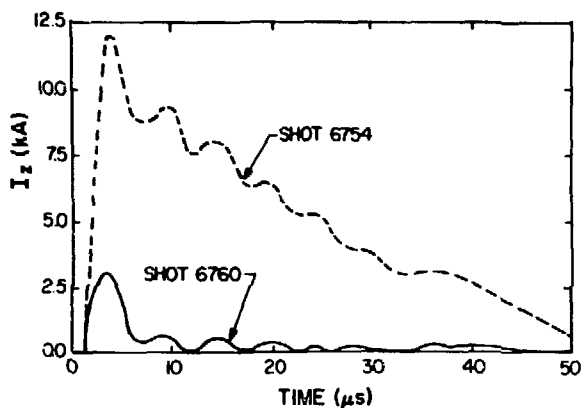
Fig. III-14. Axial current with and without cancellation circuit.
