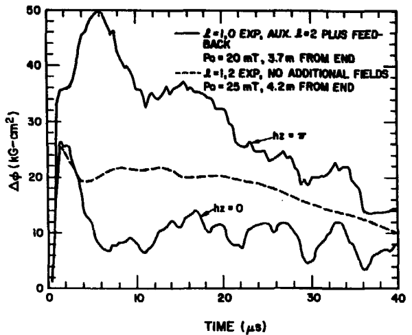
Fig. III-8. Excluded flux for \ell=1,2 compared with \ell=0,1 fields.
