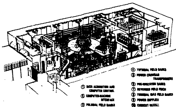
Fig. II-12. ZT-40 Facility.
