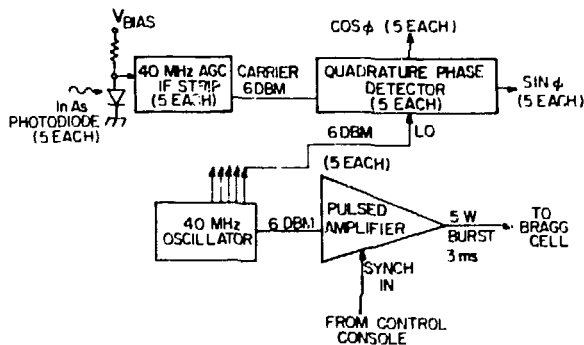
Fig. II-11. Block diagram of the interferometer electronics.
