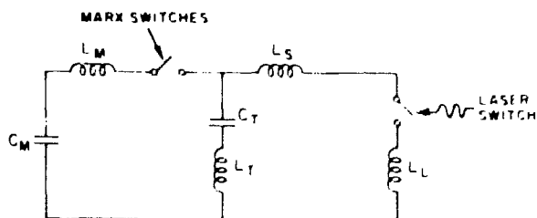
Fig. XVII-21. Basic HDZP circuit.
