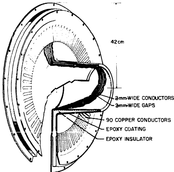
Fig. XVII-29. Radially fed implosion heating coil.
