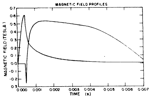
Fig. XVII-8. Representative Slow Mode I waveforms.
