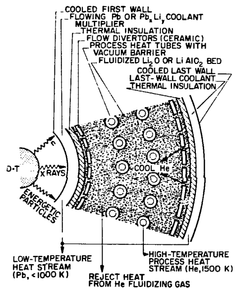
FLUIDIZED - BED BLANKET
