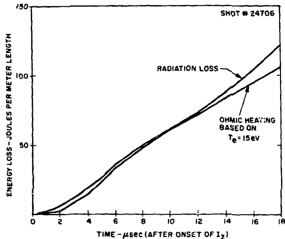
Fig. II-4. Curves comparing the measured radiation loss with the calculated ohmic input.
