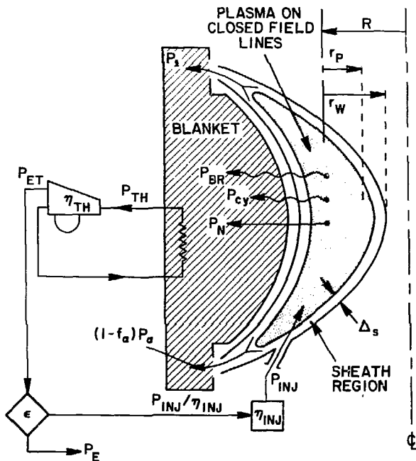
Fig. XVI-13. Schematic diagram of idealized, steady-state Tormac reactor energy balance.
