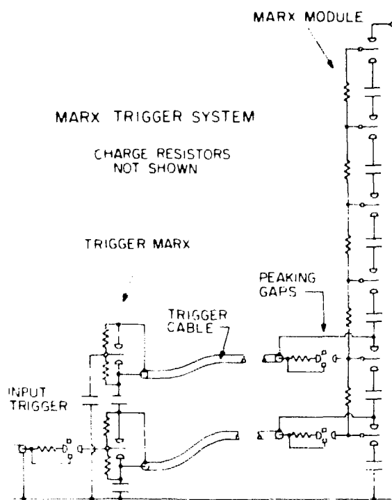
Fig. XVII-25. HDZP Marx trigger system.
