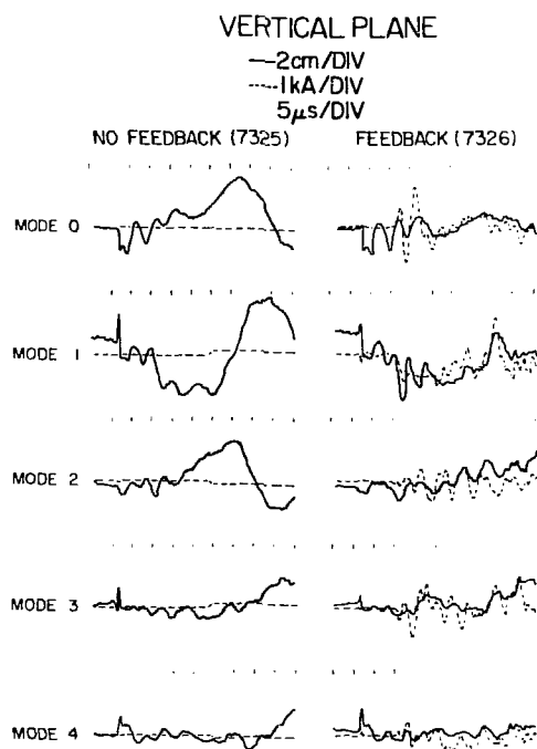
Fig. III-16. Vertical mode amplitudes controlled by feedback.
