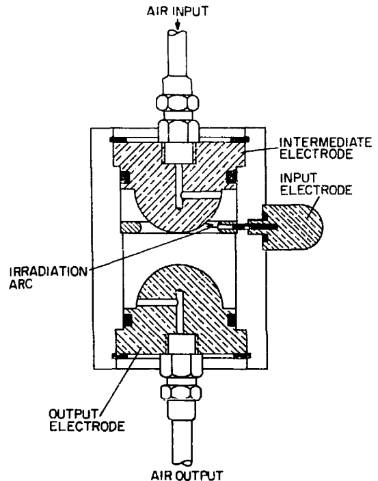
Fig. XVII-31. Inside-out trigatron peaking gap.
