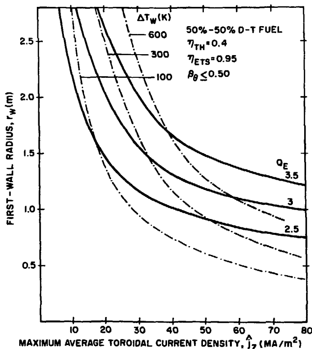
Fig. XVI-3. Dependence of first-wall radius on the average (maximum) toroidal current density for a fixed engineering Q -value (inverse of recirculating power fraction) for the Reversed-Field Pinch Reactor (RFPR-I). The dashed curves represent lines of constant first-wall surface temperature rise.
