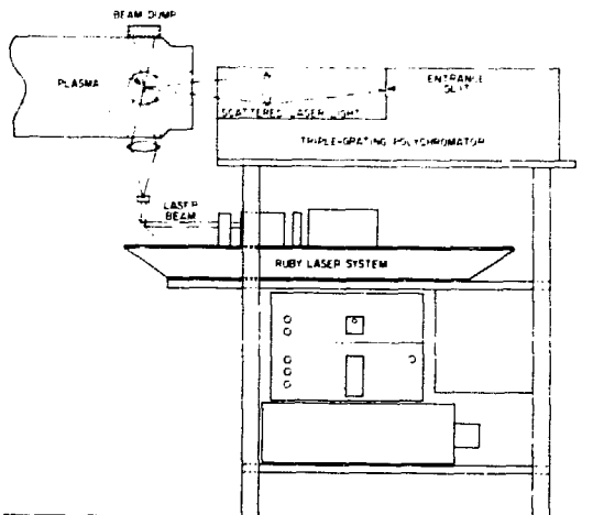
Fig. XII-7. Portable Thomson scattering set-up.
