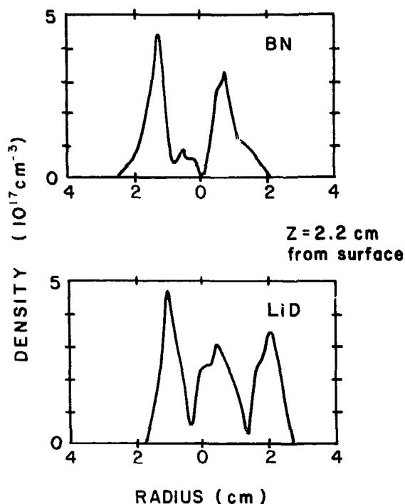
Fig. IV-22. Radial density profiles 2.2 centimeters from the plug surface.
