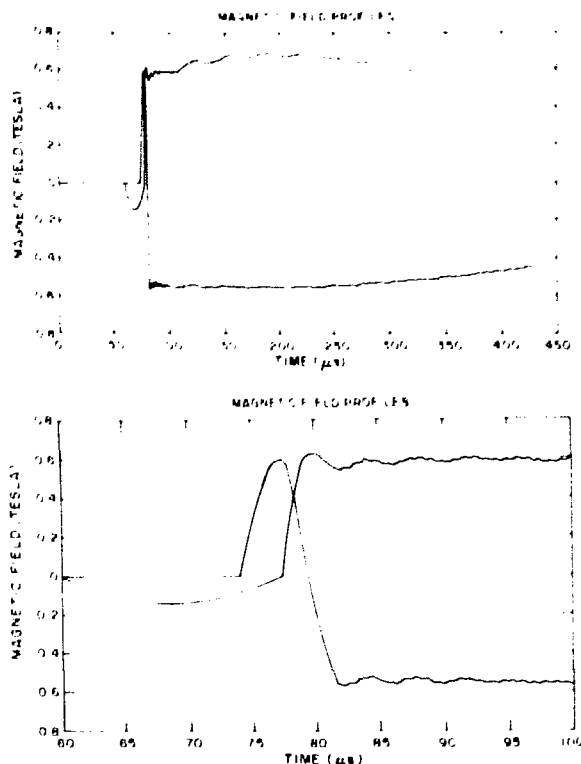
Fig. XVII-6. Representative Padua Mode waveforms.
