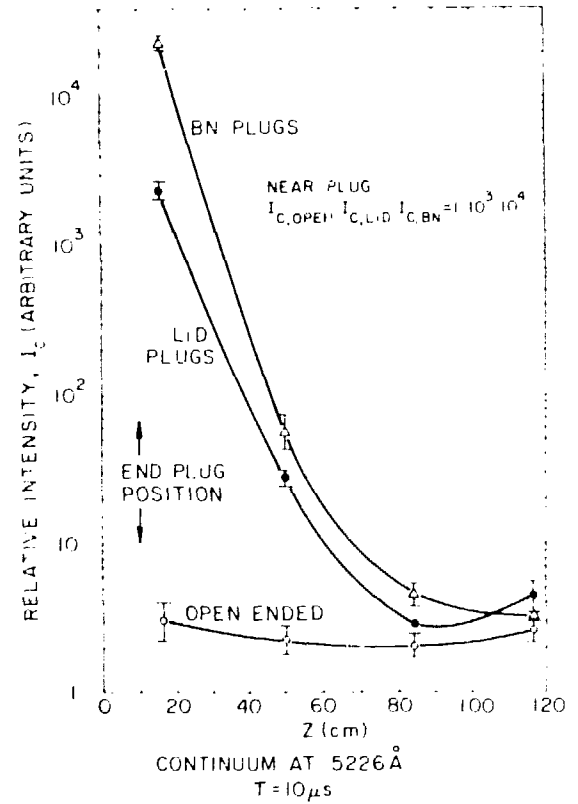
Fig. IV-20. Relative intensity of continuum radiation near the end of the compression coil at 10 \mu s after primary current initiation.
