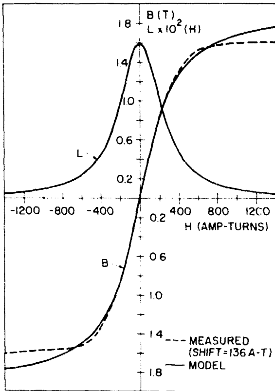
Fig. XVII-10. Transformer simulation flux model.
