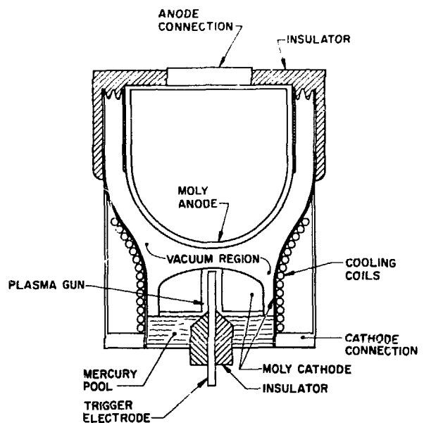
Fig. XVII-28. Conceptual mercury-wetted switch.
