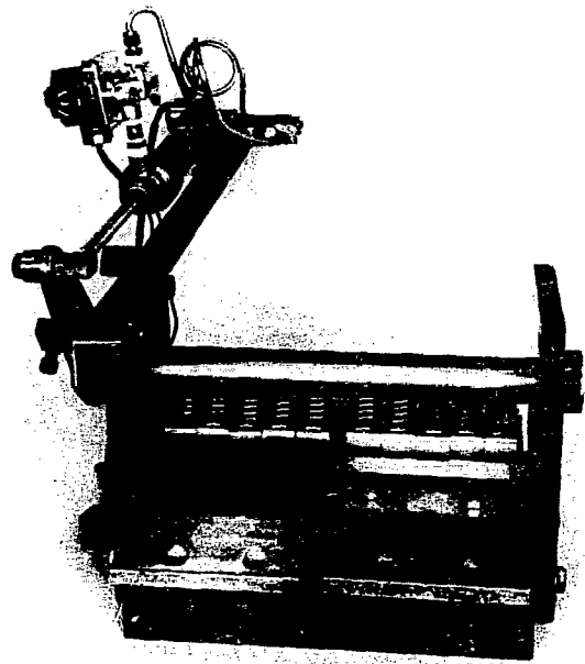
Fig. XV-6. High-current bypass component of the hybrid switch.
