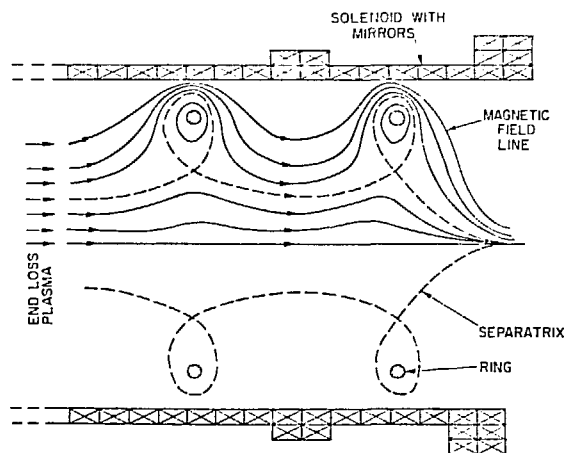
Figure XIII-2. Schematic of magnetic field geometry of IRES.
