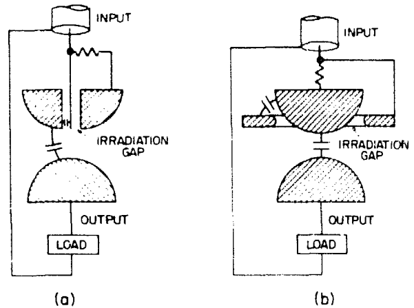
Fig. XVII-30. Peaking gap systems.
