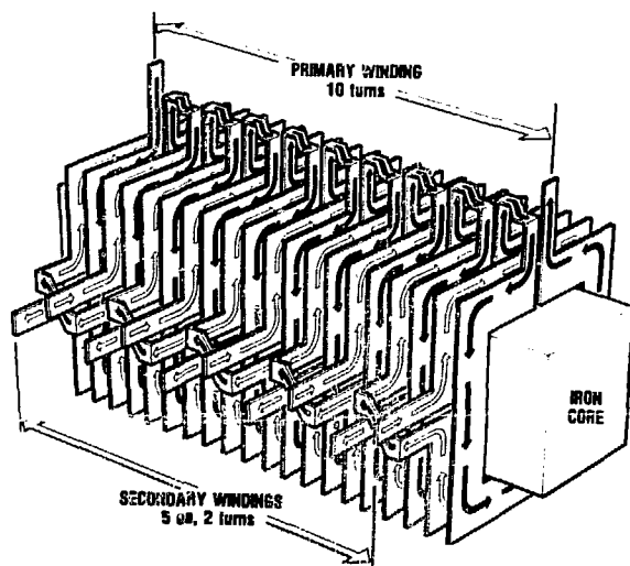
Fig. XVII-13. ZT-40 power crowbar transformer winding geometry.
