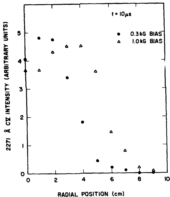
Fig. VI-13. Radial profiles of the C V 2271-A radiation.
