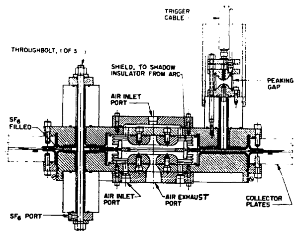
Fig. XVII-14. ZT-40 power crowbar switch.
