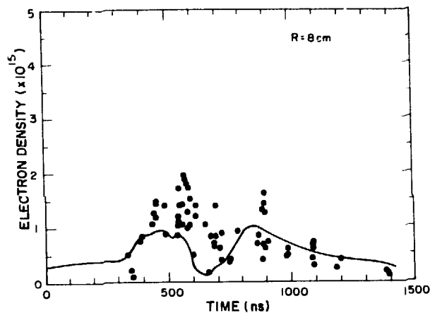
Fig. VII-1. Thomson scattering density measurements at R=8 cm. The solid curve is the interferometric density measurement at the same radius.
