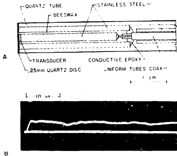
Fig. VI-8. Pressure probe (a) cross section, and (b) shock tube response.
