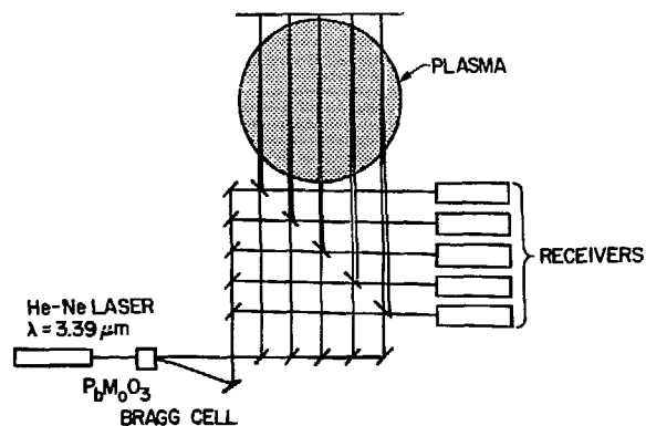
Fig. II-10. Schematic of the five-channel interferometer.
