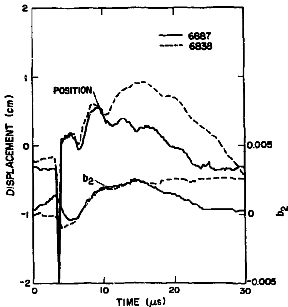
Fig. III-5. Position and trimming circuit waveforms.
