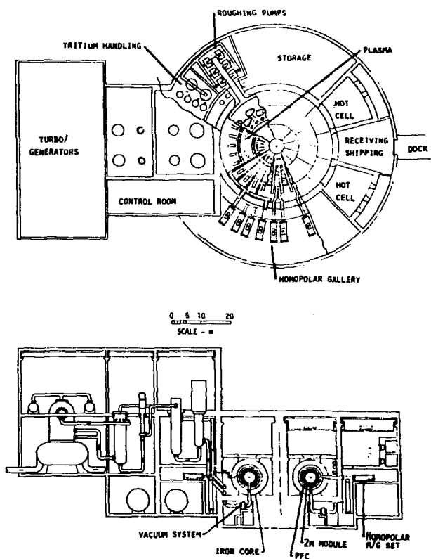
Fig. XVI-4. Plan and elevation views of a 750 MWe (net) Reversed-Field Pinch Reactor (RFPR-I).
