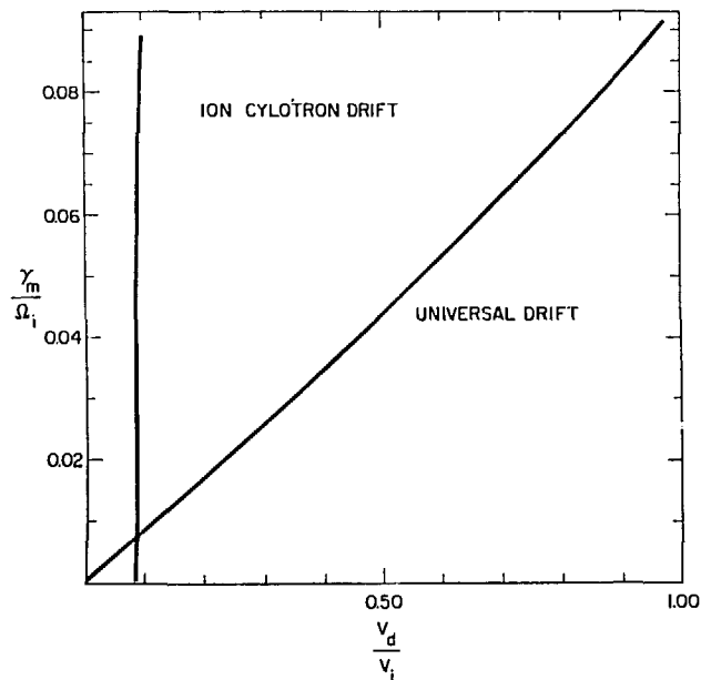
Figure XIII-1. The growth rate maximized over wavenumber, \gamma_m , of the universal and ion - cyclotron drift instabilities as a function density gradient drift speed v_d for T_e = T_i . Here \Omega_i = ion-cyclotron frequency and v_i = ion thermal speed.
