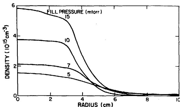
Fig. V-3. Radial plasma density profiles for different D_2 fill pressures.
