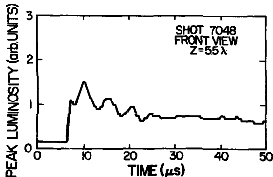
Fig. III-13. Position detector peak luminosity signal.
