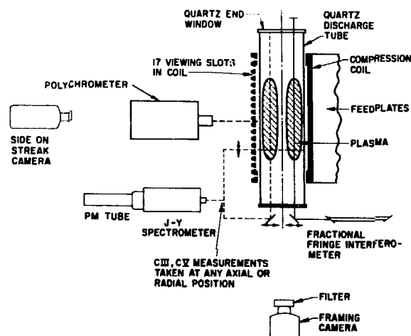
Fig. VI-2. Diagnostic arrangement on FRX-A.
