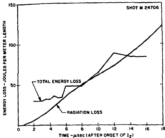
Fig. II-3. Curves comparing measured radiation loss with that deduced from energy balance shown in Fig. II-2.
