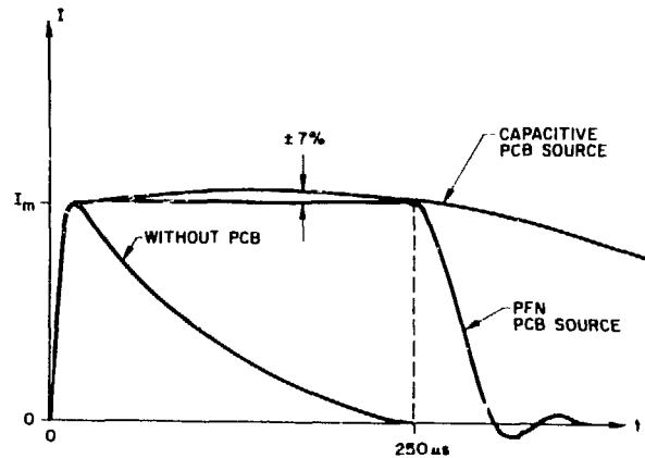
Fig. XVII-2. General ZT-40 current waveforms.
