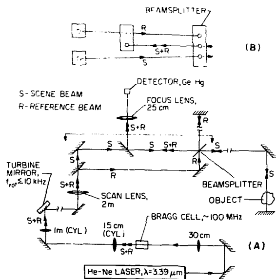
Fig. XII-1. System optical schematic.
