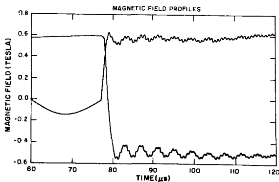
Fig. XVII-5. Representative Matched Mode waveforms.
