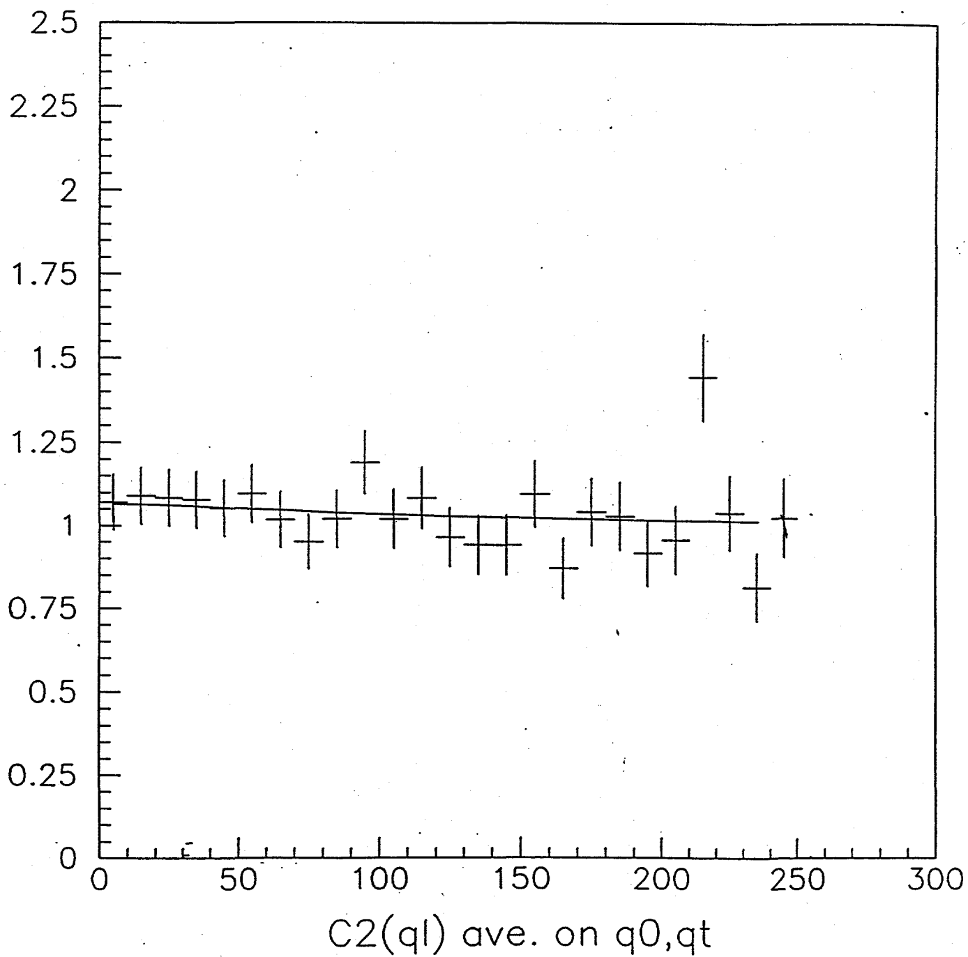
Figure 4: The projection of C_2(q) on the q_{||} axis.
