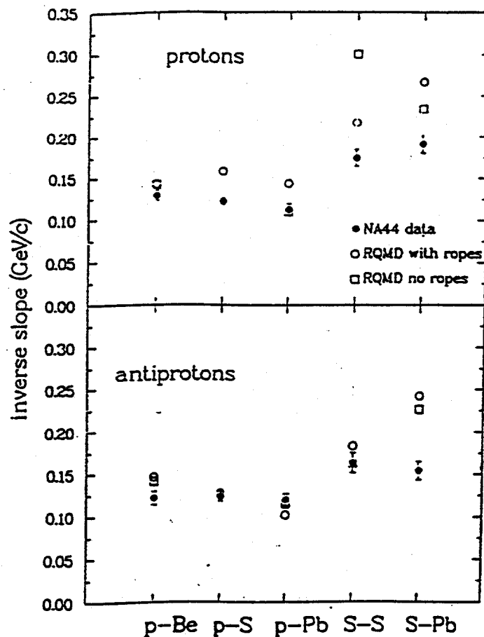
Figure 4 - The apparent temperature extracted from m_t spectra of protons and antiprotons near mid-rapidity for 450 proton and 200 A GeV sulfur reaction on various targets.
