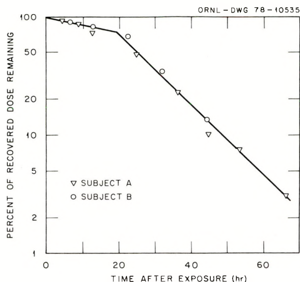
Figure D.6.5. Pentachlorophenol remaining in two human subjects after inhalation exposure. Source: Adapted from Casarett et al., 1969, Figure 4, p. 364. Reprinted by permission of the publisher.
