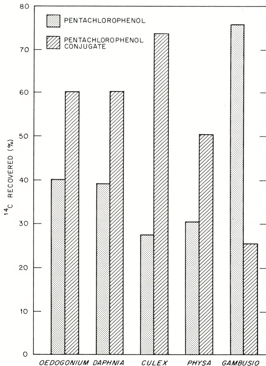
Figure D.5.6. Relative detoxification capacities of key organisms in a model aquatic ecosystem following treatment with radioactive pentachlorophenol. Source: Adapted from Lu and Metcalf, 1975, Figure 9, p. 279. Reprinted by permission of the publisher.
