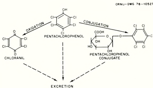
Figure D.6.12. Proposed metabolic pathway of pentachlorophenol in mammals. Source: Adapted from Tashiro et al., 1970, Figure 5, p. 129. Reprinted by permission of the publisher.
