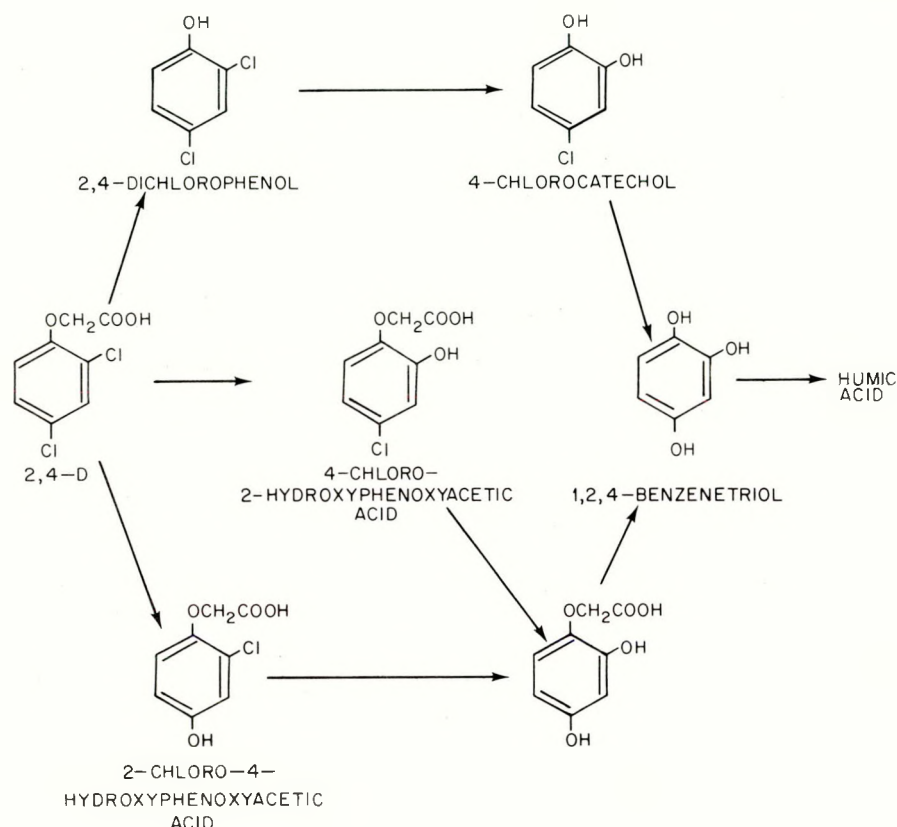
Figure B.7.4. Photolysis pathway for 2,4-D. Source: Adapted from Crosby and Tutass, 1966, Figure 3, p. 599. Reprinted by permission of the publisher.
