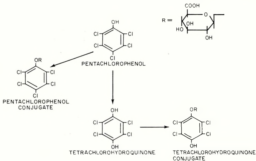
Figure D.6.13. Proposed metabolic pathway of pentachlorophenol in mice. Source: Adapted from Jakobson and Yllner, 1971, Figure 2, p. 522. Reprinted by permission of the publisher.
