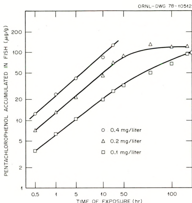
Figure D.5.2. Accumulation of pentachlorophenol in goldfish surviving in pentachlorophenol media (0.1, 0.2, and 0.4 mg/liter). Source: Adapted from Kobayashi and Akitake, 1975a, Figure 1, p. 89. Reprinted by permission of the publisher.
