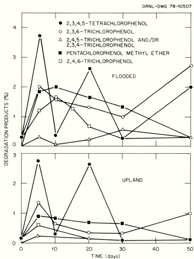
Figure C.7.4. Changes in amounts of pentachlorophenol degradation products during incubation under flooded and upland conditions. Source: Adapted from Kuwatsuka and Igarashi, 1975, Figure 4, p. 412.
