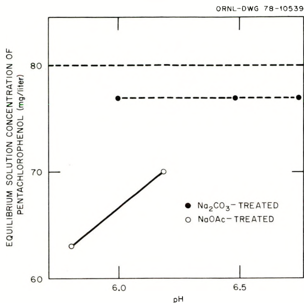
Figure D.2.1. Effect of pH on the adsorption of pentachlorophenol by isolated allophanes. Source: Adapted from Choi and Aomine, 1974 b , Figure 5, p. 377. Reprinted by permission of the publisher.
