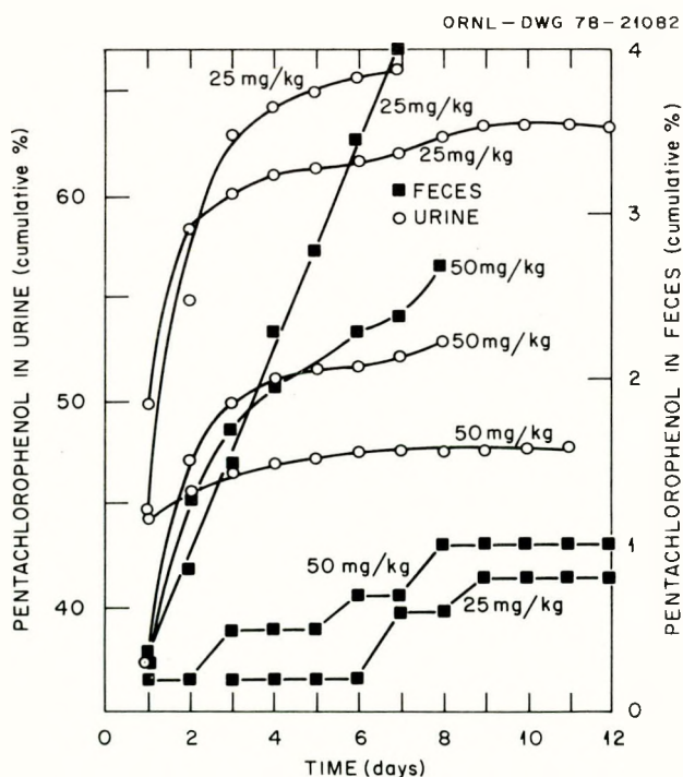
Figure D.6.11. Excretion of pentachlorophenol by rabbits after oral administration of sodium pentachlorophenate. Source: Compiled from Deichmann et al., 1942, Table 8, p. 114.
