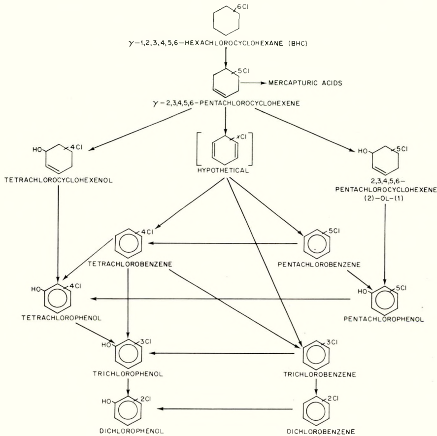
Figure A.8.2. Proposed metabolic pathway for lindane in rats. Source: Adapted from Engst et al., 1976, Figure 12, p. 113. Reprinted by courtesy of Marcel Dekker, Inc.
