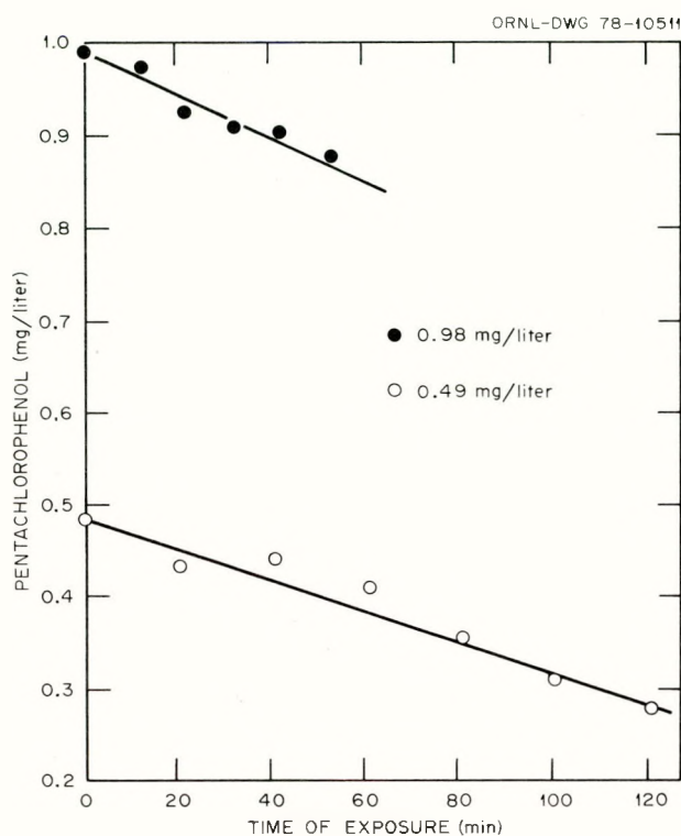
Figure D.5.1. Decrease of pentachlorophenol concentration in water during culture of rainbow trout. Source: Adapted from Tsuda and Kariya, 1963, Figure 1, p. 830. Reprinted by permission of the publisher.
