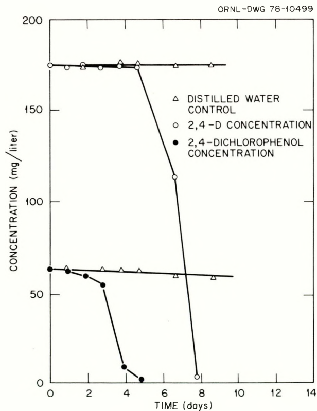
Figure B.7.1. Removal of 2,4-dichlorophenol and 2,4-D from solution in aeration basin effluent by continuous aeration. Source: Adapted from Sidwell, 1971, Figure 5, p. 67.
