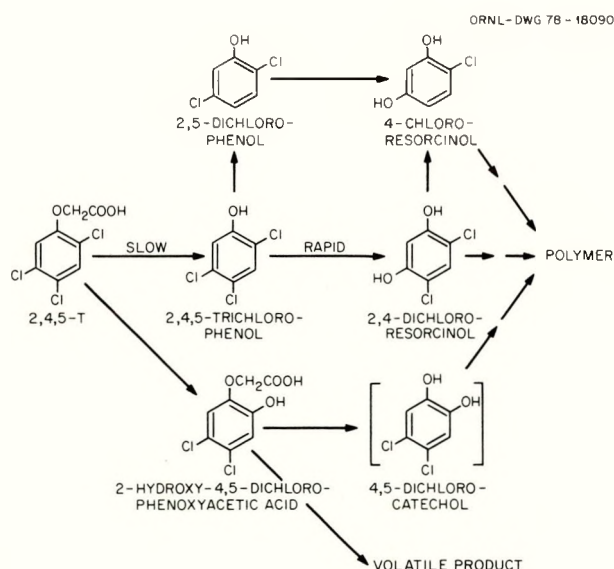
Figure C.7.5. Proposed photodecomposition pathway for 2,4,5-T in aqueous solution. Source: Adapted from Crosby and Wong, 1973, Figure 2, p. 1053. Reprinted by permission of the publisher.
