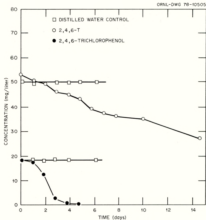
Figure C.7.2. Removal of 2,4,6-trichlorophenol and 2,4,6-T from solution in aeration basin effluent with continuous aeration. Source: Adapted from Sidwell, 1971, Figure 9, p. 71.
