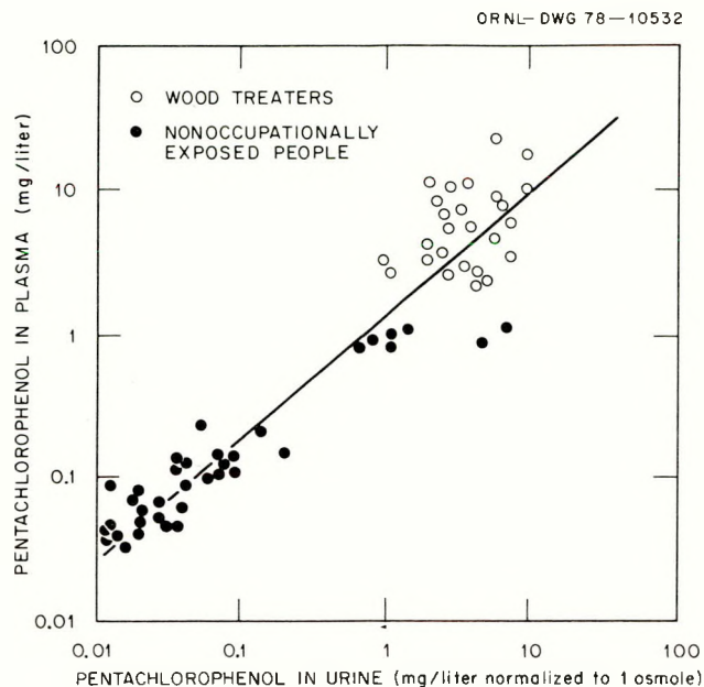
Figure D.6.2. Pentachlorophenol in paired blood and urine samples of wood treaters and nonoccupationally exposed people. Source: Adapted from Casarett et al., 1969, Figure 5, p. 364. Reprinted by permission of the publisher.
