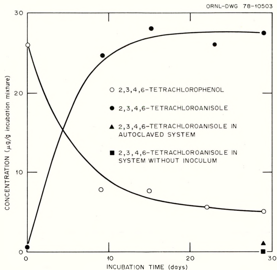
Figure C.5.1. Conversion of 2,3,4,6-tetrachlorophenol to 2,3,4,6-tetrachloroanisole in simulated broiler house litter. Source: Adapted from Curtis et al., 1972, Figure 1, p. 224. Reprinted by permission of the publisher.
