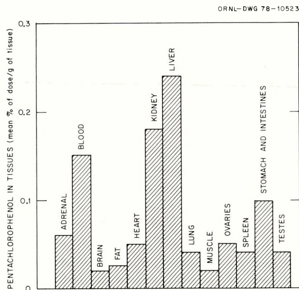
Figure D.6.7. Tissue distribution of [ ^{14}\text{C} ]pentachlorophenol and/or its labeled metabolites 40 hr after oral administration to rats. Source: Adapted from Larsen et al., 1972, Figure 2, p. 2005. Reprinted by permission of the publisher.
