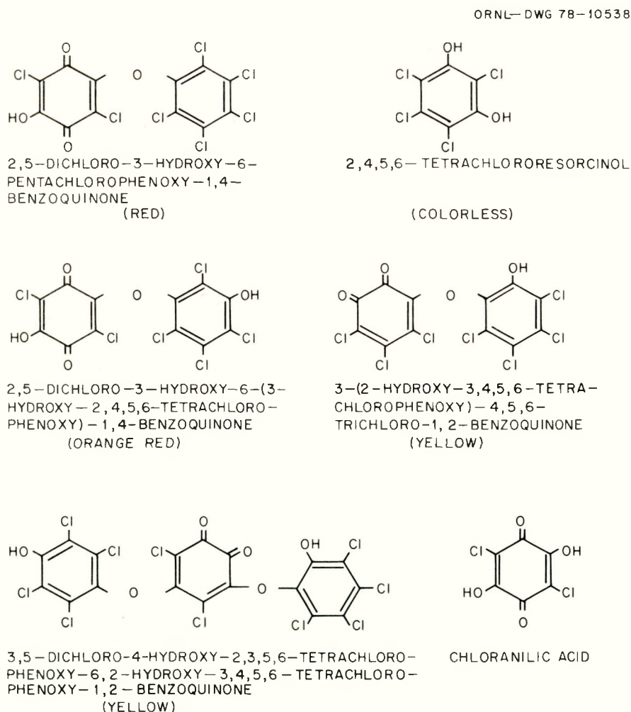
Figure D.7.1. Photochemical degradation products obtained from irradiation of an aqueous solution of sodium pentachlorophenate. Source: Adapted from Munakata and Kuwahara, 1969, Figure III, p. 17. Reprinted by permission of the publisher.
