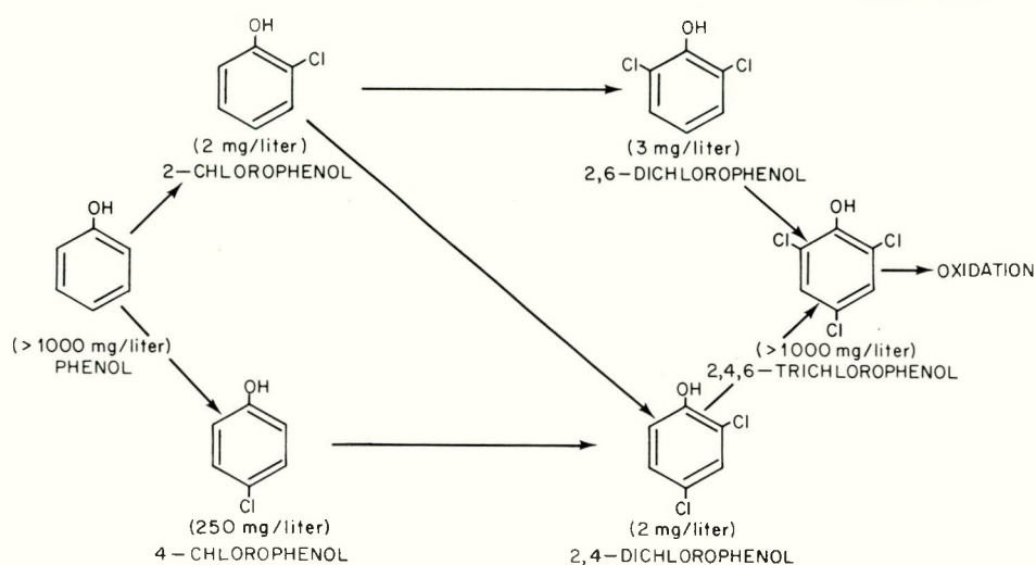
Figure C.7.6. Reaction scheme for the chlorination of phenol. Numbers in parentheses indicate odor threshold concentrations. Source: Adapted from Burttschell et al., 1959, Figure 3, p. 212. Reprinted with permission of the American Water Works Association from JOURNAL AWWA, Volume 51, copyrighted 1959.
