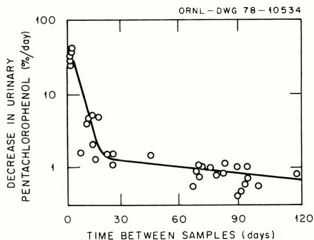
Figure D.6.15. Change in urinary pentachlorophenol with time for occupationally exposed people. Source: Adapted from Bevenue et al., 1967, Figure 2, p. 328. Reprinted by permission of the publisher.
