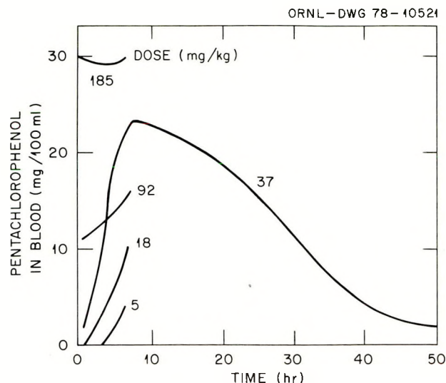
Figure D.6.3. Pentachlorophenol in blood of rabbits after a single oral dose of sodium pentachlorophenate. Source: Adapted from Deichmann et al., 1942, Figure 1, p. 110. Reprinted by permission of the publisher.
