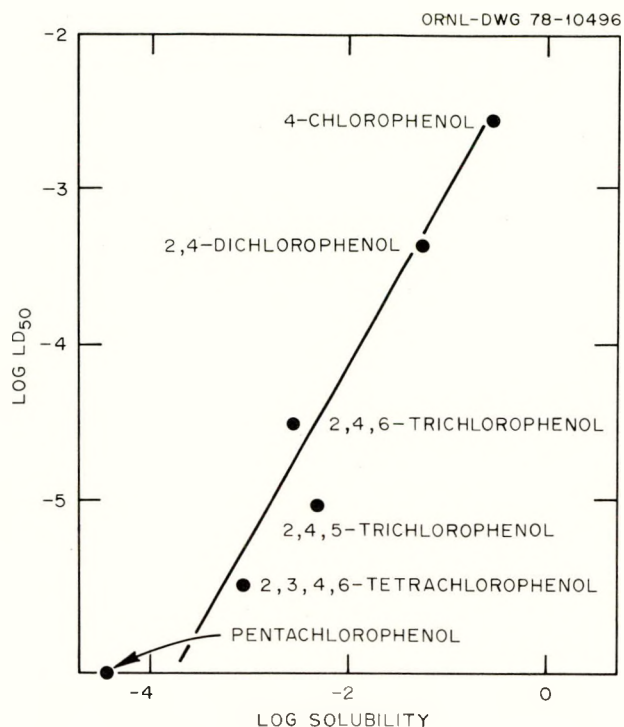
Figure A.4.1. Relationship between the logarithms of the solubilities of chlorophenols and the logarithms of the LD 50 in Lemna minor . Source: Adapted from Blackman, Parke, and Garton, 1955 b , Figure 2, p. 63. Reprinted by permission of the publisher.
