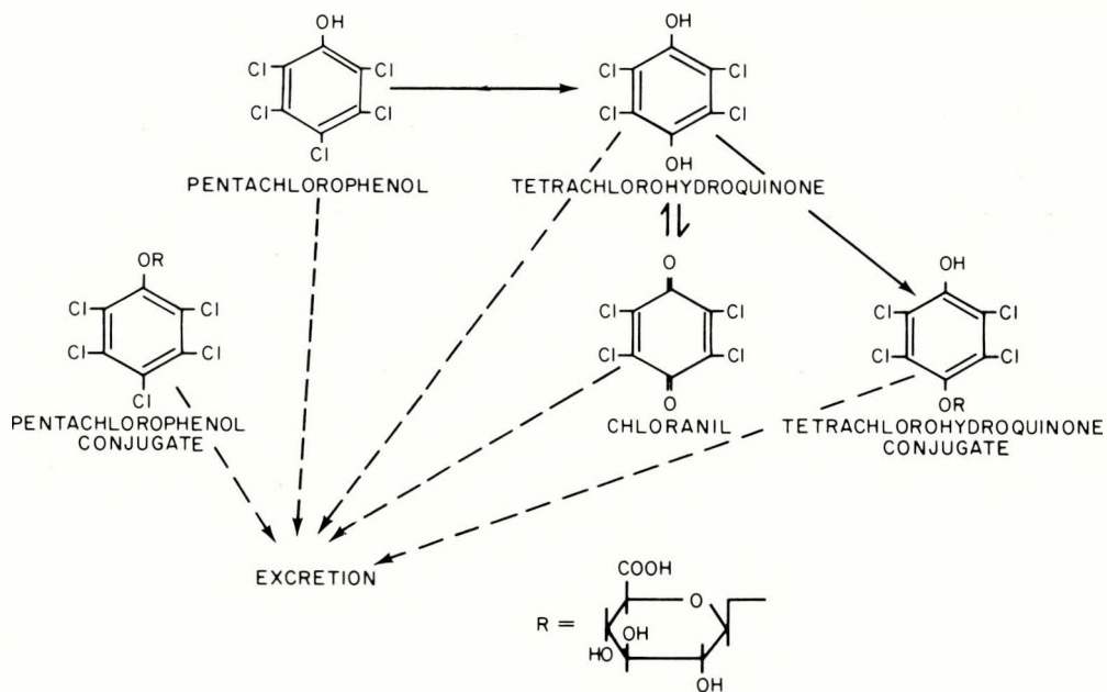
Figure D.6.14. Proposed integrated metabolic pathway of pentachlorophenol in mammals.
