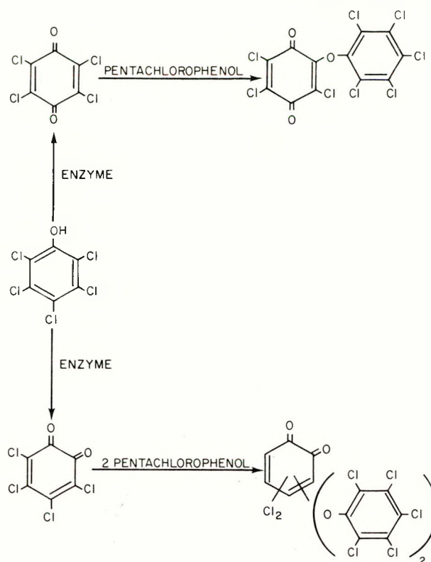
Figure D.3.1. Probable detoxification of pentachlorophenol by the laccase of Coriolus versicolor . Source: Adapted from Stranks, 1976, Figure 2, p. 14. Reproduced by permission of the Minister of Supply and Services Canada.
