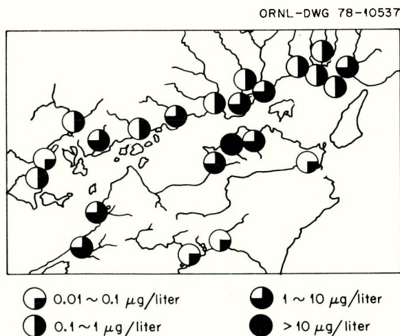
Figure D.6.20. Pentachlorophenol residues in river water in southwestern Japan during July 1969. Source: Adapted from Goto, 1971, Figure 2, p. 109.
