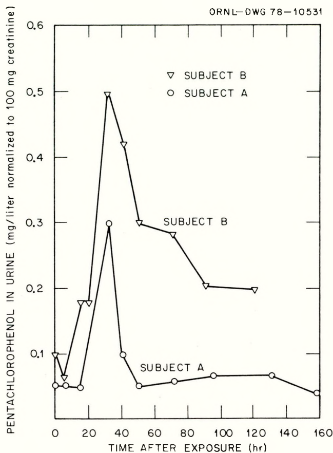
Figure D.6.1. Pentachlorophenol in urine of two subjects following respiratory exposure. Source: Adapted from Casarett et al., 1969, Figure 3, p. 363. Reprinted by permission of the publisher.
