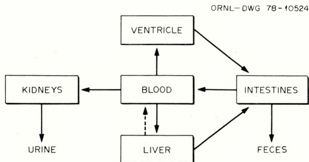
Figure D.6.8. Turnover of pentachlorophenol and/or its metabolites in the mouse. Source: Adapted from Jakobson and Yllner, 1971, Figure 4, p. 523. Reprinted by permission of the publisher.
