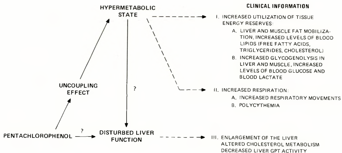
Figure D.5.10. Action of pentachlorophenol on eels in vivo. Source: Adapted from Larsson, 1973, Figure 3, p. 624. Reprinted by permission of the publisher.
