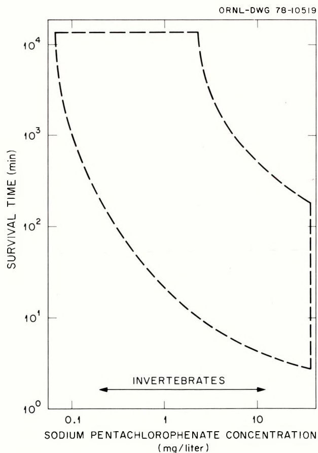
Figure D.5.9. Boundary of lethal area for a variety of fish species, relating lethal concentration of sodium pentachlorophenate to time of survival. The lethal concentrations for invertebrates are similar to those for fish. Source: Adapted from Norup, 1972, Figure 1, p. 1586. Reprinted by permission of the publisher.
