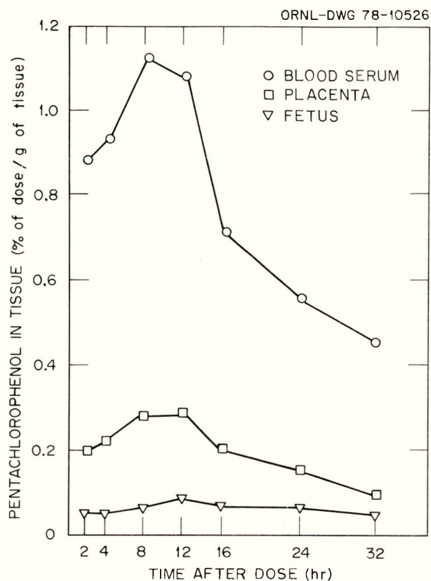
Figure D.6.10. [ ^{14}\text{C} ]Pentachlorophenol and/or its metabolites in tissues after an oral dose to pregnant rats on day 15 of gestation. Source: Adapted from Larsen et al., 1975, Figure 1, p. 125. Reprinted by courtesy of Marcel Dekker, Inc.
