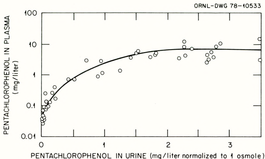
Figure D.6.6. Relationship between pentachlorophenol concentrations in plasma and urine. Source: Adapted from Casarett et al., 1969, Figure 6, p. 365. Reprinted by permission of the publisher.
