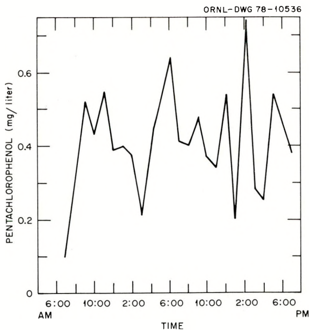
Figure D.6.19. Hourly concentrations of pentachlorophenol in the Willamette River on September 30, 1969. Source: Adapted from Buhler, Rasmusson, and Nakaue, 1973, Figure 2, p. 932. Reprinted by permission of the publisher.
