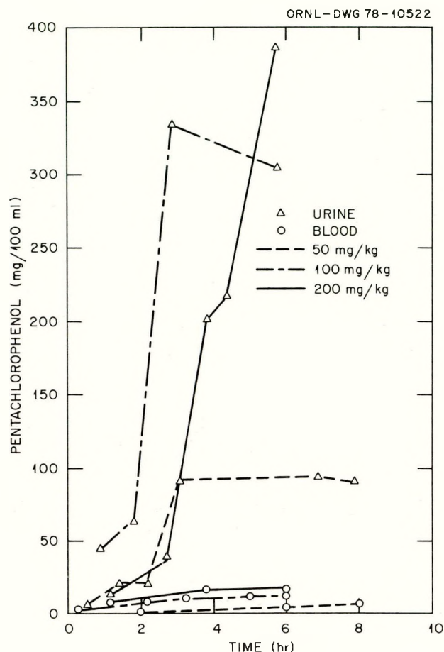
Figure D.6.4. Pentachlorophenol in blood and urine of rabbits exposed to a single oral dose. Source: Adapted from Machle, Deichmann, and Thomas, 1943, Figures 13, p. 193. Reprinted by permission of the publisher.
