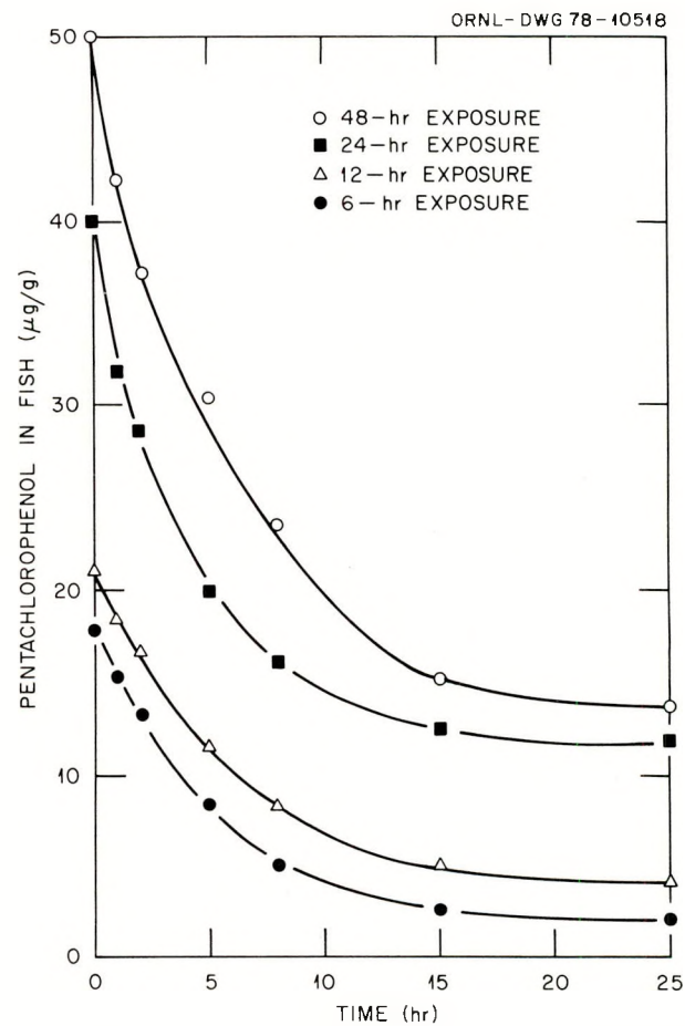
Figure D.5.8. Retention of pentachlorophenol in goldfish during culture in running water after various exposures (6 to 48 hr) to 0.2 mg/liter pentachlorophenol. Source: Adapted from Kobayashi and Akitake, 1975a, Figure 3, p. 90. Reprinted by permission of the publisher.
