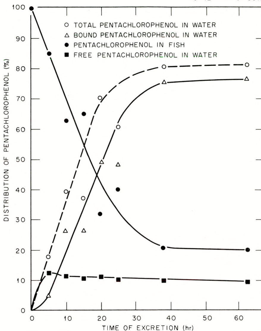
Figure D.5.5. Change in amounts of pentachlorophenol in goldfish and in free and bound pentachlorophenol in pentachlorophenol-free water. Source: Adapted from Akitake and Kobayashi, 1975, Figure 1, p. 324. Reprinted by permission of the publisher.
