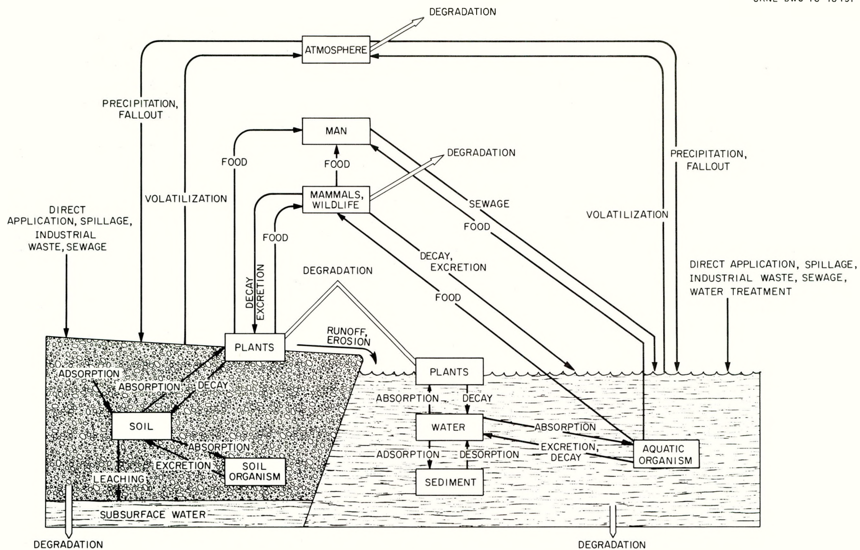
Figure A.8.1 Possible cycling of chlorophenols in the environment.
