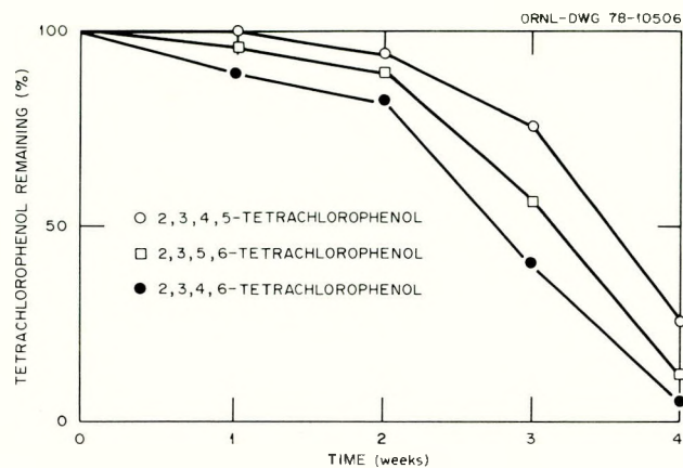
Figure C.7.3. Degradation of tetrachlorophenol isomers in paddy soil. Source: Adapted from Ide et al., 1972, Figure 7, p. 1943. Reprinted by permission of the publisher.
