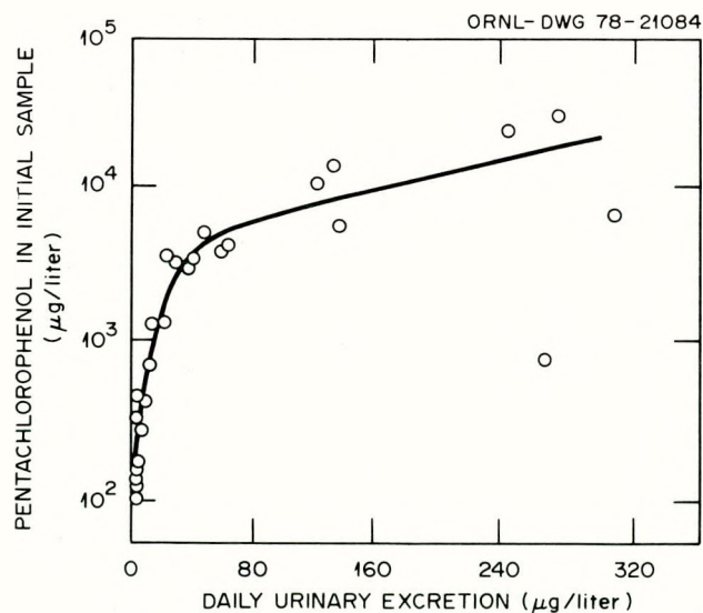
Figure D.6.17. Excretion of orally administered [ ^{14}\text{C} ]pentachlorophenol by rats. Source: Compiled from Larsen et al., 1972, Table I, p. 2004.
