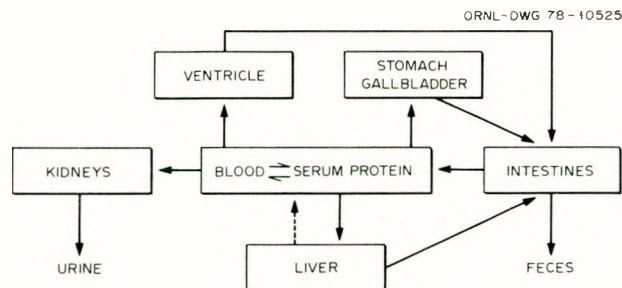
Figure D.6.9. Proposed turnover of pentachlorophenol and/or its metabolites in mammals.
