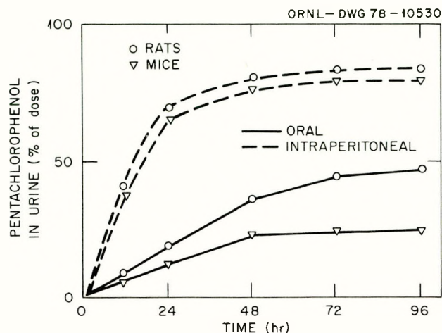
Figure D.6.18. Cumulative excretion of [ ^{14}\text{C} ]pentachlorophenol in the urine of rats and mice after a single oral or intraperitoneal dose. Source: Adapted from Ahlborg, Lindgren, and Mercier, 1974, Figure 1, p. 276. Reprinted by permission of the publisher.
