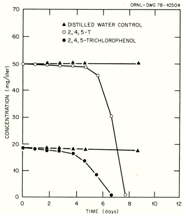
Figure C.7.1. Removal of 2,4,5-trichlorophenol and 2,4,5-T from solution in aeration basin effluent with continuous aeration. Source: Adapted from Sidwell, 1971, Figure 8, p. 70.
