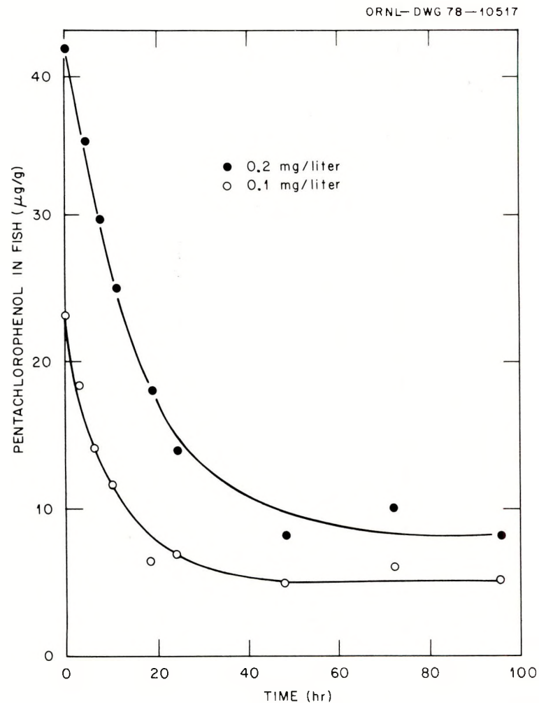
Figure D.5.7. Retention of pentachlorophenol in goldfish during culture in running water after a 24-hr exposure to pentachlorophenol media (0.1 and 0.2 mg/liter). Source: Adapted from Kobayashi and Akitake, 1975a, Figure 2, p. 90. Reprinted by permission of the publisher.
