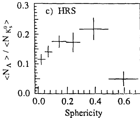
Fig. 14. (a) \Lambda multiplicity in 2 jet and 3 jet events as a function of the jet energy by TASSO. (b) Thrust distribution of events with a \Lambda and that in all events by MARK II. (c) The ratio of \Lambda multiplicity and K_S^0 multiplicity as a function of Sphericity by HRS. The solid lines in (a) are MC predictions for the \Lambda multiplicity in 3 jet events when the baryon multiplicity in gluon jets is f times larger than that in quark jets.
