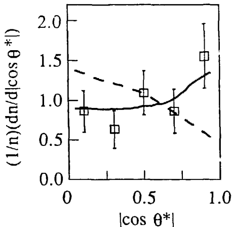
Fig. 12. Distribution of p-\bar{p} pairs in \theta^* with predictions of the LUND diquark model (solid line) and of the Webber MC (dashed line).
