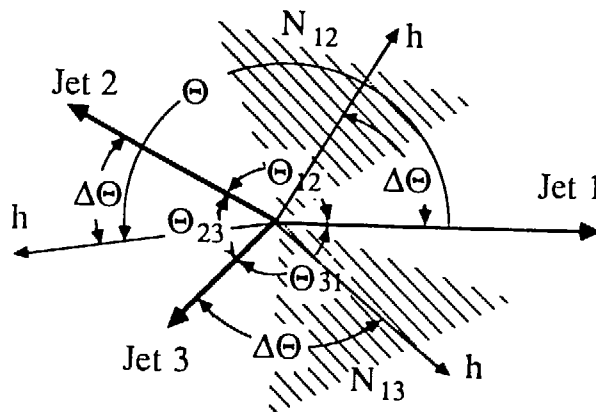
Fig. 16. Definitions of variables in the analysis of 3 jet events.
