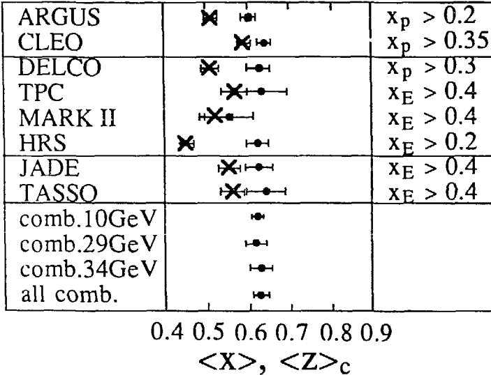
Fig. 6. Average value of the scaled momentum of D^* before ( \langle x \rangle , marked by crosses) and after ( \langle z \rangle , marked by circle) corrections mentioned in the text.
