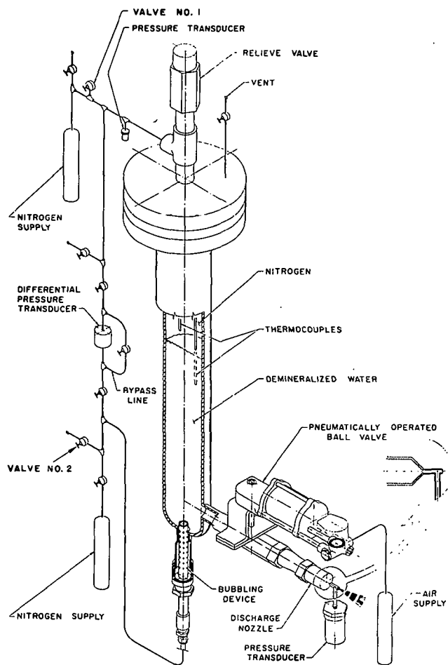
Fig. 1 Schematic of experimental apparatus
