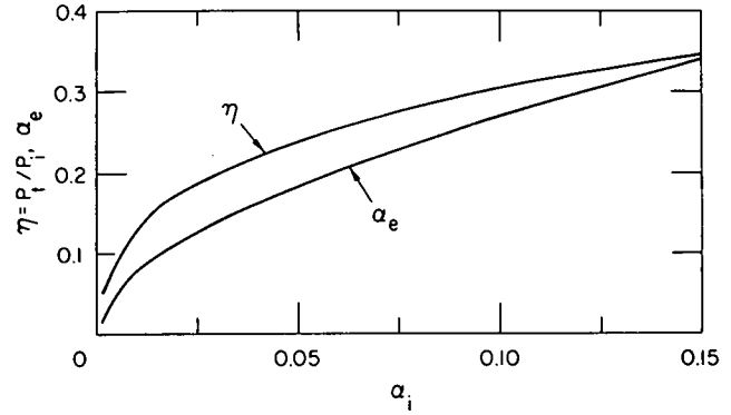
Fig.16 Variations of critical pressure ratio and exit void fraction with inlet (stagnation) void fraction in an equilibrium, homogeneous, steady, two-phase flow
