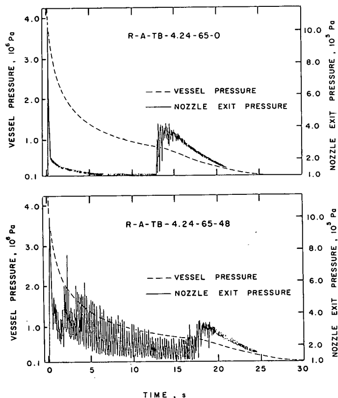
Fig.6 Measured vessel pressure and nozzle exit pressure versus time for tests conducted with discharge geometry A and with tube bundle inside the vessel
