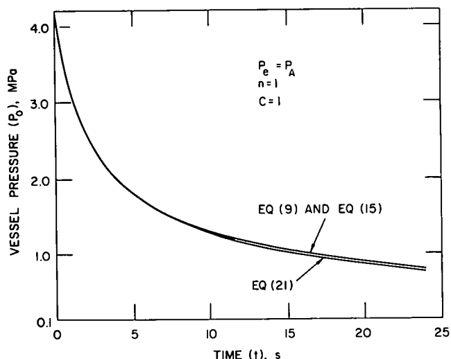
Fig.14 Comparison of the calculated variation of vessel pressure with time between employing the approximate solution provided by equation (21) and the more exact solution provided by equations (9) and (15)
