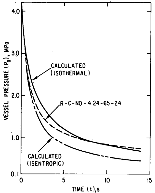
Fig.13 Comparison between calculated and measured vessel pressure versus time for test conducted with discharge geometry C, without tube bundle inside the vessel, and with 24 hour gas bubbling time
