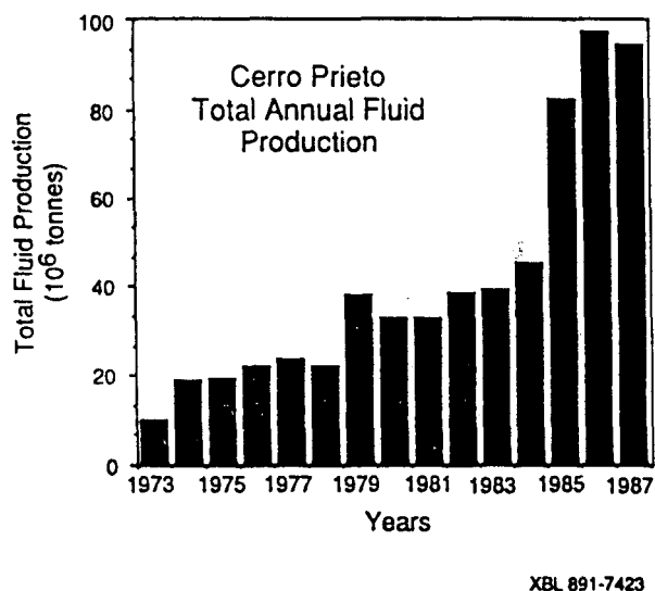
Figure 6. Total annual fluid production at Cerro Prieto.
