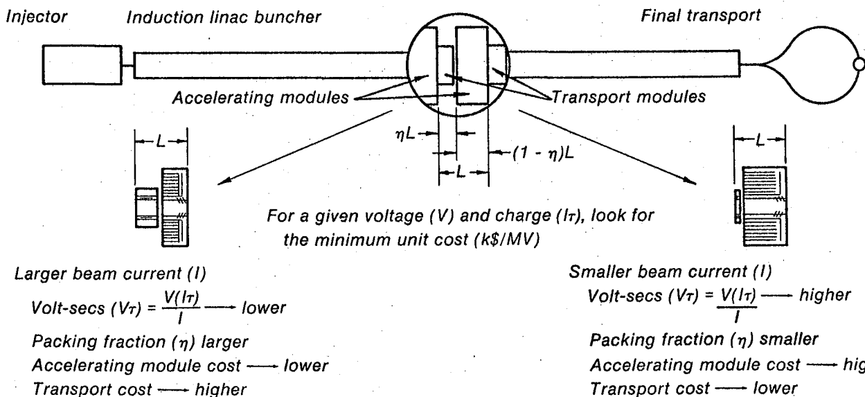
FIG. 1 - INDUCTION LINAC FUSION DRIVER
