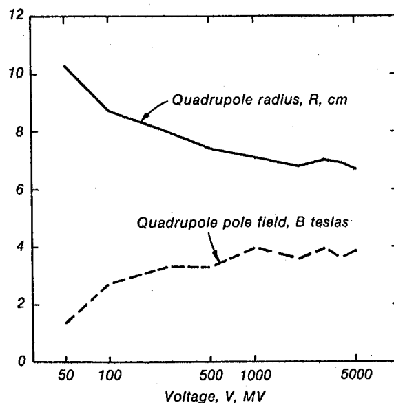
FIG. 6 - TRANSPORT MAGNET FIELD AND RADIUS
