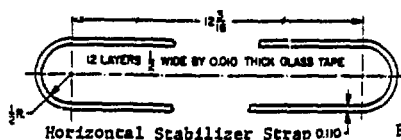
Horizontal Stabilizer Strap 0.010 Figure 3
