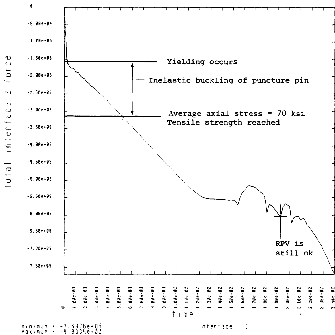
Fig. 3. Interface force between RPV and puncture pin (units are in in., lb, and s).
