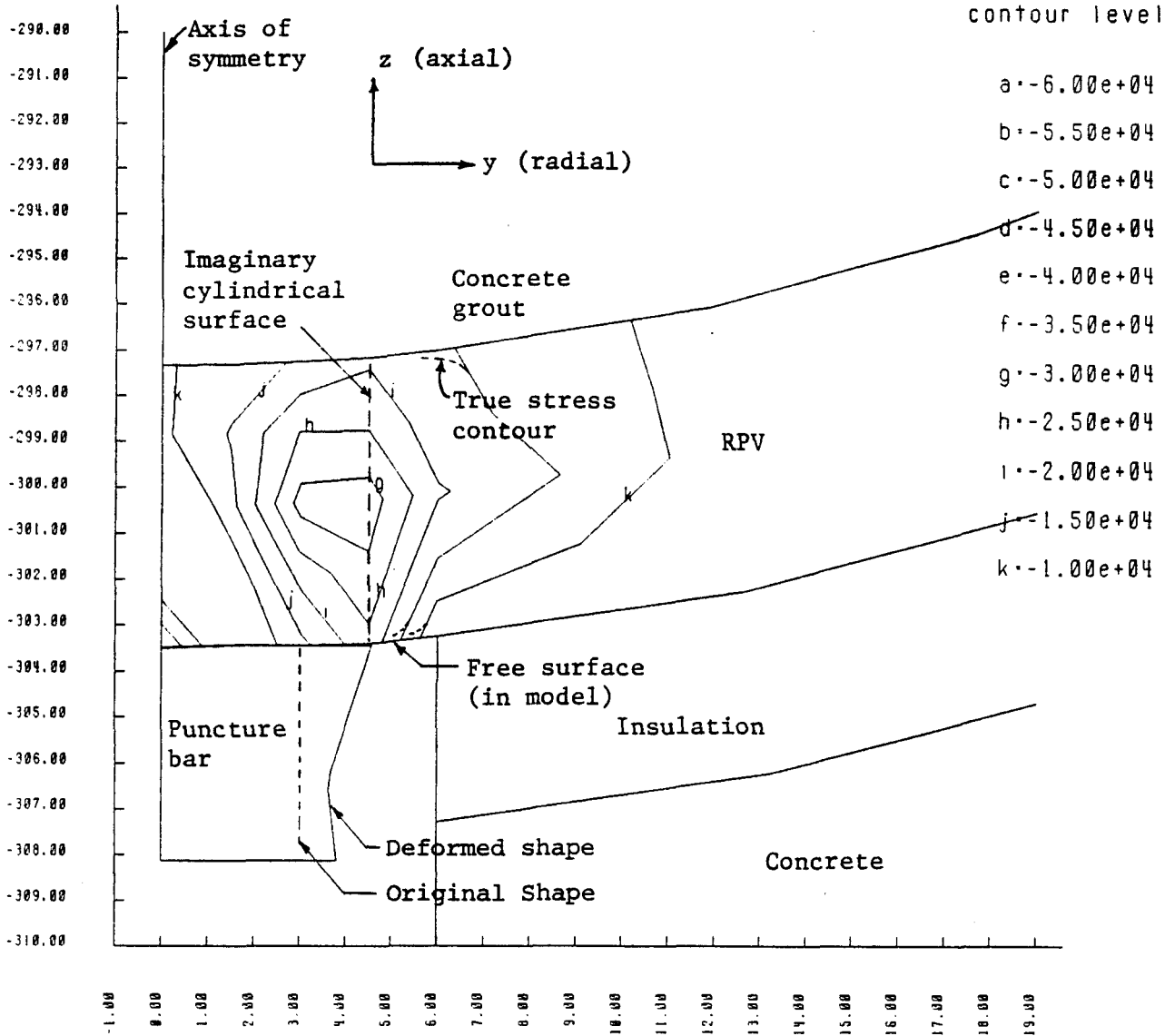
Fig. 2. Contours of y-z shear stress at time of 19 ms. (units are in in., lb, and s).
