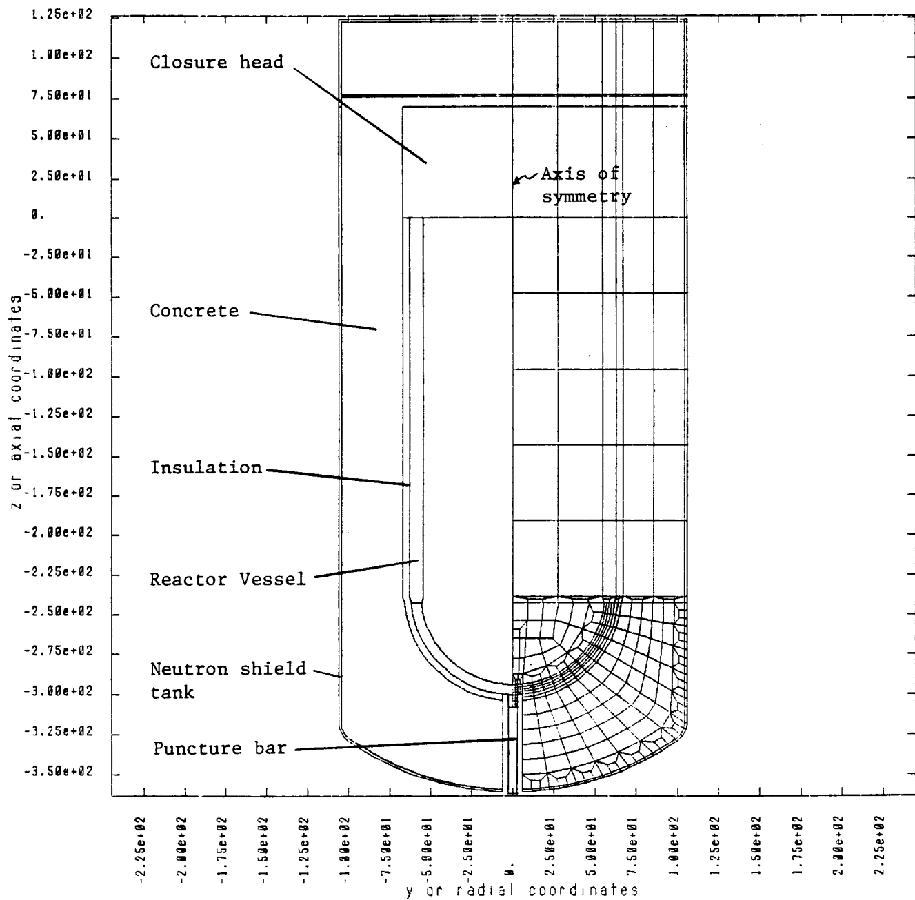
Fig. 1. Axisymmetric finite-element model of Shippingport RPV/NST package for puncture analysis.
