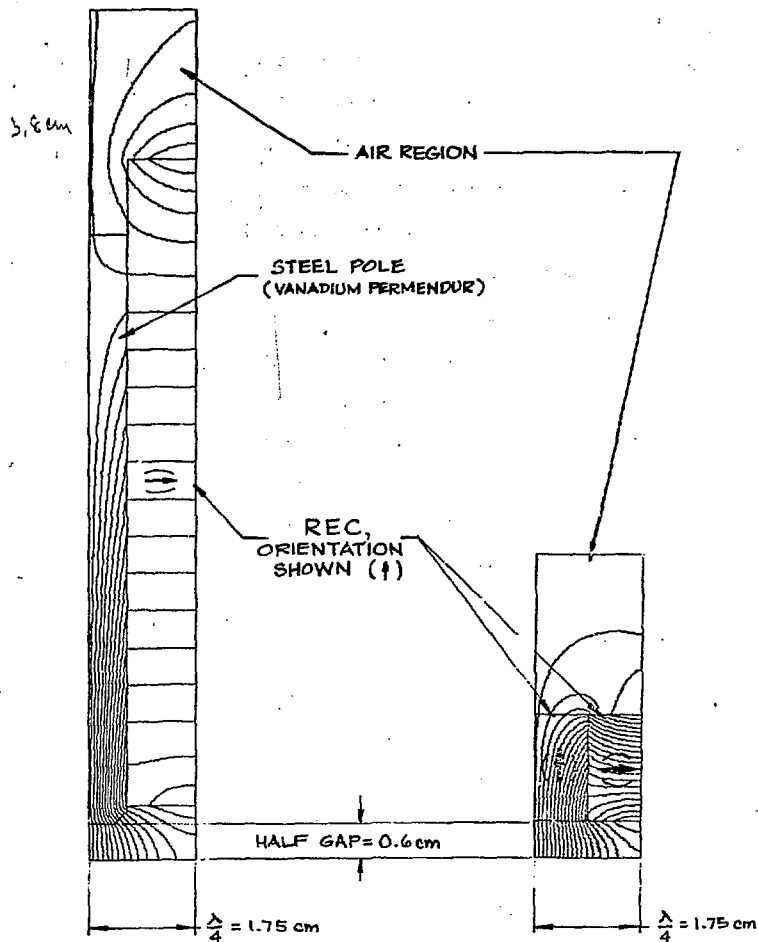
A) STEEL-REC HYBRID CONFIGURATION
