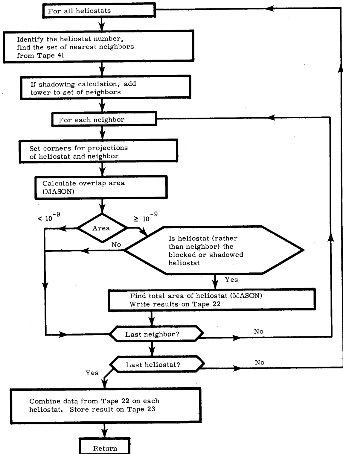
Figure A-5. Flow Diagram for OVER
