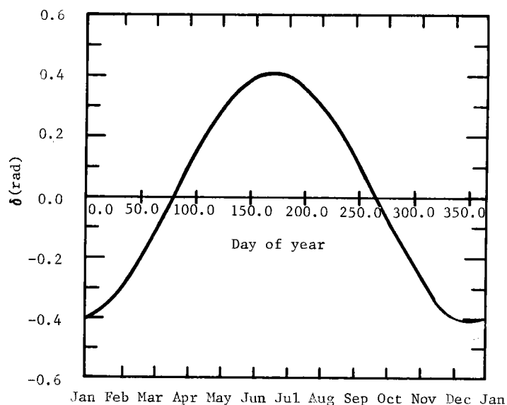
Figure A-3. Declination of the Sun
