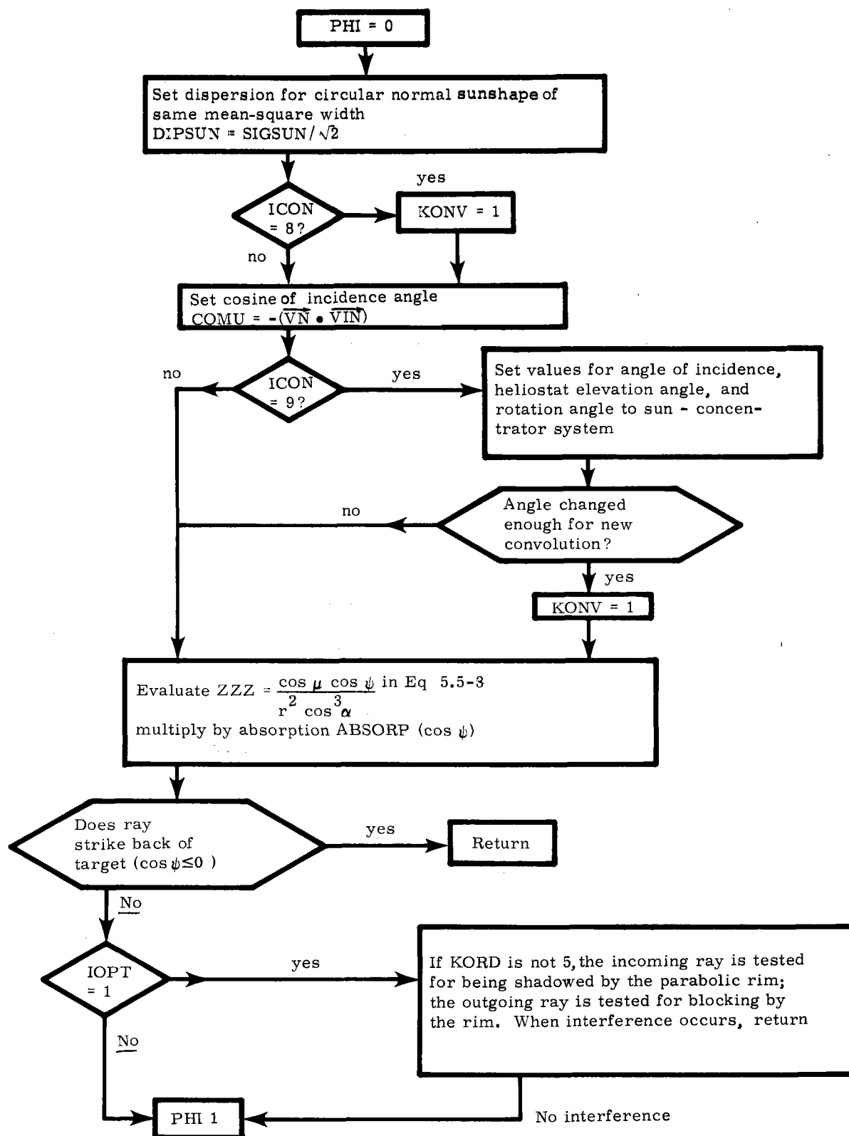
Figure A-6. Flow Chart for PHI
