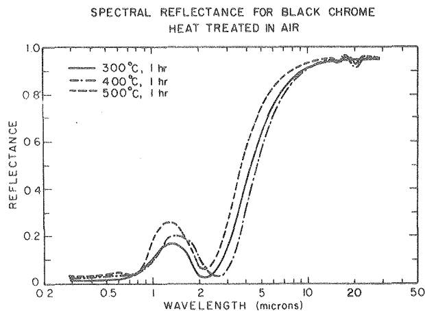
Figure 3. Spectral reflectance for black chrome heat treated in dry air over the 300-500°C range.
