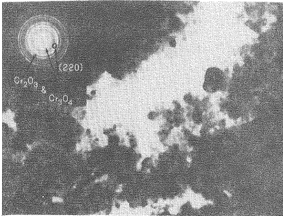
Figure 8. Morphology of black chrome after 1 hour heat treatment at 600°C, viewed by TEM at 100 kV.
