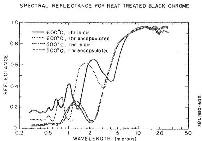
Figure 4. Spectral reflectance for both black chrome annealed in dry air and vacuum at 500, 600°C.
