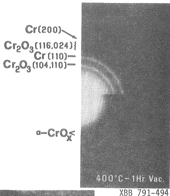
Figure 7. Typical diffraction pattern for 1 hour heat treatment
