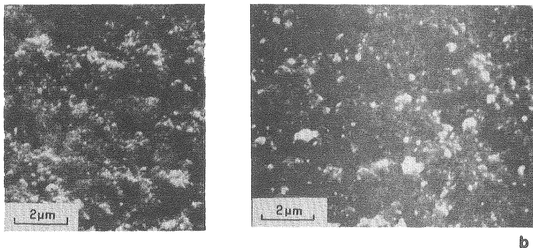
Figure 5. Black chrome examined by SEM at 20 kV, 20° tilt after 1 hour heat treatments. (a) typical surface structure for 27°-200°C heat treated samples. (b) surface structure for 600°C heat treatment, showing formation of bright white particles.
