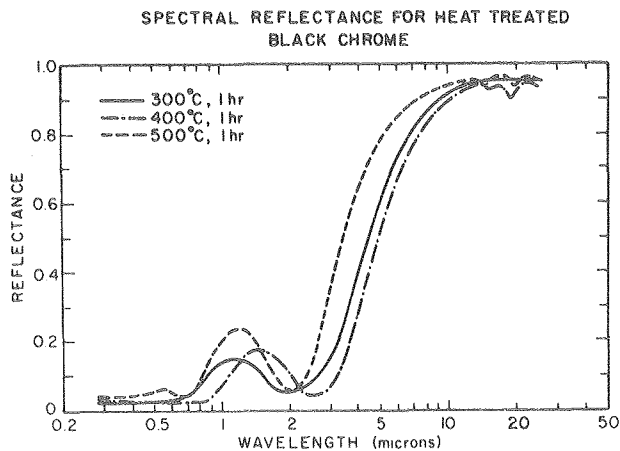
Figure 2. Spectral reflectance for black chrome heat treated in vacuum over the 300-500°C range.
