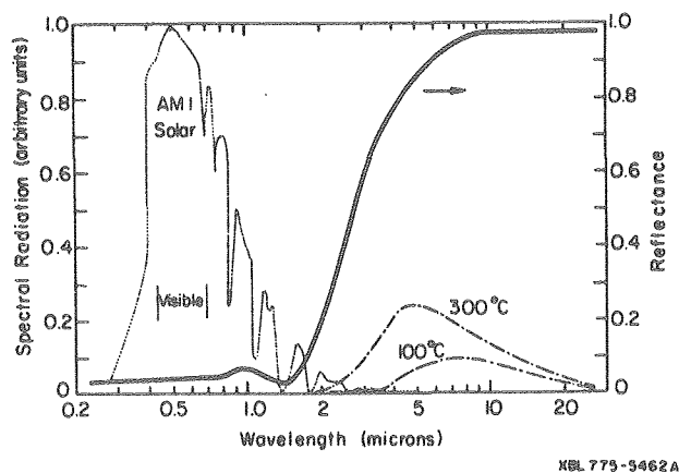
Figure 1. Wavelength correlation between black chrome spectral reflectance, the solar spectrum and black body spectrum (100°C, 300°C).
