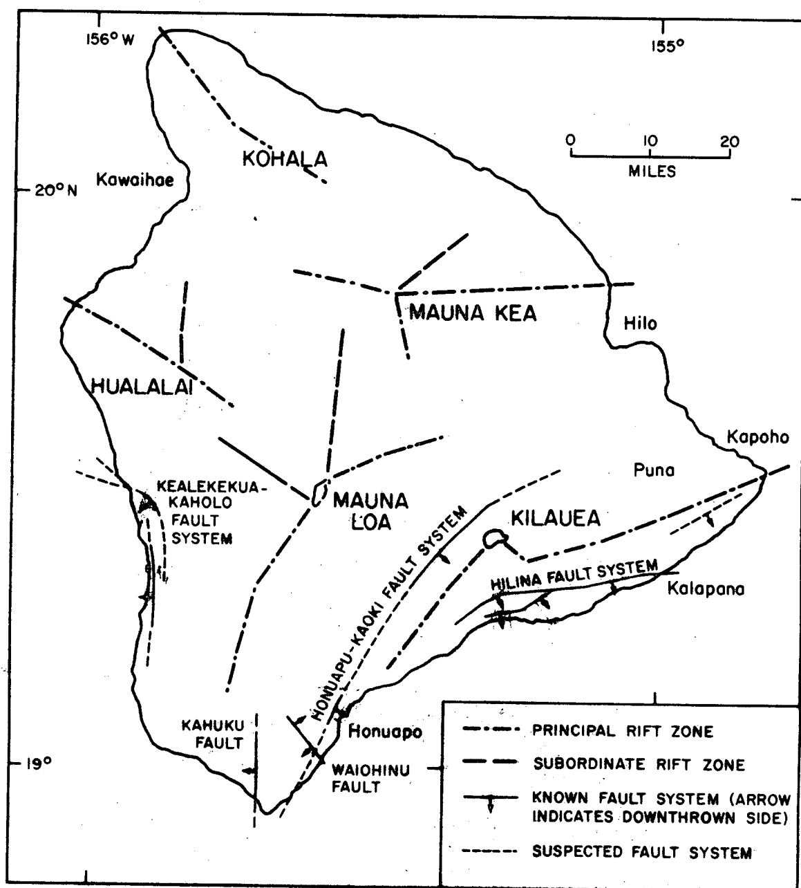
FIGURE 2. MAP OF THE ISLAND OF HAWAII SHOWING VOLCANOES AND ASSOCIATED RIFT ZONES
