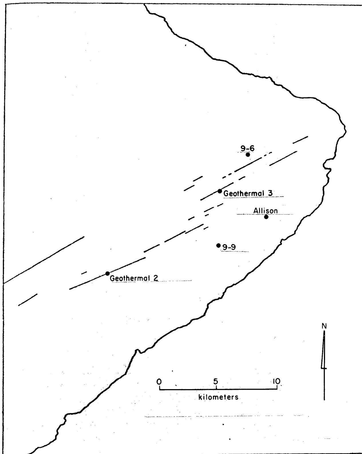
FIGURE 9. LOCATION OF WELLS, IN PUNA, ISLAND OF HAWAII
