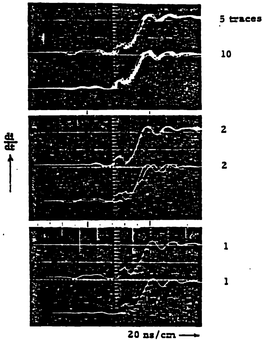
SPARK GAP JITTER MEASUREMENT FOR 80kV 27.6psig-air M_f = 1.75
