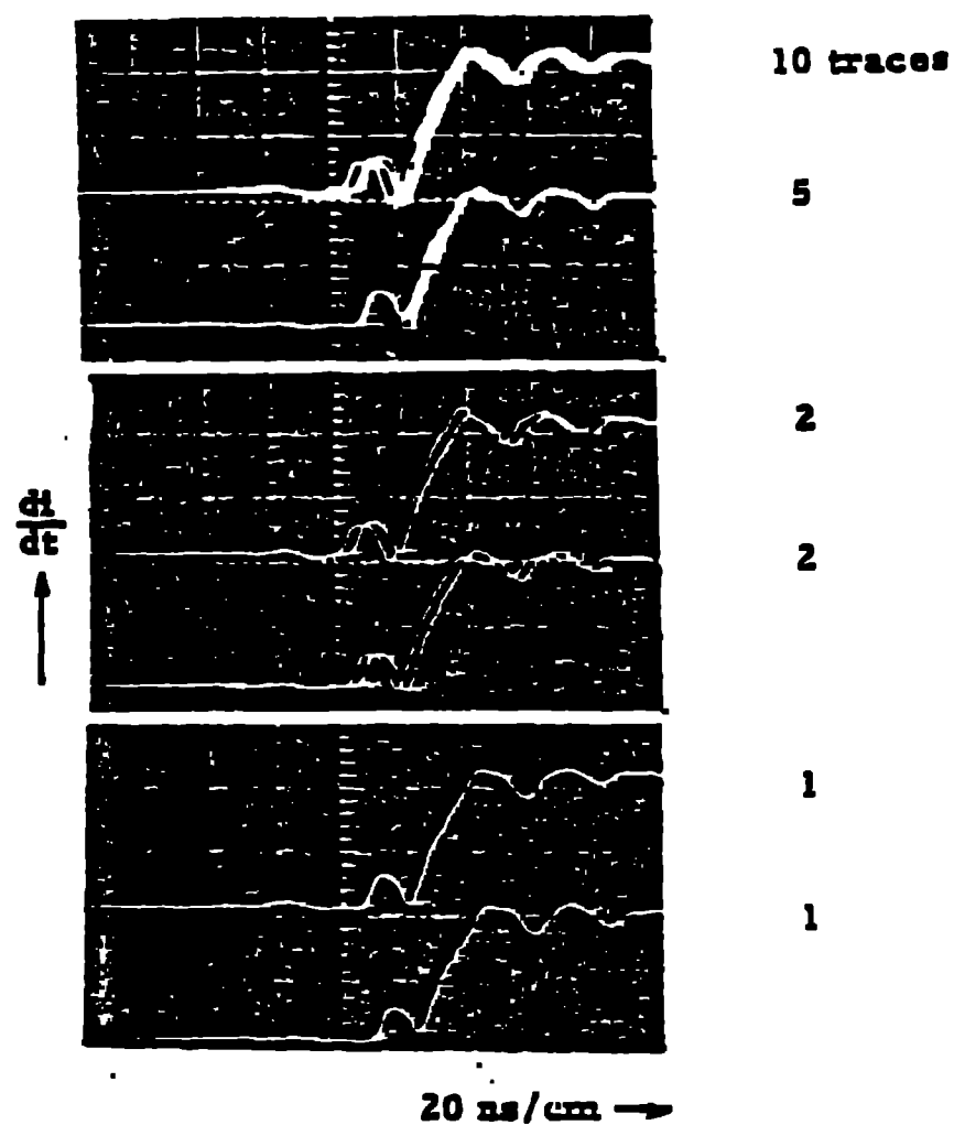
SPARK GAP JITTER MEASUREMENT FOR 120kV 60psig-air M_g = 2
