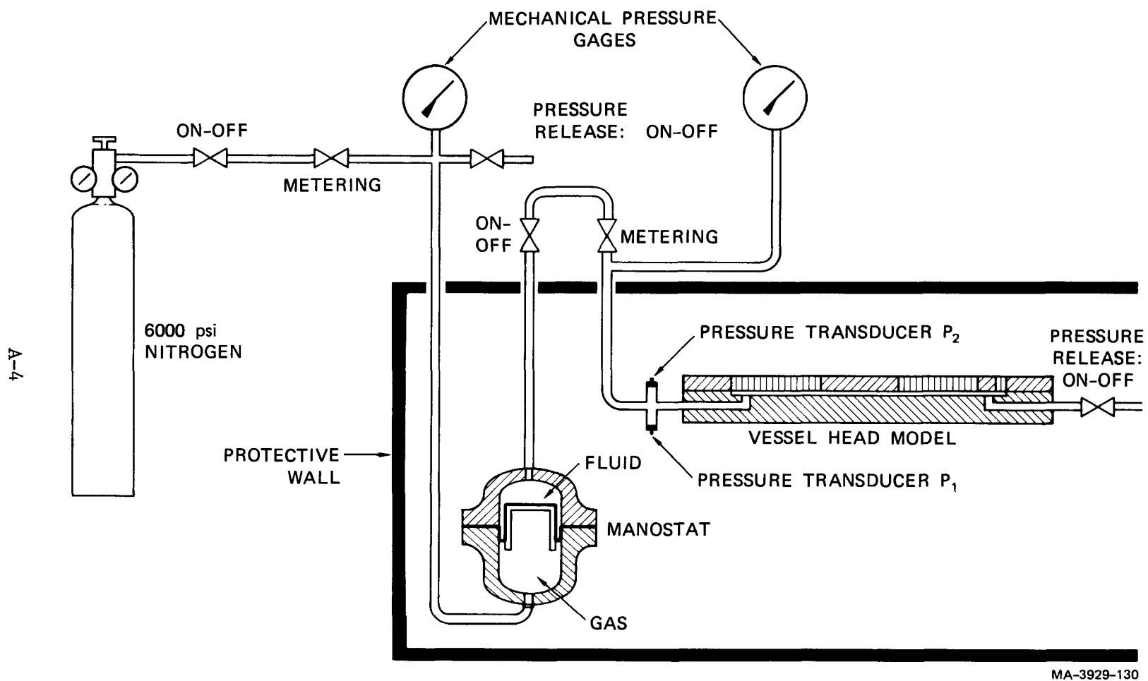
FIGURE A.2 STATIC TEST APPARATUS SCHEMATIC
