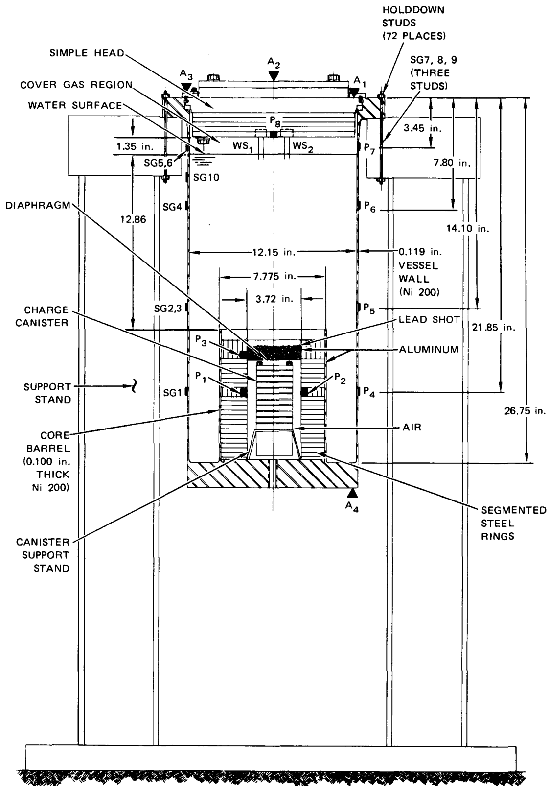
FIGURE 7 SM 2 WITH INSTRUMENTATION
