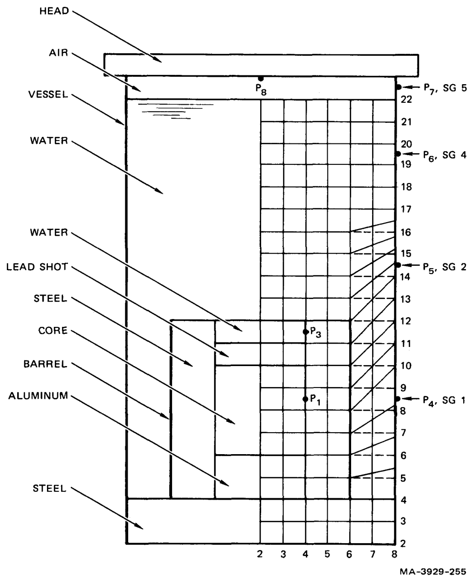
FIGURE 25 ZONE LAYOUT FOR SM 2 GE REXCO MODEL
