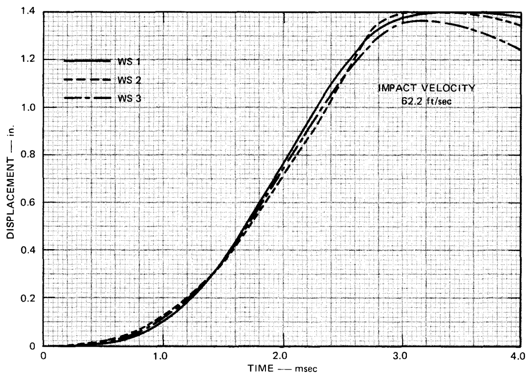
FIGURE D.28 WATER SURFACE DISPLACEMENT FOR SM 5
