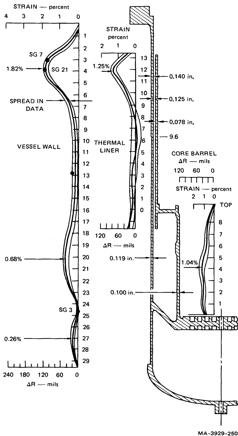
FIGURE D.29 DEFORMED SHAPE PROFILE FOR SM 5
