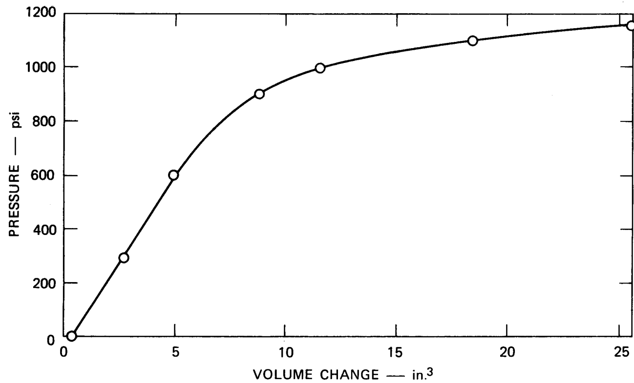
FIGURE A.11 PRESSURE-VOLUME CHANGE RELATION FOR SM 1
