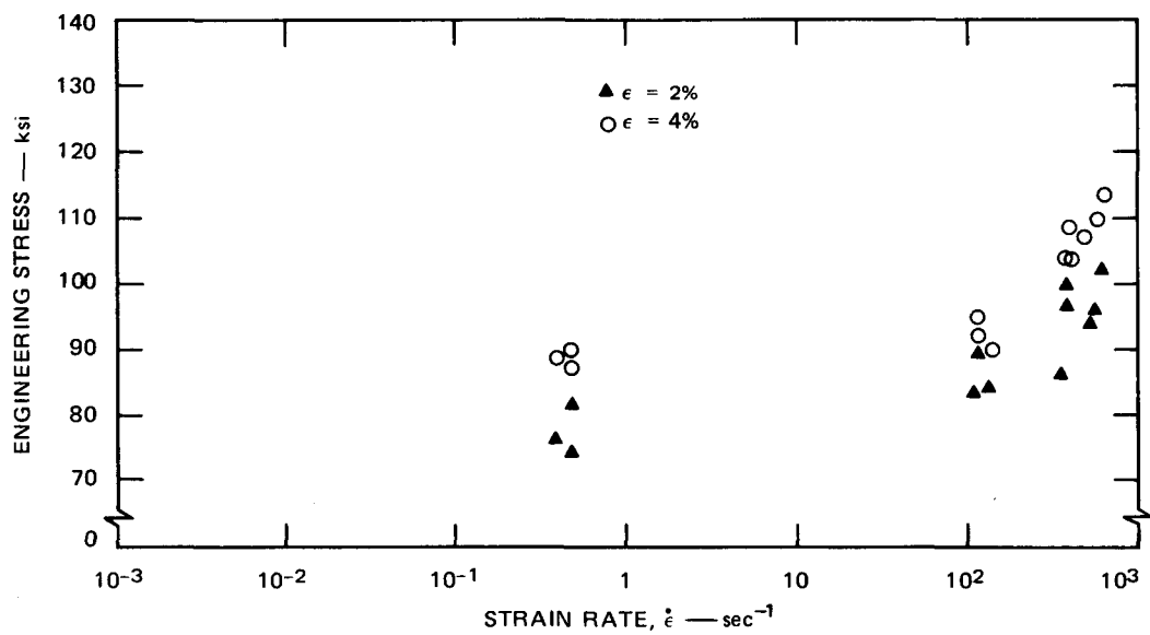
FIGURE B.5 STRAIN RATE EFFECTS IN 533-B CLASS 1 CARBON STEEL
