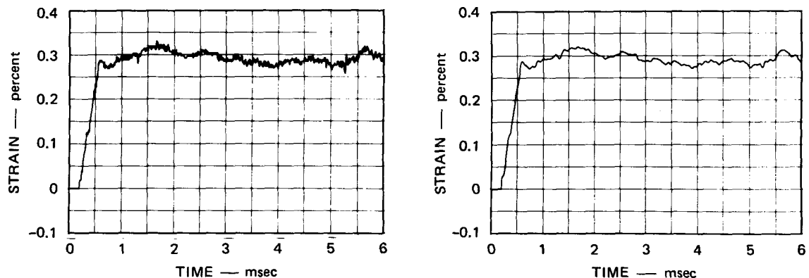
(b) STRAIN RECORDS SM 5 S5 COF = 10 kHz
