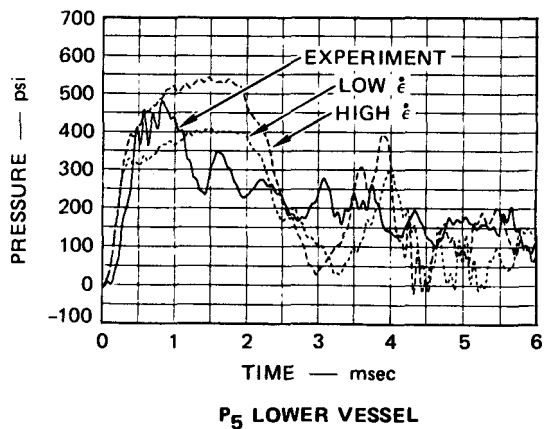
FIGURE 33 COMPARISON OF SM 5 PRESSURE RECORDS WITH GE REXCO RESULTS
