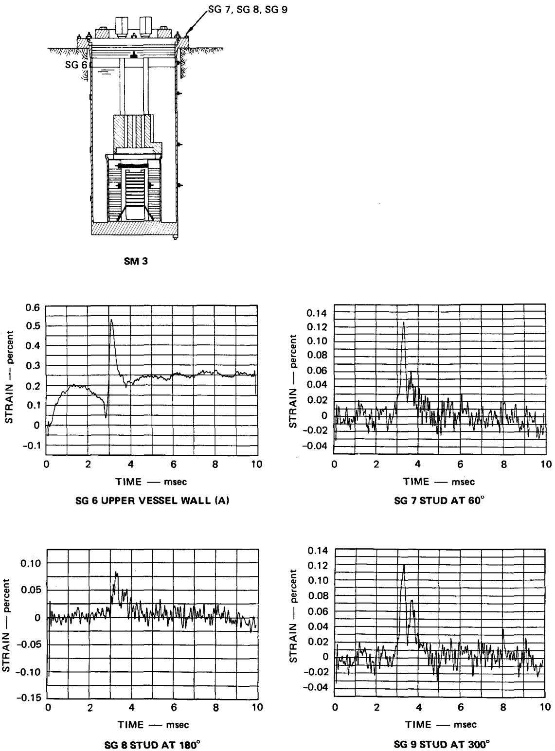
FIGURE D.11 STRAIN RECORDS FOR SM 3 (Concluded)
