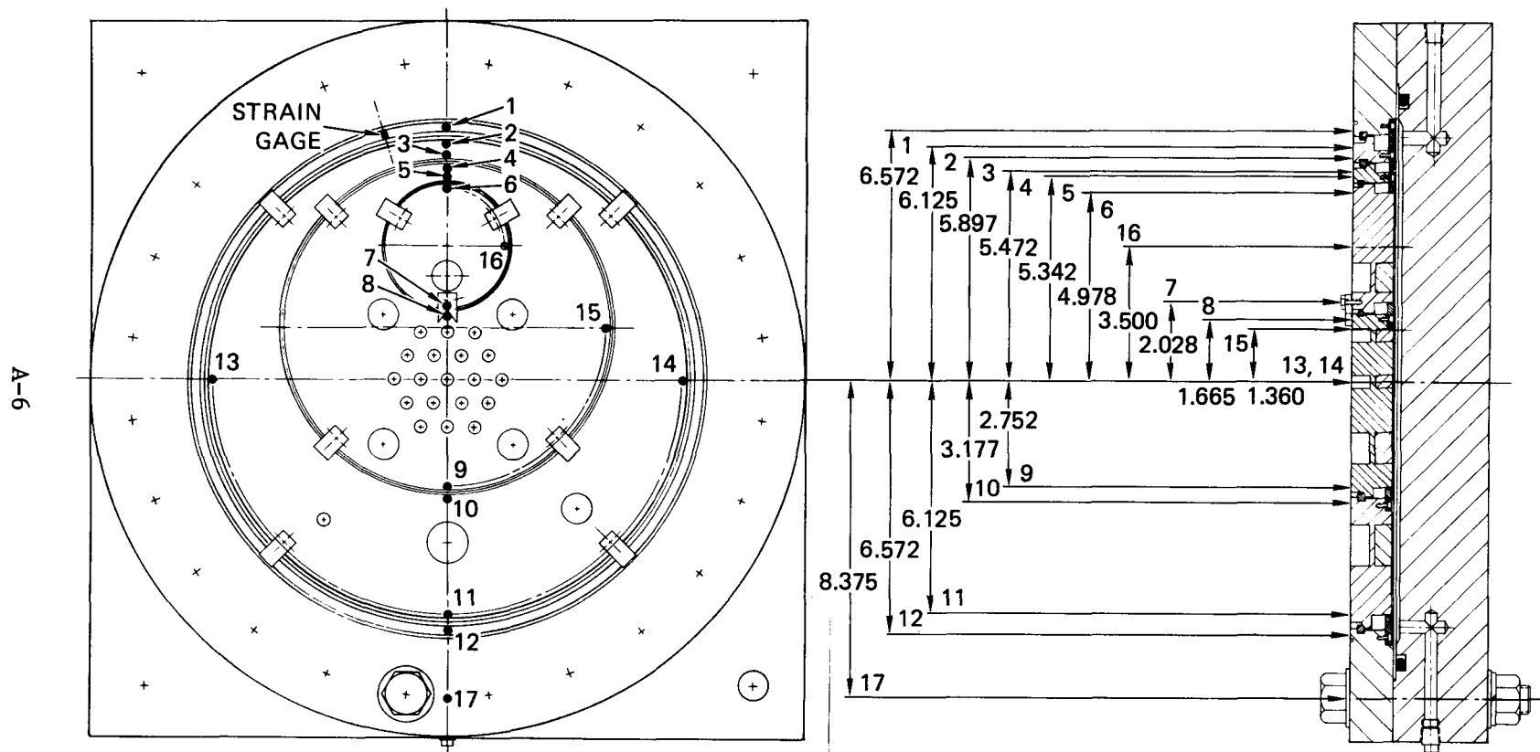
FIGURE A.3 INSTRUMENTATION LAYOUT FOR STATIC TEST SM 1
