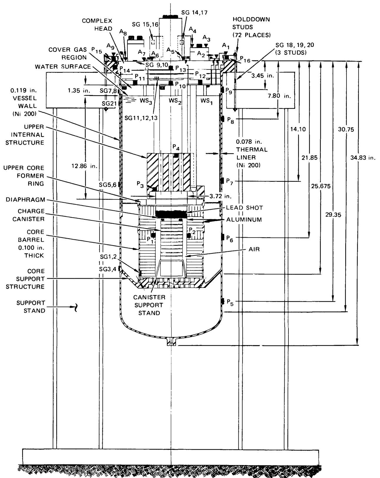
FIGURE 18 SM 5 WITH INSTRUMENTATION
