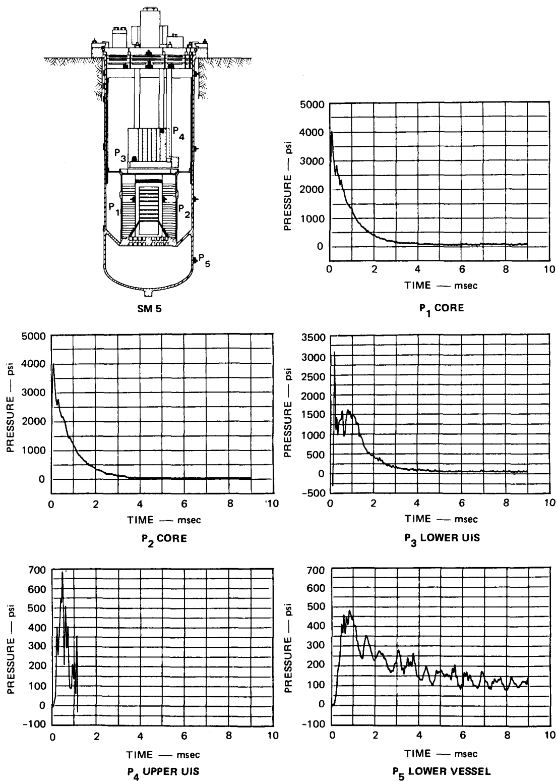
FIGURE D.25 PRESSURE RECORDS FOR SM 5
