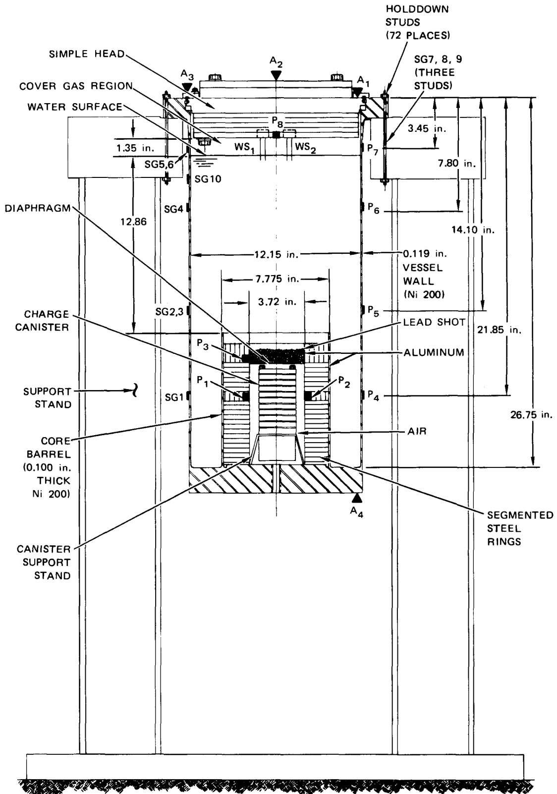
FIGURE D.1 SM 2 WITH INSTRUMENTATION
