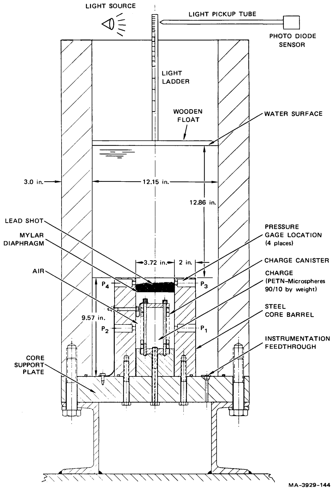
FIGURE C.1 SCHEMATIC OF CALIBRATION TEST APPARATUS
