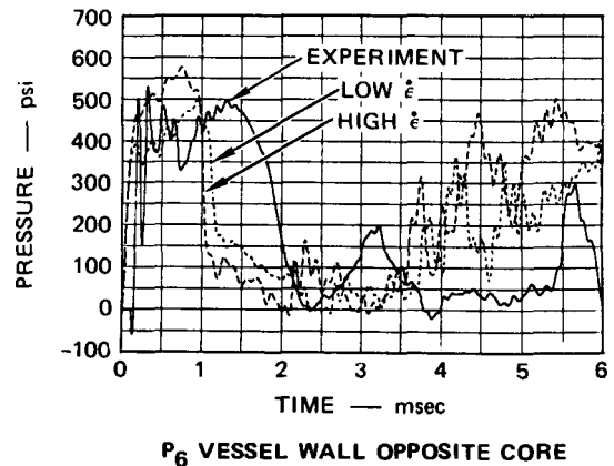
FIGURE 33 COMPARISON OF SM 5 PRESSURE RECORDS WITH GE REXCO RESULTS
