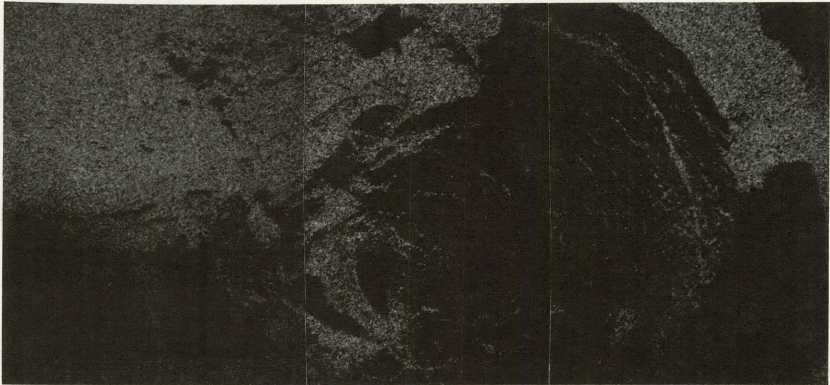
Figure 6. SCANNING ELECTRON MICROSCOPE ALUMINUM X-RAY MAP THAT VERIFIES THOSE AREAS WHICH ARE VOID OF ALUMINUM (THE DARK AREAS). (This Area is the same as that in Figure 5; ~ 70X)
