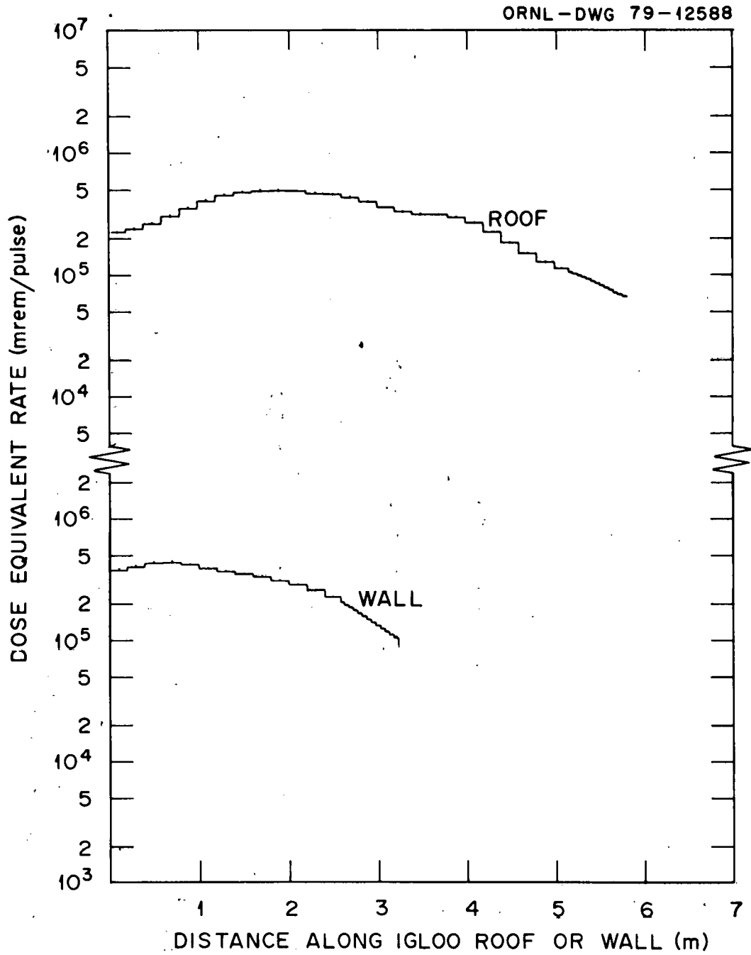
Fig. 7. Dose equivalent rate as a function of distance along the roof and wall of the igloo.
