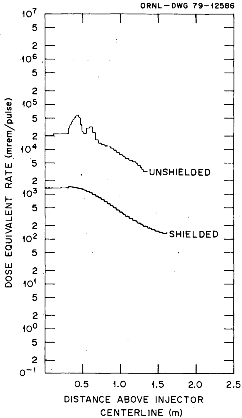
Fig. 9. Dose equivalent rate along the rear of the neutral beam injector as a function of distance above the injector centerline.
