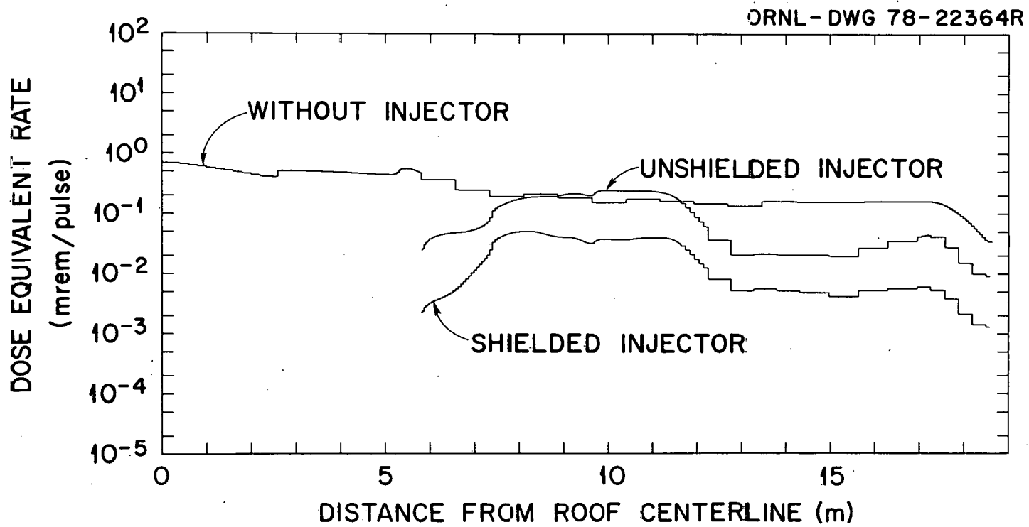
Fig. 5. Dose equivalent rate as a function of distance from the roof centerline.
