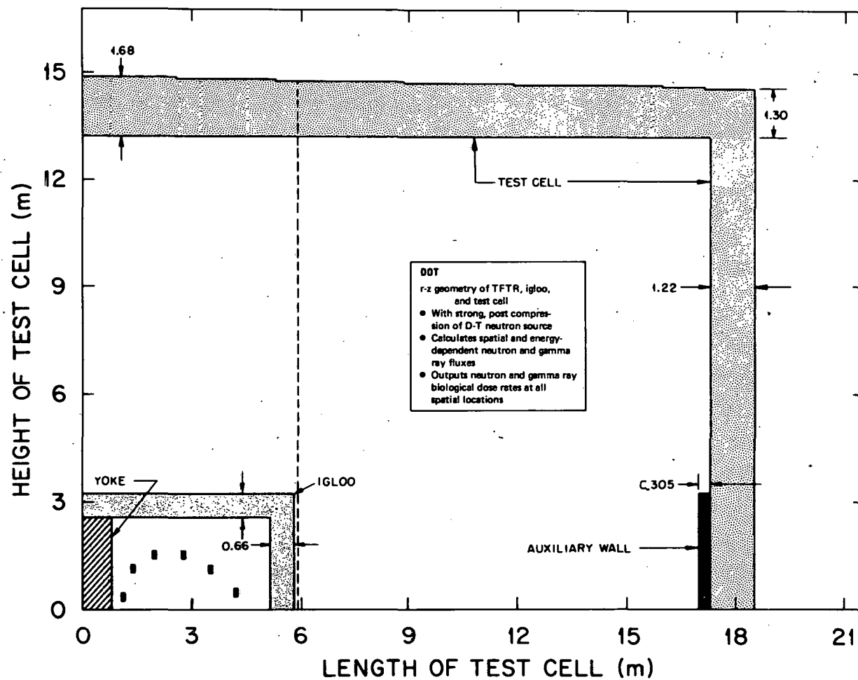
Fig. 1. Two-dimensional calculations model of the test cell and igloo.
