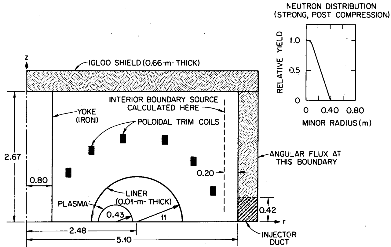
Fig. 4. Two-dimensional calculational model of the TFTR and the igloo used to obtain the energy, spatial, and angular distributions of neutrons and gamma rays incident on the injector.
