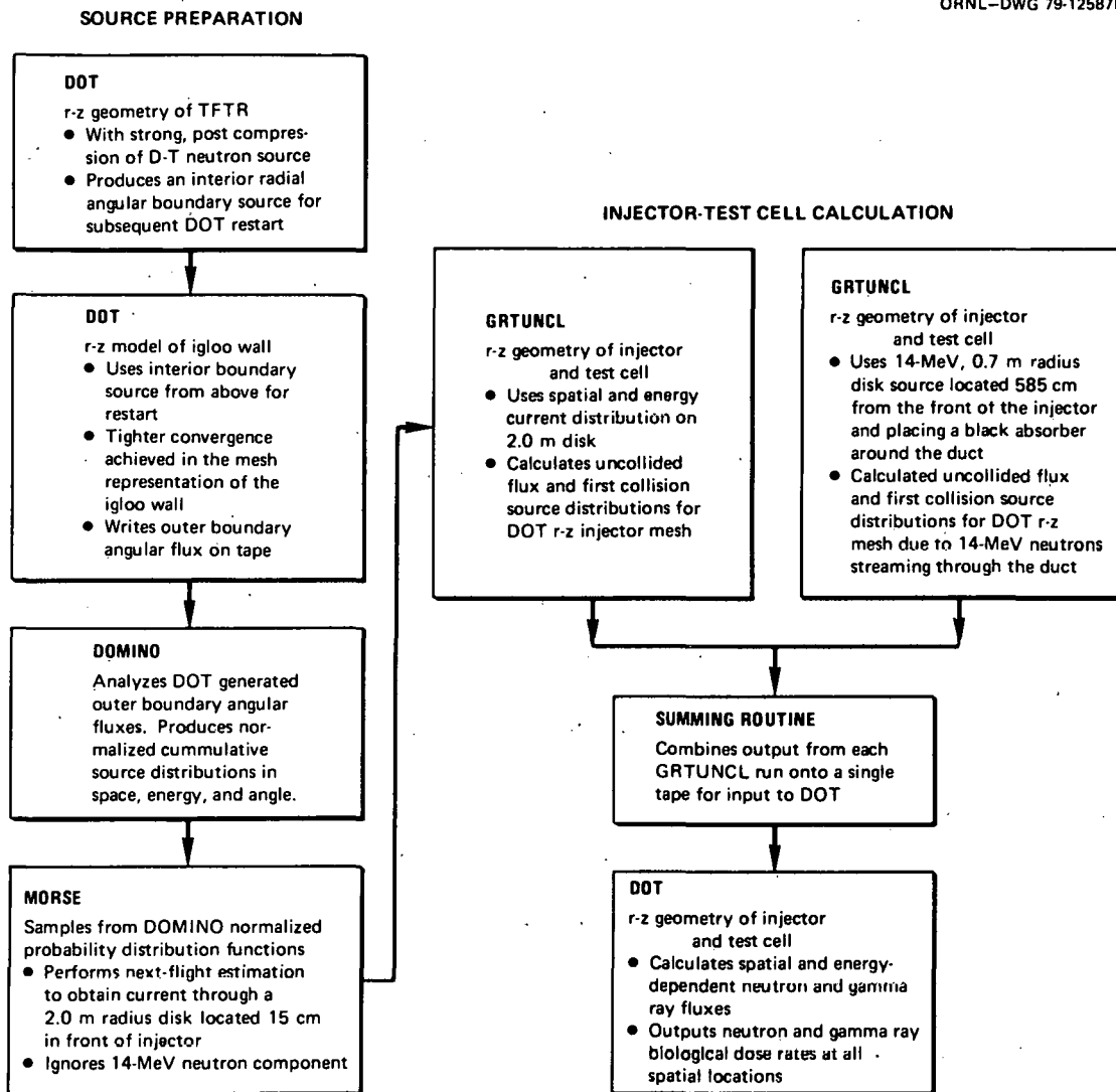
Fig. 3. Calculational sequences used to estimate the contributions to the dose equivalent rate on the test cell roof and walls due to streaming through the neutral beam injector.
