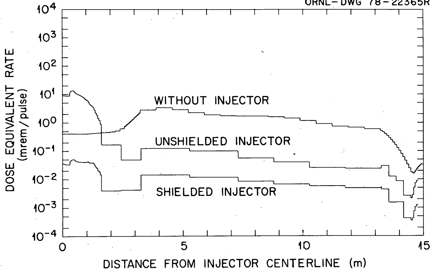
Fig. 6. Dose equivalent rate outside the test cell wall as a function of distance from the injector centerline.
