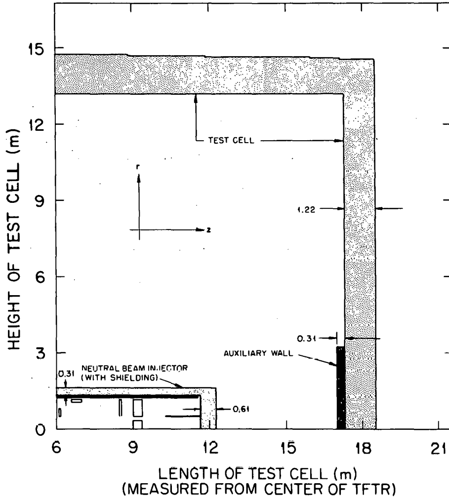
Fig. 2. Two-dimensional calculational model of the test cell and the neutral beam injector.
