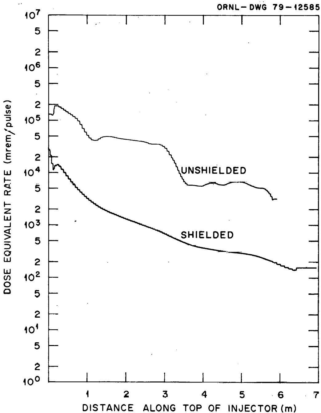
Fig. 8. Dose equivalent rate as a function of distance along the neutral beam injector.
