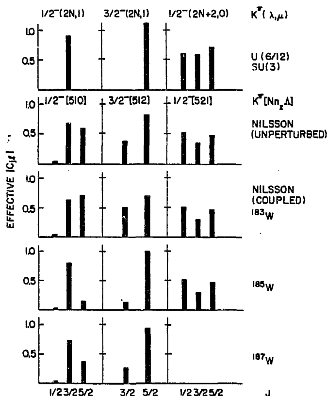
Fig. 6. Values of C_{J, \lambda}^{\text{eff}} in the U(6/12) and Nilsson schemes. Those for the latter are calculated using the wave functions and Coriolis mixing amplitudes of ref. 17.
