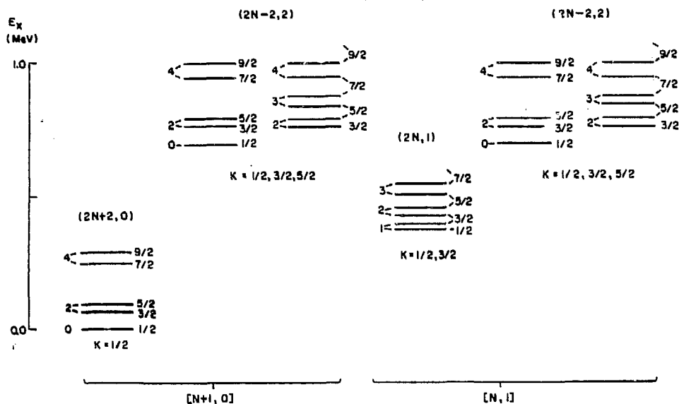
Fig. 5. The SU(3) scheme of U(6/12). Representations are labelled by the (\lambda, \mu) quantum number of SU_{BF}^3(3) and by the [N_1 N_2] labels of U_{BF}^6(6) .
