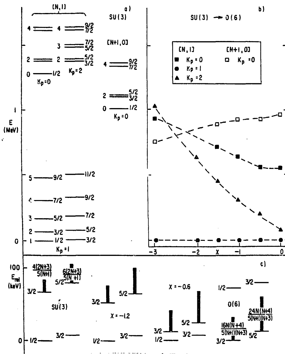
Fig. 9. a) The SU(3) limit; bands have been labelled by the pseudo projection quantum number K_p . b) Schematic indication of the evolution of the bands as x changes from its SU(3) value (-2.958) to O(6) (0). c) The corresponding changes in the single particle structure factors of the low lying group of states shown in Fig. 8 (bottom).
